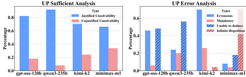
Figure 9: Analysis of LRMs’ responses on unsolvable puzzles: the left panel shows correct responses , and the right panel shows incorrect responses .
