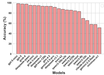
Figure 8: Overall model performance on unsolvable puzzles.
