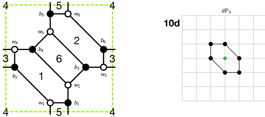
Figure 29: The brane tiling and toric diagram of Model 10d.
