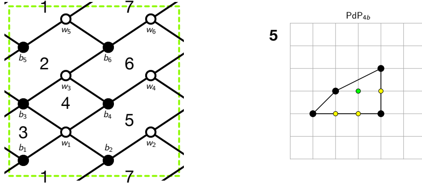
Figure 16: The brane tiling and toric diagram of Model 5.
