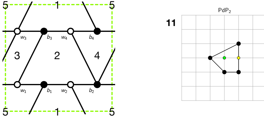
Figure 30: The brane tiling and toric diagram of Model 11.
