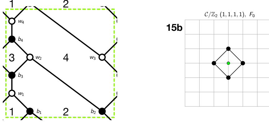
Figure 36: The brane tiling and toric diagram of Model 15b.
