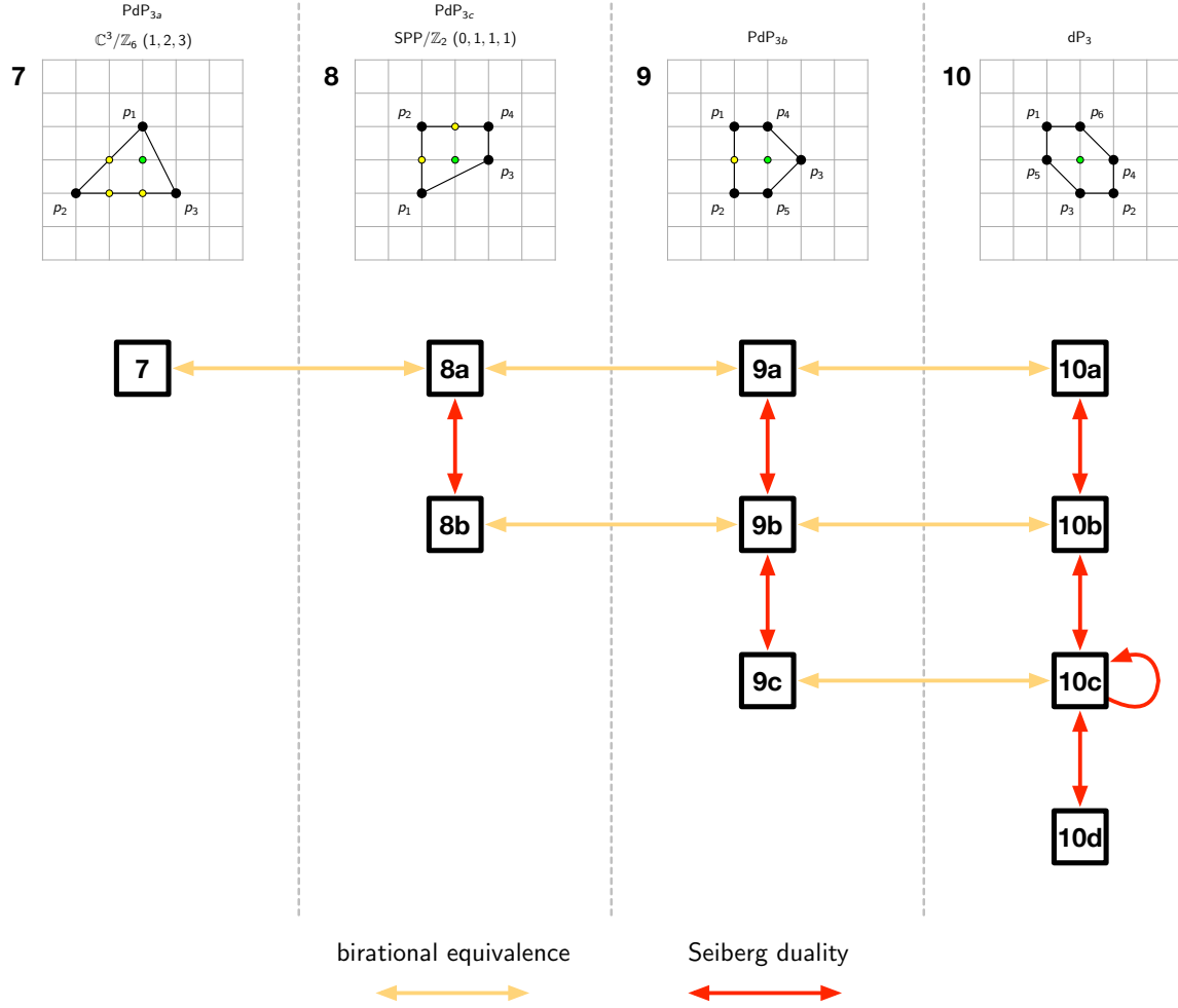
Figure 40: Brane tilings and toric diagrams in Bucket 3.
