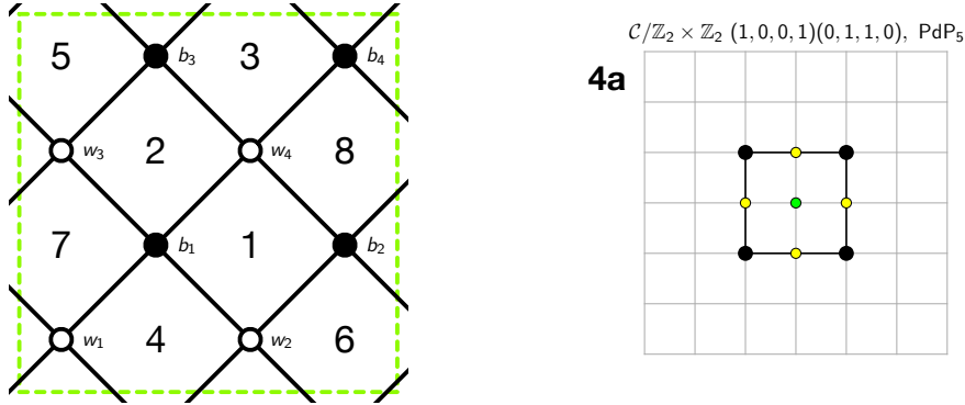
Figure 12: The brane tiling and toric diagram of Model 4a.
