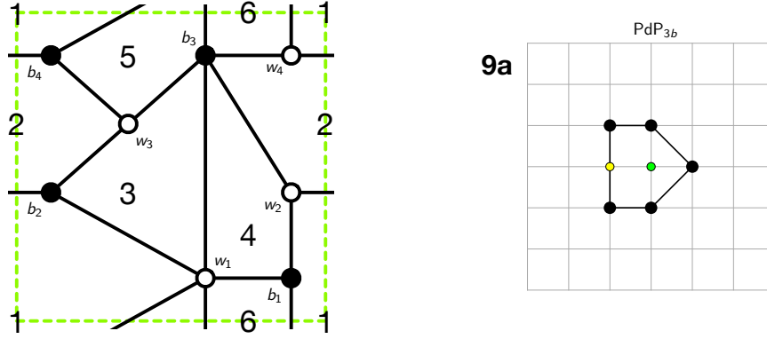
Figure 23: The brane tiling and toric diagram of Model 9a.
