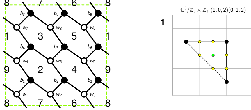
Figure 8: The brane tiling and toric diagram of Model 1.
