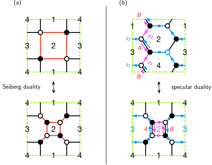
Figure 3: (a) Seiberg duality on brane tilings [27, 28, 30, 34, 35] is a local deformation of the bipartite graph on the 2-torus acting on square faces, which is also known as urban renewal or spider moves [4, 43, 44]. (b) Specular duality on brane tilings [68] swaps directed paths along edges corresponding to zig-zag paths with directed paths around faces and vice versa while preserving intersections between these paths.
