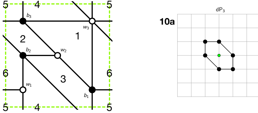
Figure 26: The brane tiling and toric diagram of Model 10a.
