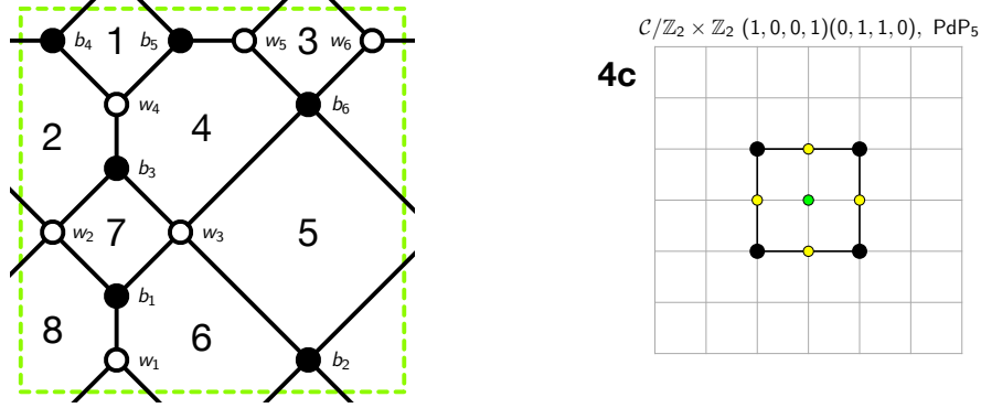
Figure 14: The brane tiling and toric diagram of Model 4c.
