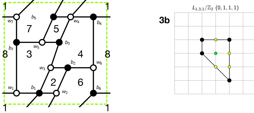
Figure 11: The brane tiling and toric diagram of Model 3b.
