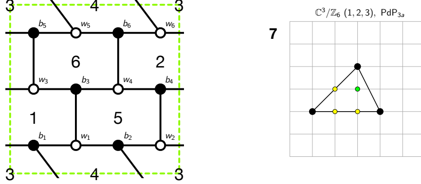
Figure 20: The brane tiling and toric diagram of Model 7.
