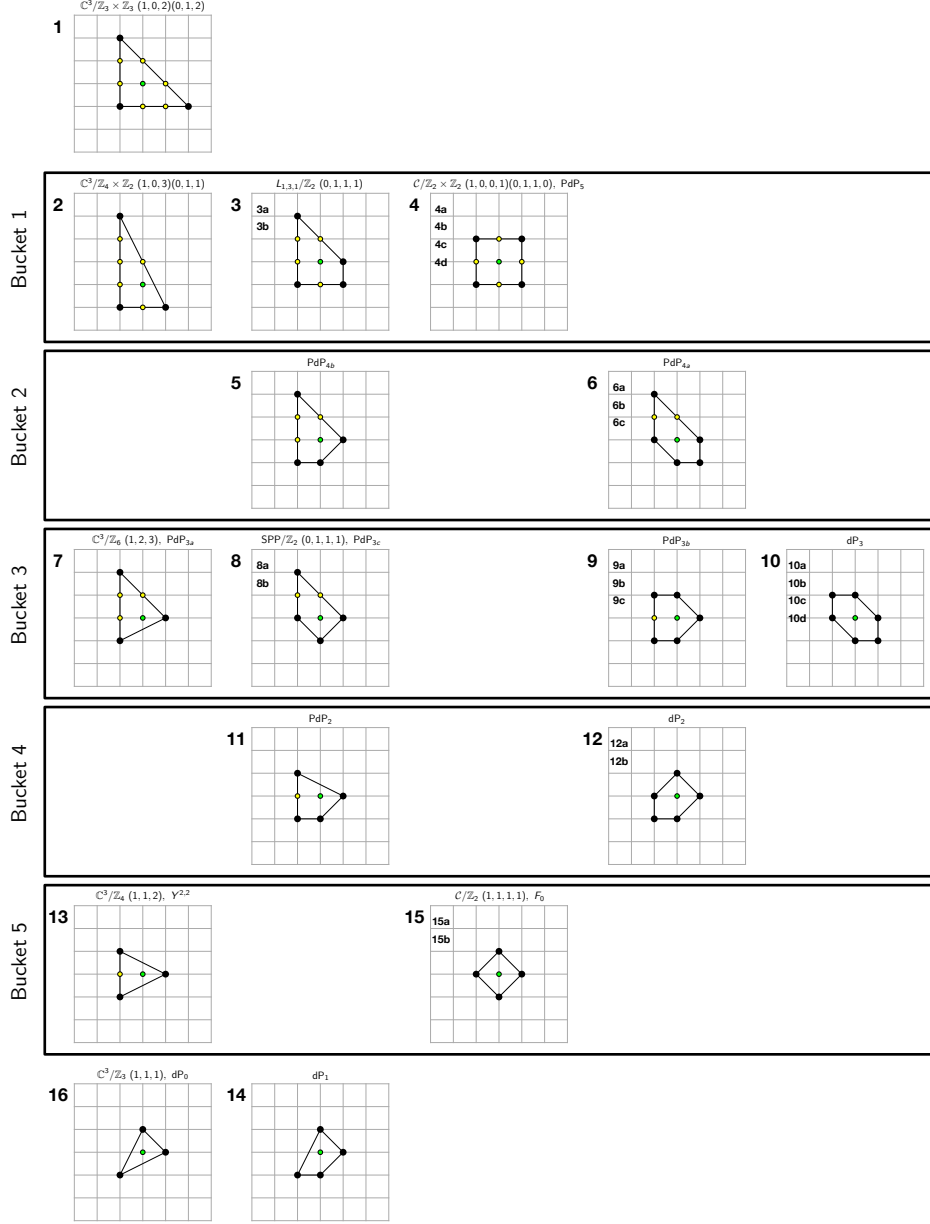
Figure 1: The 16 reflexive polygons in 2 dimensions with labels corresponding to the associated 30 brane tilings classified in [15]. Birational transformations between toric Calabi-Yau 3-folds correspond to birational equivalence between the associated dimer integrable systems. Combined with Seiberg duality, we identify 5 equivalence classes called buckets amongst the 30 brane tilings and dimer integrable systems classified in this work.
