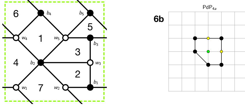
Figure 18: The brane tiling and toric diagram of Model 6b.
