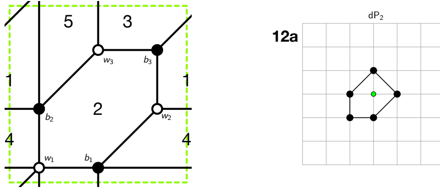
Figure 31: The brane tiling and toric diagram of Model 12a.
