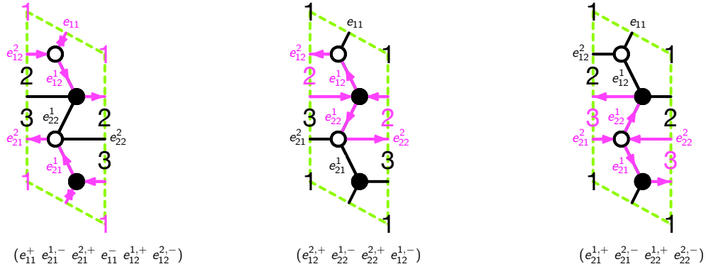
Figure 6: The brane tiling for the suspended pinch point (SPP) with zig-zag paths given by \Sigma_e \cdot (\sigma_W^{-1})^+ \cdot (\sigma_B)^- and face paths given by \Sigma_e \cdot (\sigma_W^{-1})^+ \cdot (\sigma_B^{-1})^- .
