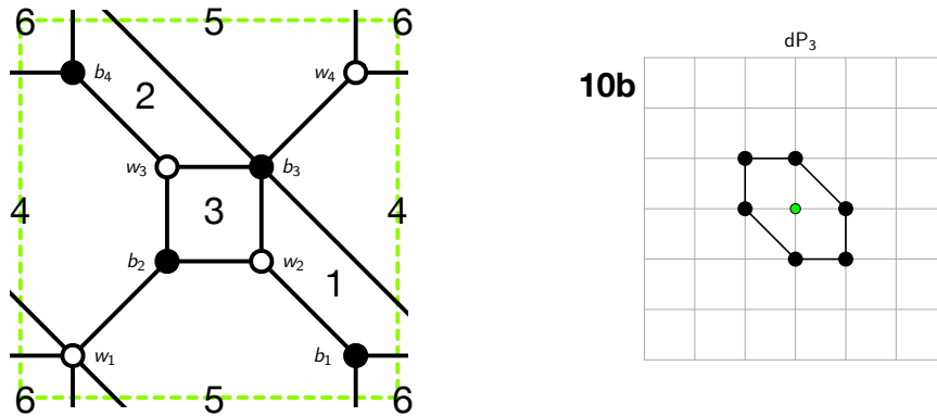
Figure 27: The brane tiling and toric diagram of Model 10b.
