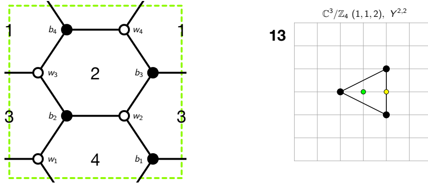
Figure 33: The brane tiling and toric diagram of Model 13.
