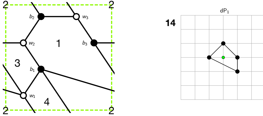
Figure 34: The brane tiling and toric diagram of Model 14.
