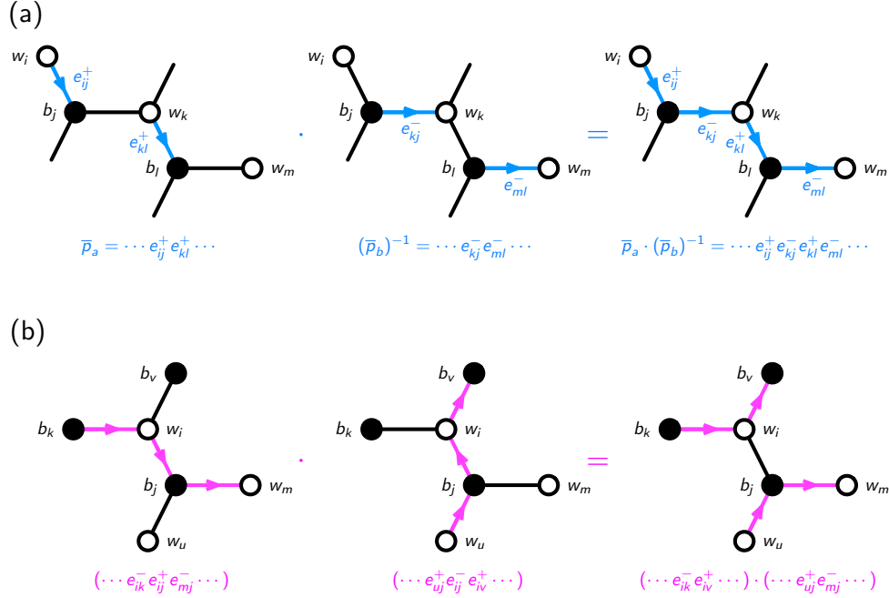
Figure 4: (a) A product of perfect matchings weights \bar{p}_a and (\bar{p}_b)^{-1} in terms of directed edge variables, and (b) a product of closed directed paths given by permutations in S_{2|E|} with a cancellation between a pair of directed edges.
