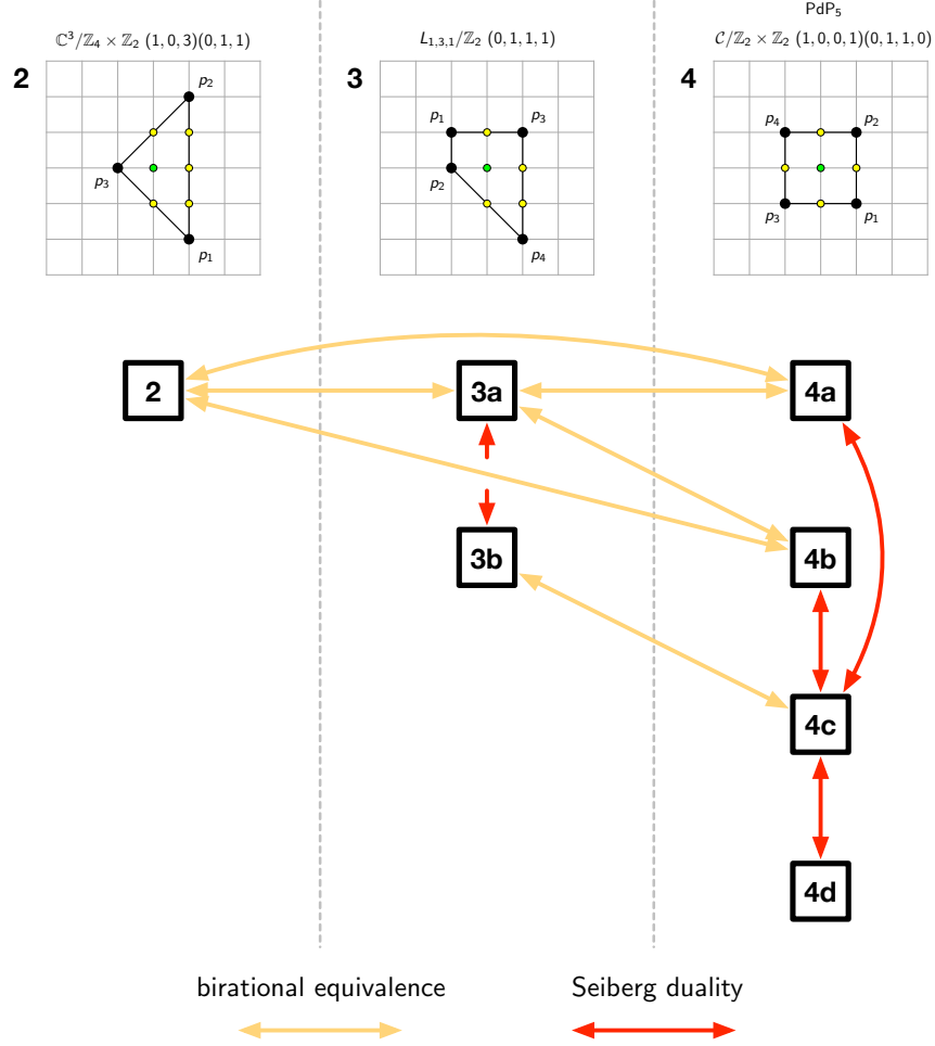
Figure 38: Brane tilings and toric diagrams in Bucket 1.
