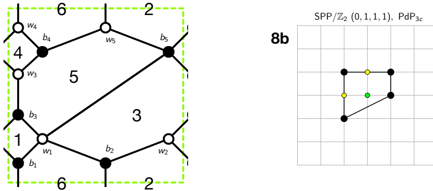
Figure 22: The brane tiling and toric diagram of Model 8b.
