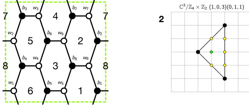
Figure 9: The brane tiling and toric diagram of Model 2.
