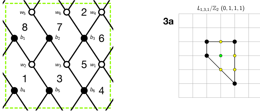
Figure 10: The brane tiling and toric diagram of Model 3a.
