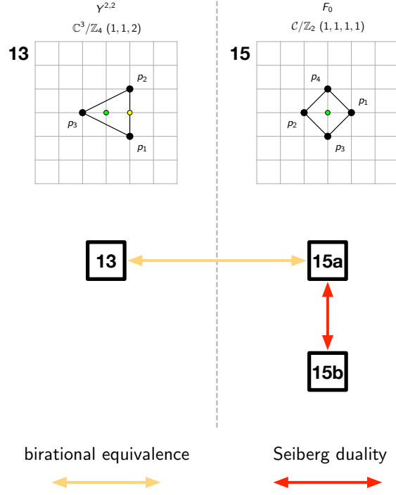
Figure 42: Brane tilings and toric diagrams in Bucket 5.
