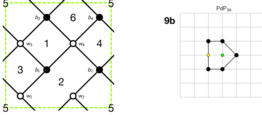
Figure 24: The brane tiling and toric diagram of Model 9b.
