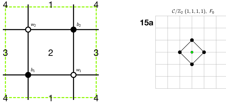
Figure 35: The brane tiling and toric diagram of Model 15a.
