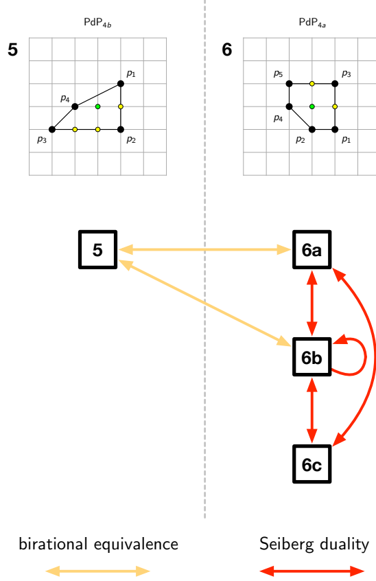
Figure 39: Brane tilings and toric diagrams in Bucket 2.
