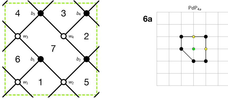
Figure 17: The brane tiling and toric diagram of Model 6a.
