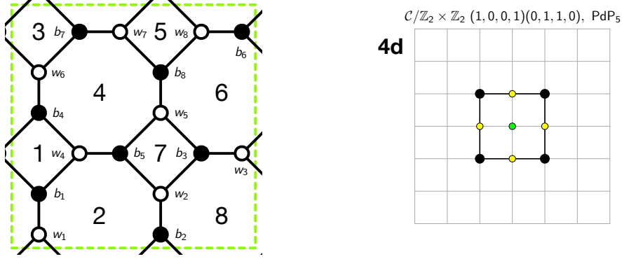
Figure 15: The brane tiling and toric diagram of Model 4d.
