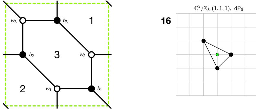
Figure 37: The brane tiling and toric diagram of Model 16.
