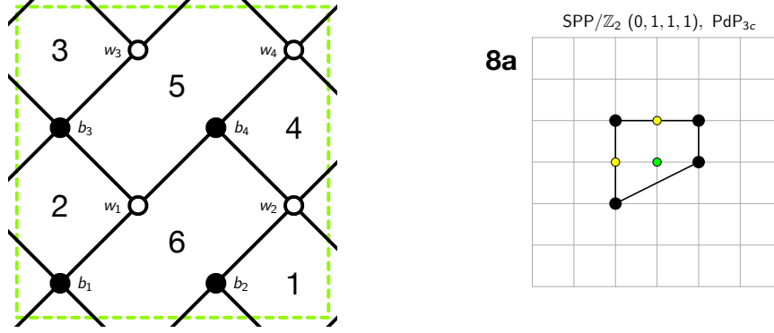
Figure 21: The brane tiling and toric diagram of Model 8a.
