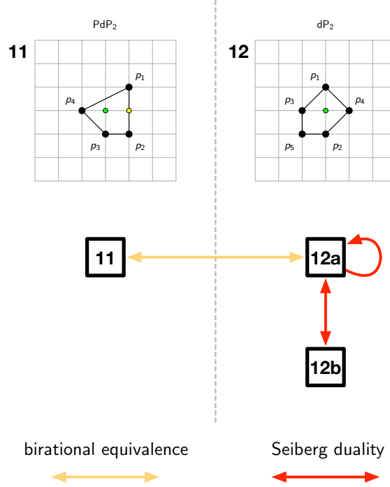
Figure 41: Brane tilings and toric diagrams in Bucket 4.
