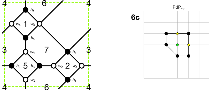
Figure 19: The brane tiling and toric diagram of Model 6c.
