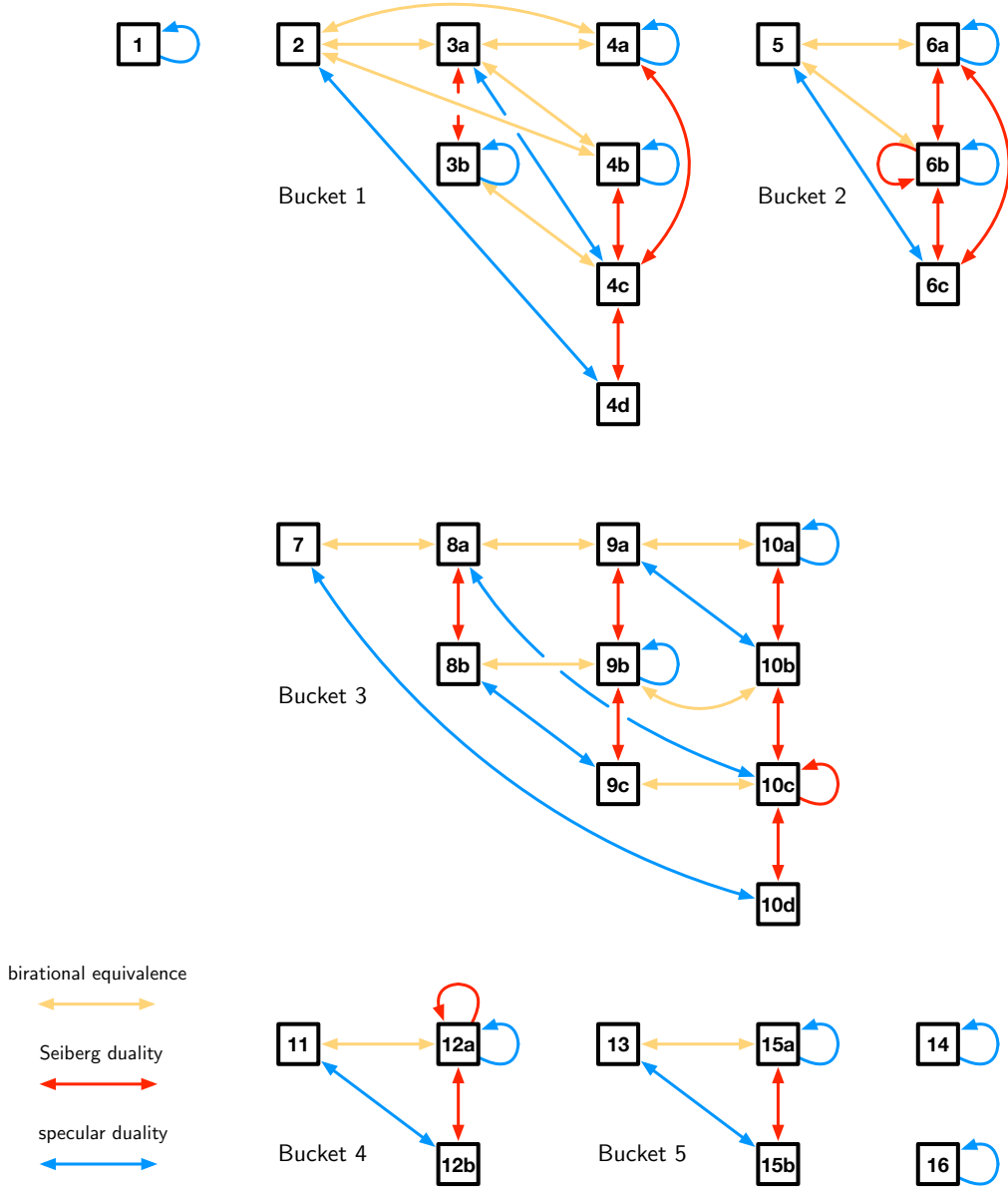
Figure 2: The 30 brane tilings corresponding to the 16 reflexive polygons in dimension 2 are related by Seiberg duality (red), specular duality (blue), and birational transformations (yellow). Under Seiberg duality and under birational transformations, the associated dimer integrable systems are equivalent and form equivalence classes, which we call buckets. The labels correspond to the 30 brane tilings classified in [15] with the corresponding 16 reflexive toric diagrams given in Figure 1.
