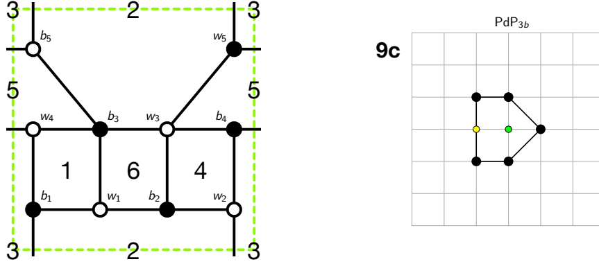
Figure 25: The brane tiling and toric diagram of Model 9c.
