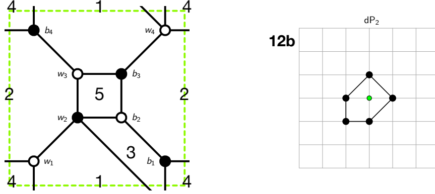
Figure 32: The brane tiling and toric diagram of Model 12b.
