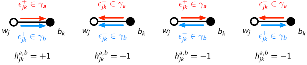
Figure 7: The possible directed intersections between directed paths \gamma_a and \gamma_b at edge e_{jk} with the corresponding directed intersection number h_{jk}^{a,b} .
