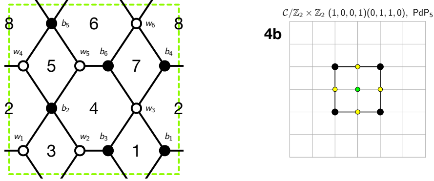
Figure 13: The brane tiling and toric diagram of Model 4b.
