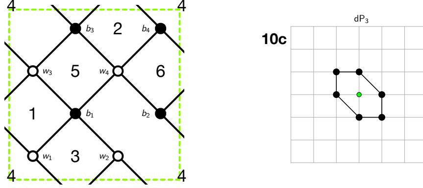
Figure 28: The brane tiling and toric diagram of Model 10c.
