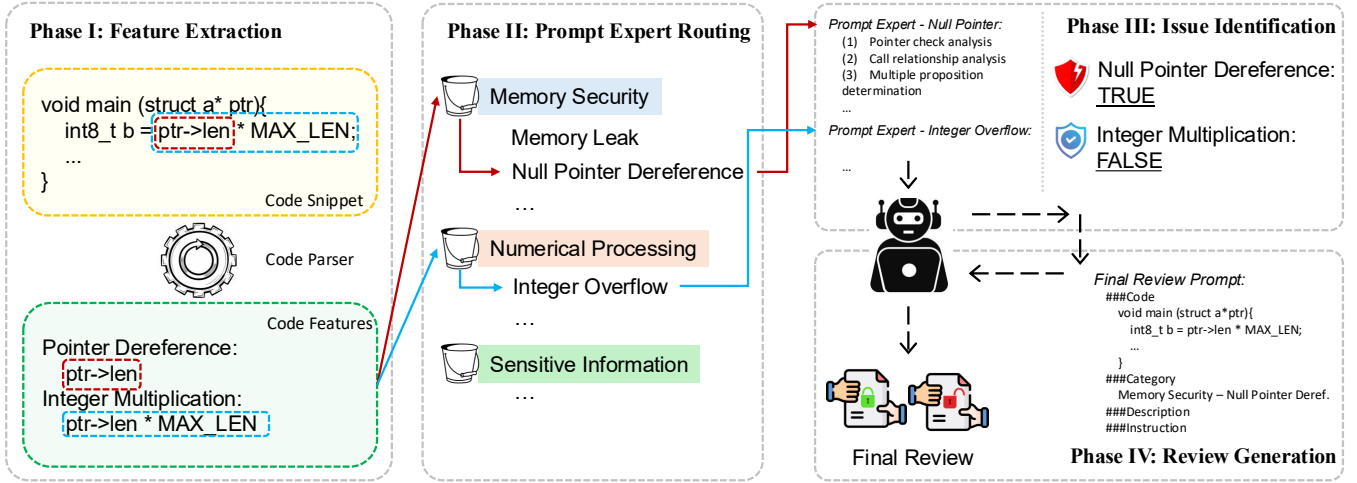
Fig. 1. The overview of iCodeReviewer.
