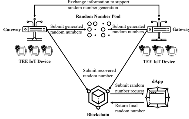
Figure 1 Overview of HRNG. Each gateway connects with multiple IoT devices equipped with TEE to provide random sources to the system, and the final random number is generated in a verifiable manner on the blockchain. Although the dApp is demonstrated as a different entity, it is actually deployed on the same blockchain and maintained by the same set of blockchain nodes.
