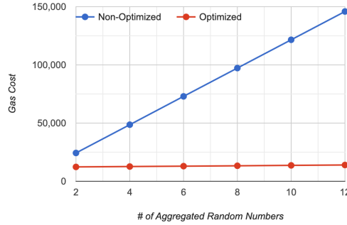
Figure 2 The gas costs for non-optimized and improved HRNG. Here both versions use the elliptic curve-based Pedersen commitment scheme but the unoptimized HRNG does not utilize the homomorphic feature. The x -axis is the number of values to be aggregated and the y -axis is the amount of gas required to finish the work (commitment openings and aggregation).
