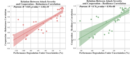
Figure 4: The extent cooperation is correlated to robustness and resilience linearly depends on the severity of the attack.
