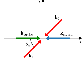
FIG. 12. Schematic diagram of a three pulse collision scenario.
