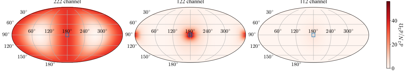
FIG. 14. Angular signal photon spectrum for particular channels from the collision of a Gaussian probe with a dipole pulse. Setup parameters are similar to Fig. 2 (b). Blue square shows 10^\circ \times 10^\circ detector region. (Left) 222 channel cubic in the dipole field corresponds to dipole self-emission and yields N_{\text{tot}} \approx 289 , N_{\text{det}} \approx 1.15 . (Middle) 122 channel linear in the probe field corresponds to the back-reflected signature we look for and yields N_{\text{tot}} \approx 38 , N_{\text{det}} \approx 1.62 . (Right) 112 channel linear in the dipole field yields N_{\text{tot}} \approx 4.4 , N_{\text{det}} \approx 0.13 .
