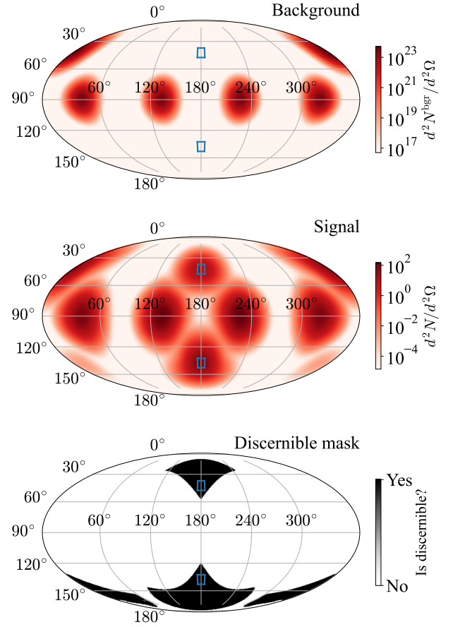
FIG. 7. Angular background and signal photon spectrum and discernible mask from the collision of a Gaussian probe with a belt configuration. Probe parameters: W = 20 J, \lambda = 800 nm, w_0 = 2\lambda , \tau_{\text{FWHM}} = 20 fs, (\vartheta_{\text{probe}}, \varphi_{\text{probe}}) = (45^\circ, 0^\circ) , \beta_{\text{probe}} = 0^\circ . The belt consists of 4 pulses ( i = 1..4 ) with W = 10 J each, (\vartheta_{b,i}, \varphi_{b,i}) = (90^\circ, 90^\circ \times i - 45^\circ) and polarization angles \beta_1 = \beta_4 = 0^\circ, \beta_2 = \beta_3 = 90^\circ (other parameters are similar to the probe). Blue squares show 10^\circ \times 10^\circ detector regions. Signal around (\vartheta, \varphi) = (135^\circ, 180^\circ) is back-reflected with N_{\text{det}} \approx 1.2 , signal around (\vartheta, \varphi) = (45^\circ, 180^\circ) is forward-angle-reflected with N_{\text{det}} \approx 0.26 .
