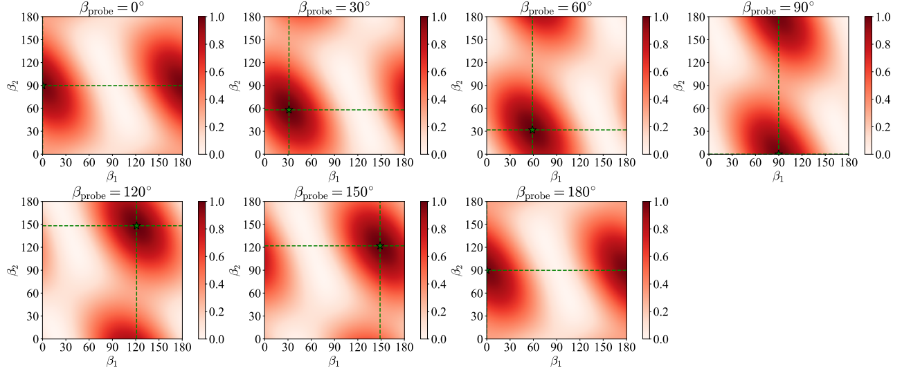
FIG. 15. Polarization prefactor (from Eq. B3) dependence on the polarization of individual beams (\beta_1, \beta_2, \beta_{\text{probe}}) for a fixed collision angle \theta_c = 45^\circ . The maximal prefactor value was normalized to 1, with a normalizing factor of \approx 38072 .
