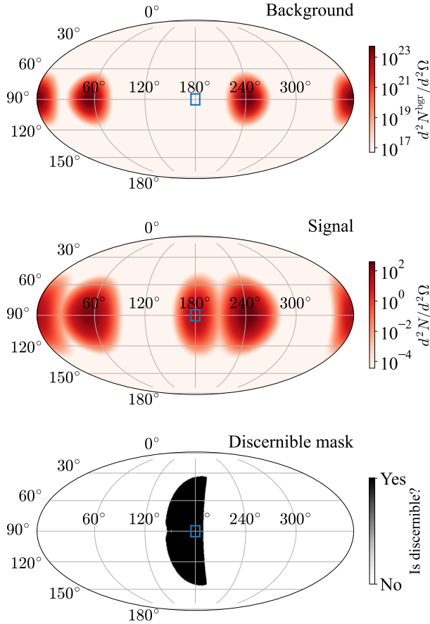
FIG. 13. Angular background and signal photon spectrum and discernible mask from the collision of three Gaussian pulses. All pulses are characterized by W = 20 J, \vartheta = 90^\circ , \lambda = 800 nm, \tau_{\text{FWHM}} = 20 fs, w_0 = 2\lambda and (\varphi_{\text{probe}}, \varphi_1, \varphi_2) = (0^\circ, 60^\circ, 240^\circ) , (\beta_{\text{probe}}, \beta_1, \beta_2) = (0^\circ, 0^\circ, 90^\circ) . Blue square shows 10^\circ \times 10^\circ detector region with N_{\text{det}} \approx 1.5 .
