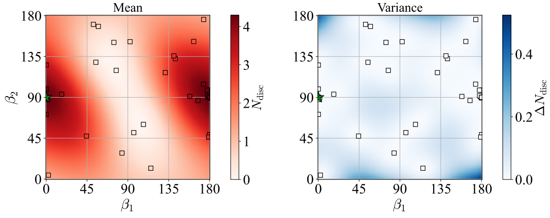
FIG. 17. Optimization results in 2-dimensional parameter space: the linear polarization angle of pump beams ( \beta_1, \beta_2 ). Colormaps correspond to (left) the mean and (right) the variance of the fitted Gaussian Process surrogate model. The optimization objective was to maximize the total number of discernible photons. The polarization of the probe is fixed \beta_{\text{probe}} = 0^\circ and the collision angle \theta_c = 55^\circ . Other parameters are similar to Fig. 13. Found optimum is (\beta_1^*, \beta_2^*) \approx (0^\circ, 90^\circ) achieving N_{\text{disc}} \approx 4.3 . Compare the mean plot to the \beta_{\text{probe}} = 0^\circ plots in Figs. 15 and 16.
