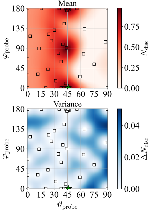
FIG. 9. Optimization results in 2-dimensional parameter space: the propagation direction of the probe ( \vartheta_{\text{probe}}, \varphi_{\text{probe}} ). Colormaps correspond to (top) the mean and (bottom) variance of the fitted Gaussian Process surrogate model. The optimization objective was to maximize the total discernible signal. The probe collides with a belt configuration consisting of four focused Gaussian pulses with polarizations \beta_1 = \beta_2 = \beta_3 = \beta_4 = 0^\circ . Other parameters are similar to Fig. 7. Found optimum is (\vartheta_{\text{probe}}^*, \varphi_{\text{probe}}^*) \approx (45.9^\circ, 0^\circ) achieving N_{\text{disc}} \approx 0.97 . The top plot shows us that there are three equivalent configurations with \vartheta_{\text{probe}} \approx 45.9^\circ : 1) \varphi_{\text{probe}} = 0^\circ \leftrightarrow probe propagates between pair of pulses described by (\mathbf{k}_4, \mathbf{k}_1) , 2) \varphi_{\text{probe}} = 90^\circ \leftrightarrow between (\mathbf{k}_1, \mathbf{k}_2) , 3) \varphi_{\text{probe}} = 180^\circ \leftrightarrow between (\mathbf{k}_2, \mathbf{k}_3) . These configurations result in the same total discernible signal, and optimization converged to one of them. When \vartheta_{\text{probe}} is too large, no sizable discernible signal could be detected. The bottom plot shows that around the observation points the variance is zero (as expected), while in unexplored parameter regions it still remains small.
