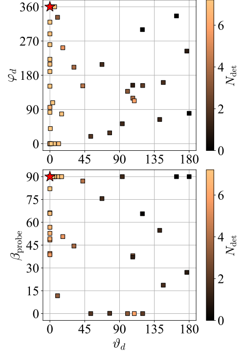
FIG. 5. Optimization results in 3-dimensional parameter space: b -dipole moment orientation ( \vartheta_d, \varphi_d ) and probe polarization ( \beta_{\text{probe}} ). The optimization objective was to maximize the signal in a 10^\circ \times 10^\circ detector around (\vartheta, \varphi) = (90^\circ, 180^\circ) . Probe and dipole pulse parameters are similar to Fig. 2. Found optimum is (\vartheta_d^*, \varphi_d^*, \beta_{\text{probe}}^*) \approx (0^\circ, 360^\circ, 90^\circ) achieving N_{\text{det}} \approx 7.2 . The optimum corresponds to \mathbf{d} \parallel \mathbf{e}_z and \mathbf{E}_{\text{probe}} \parallel \mathbf{e}_y .
