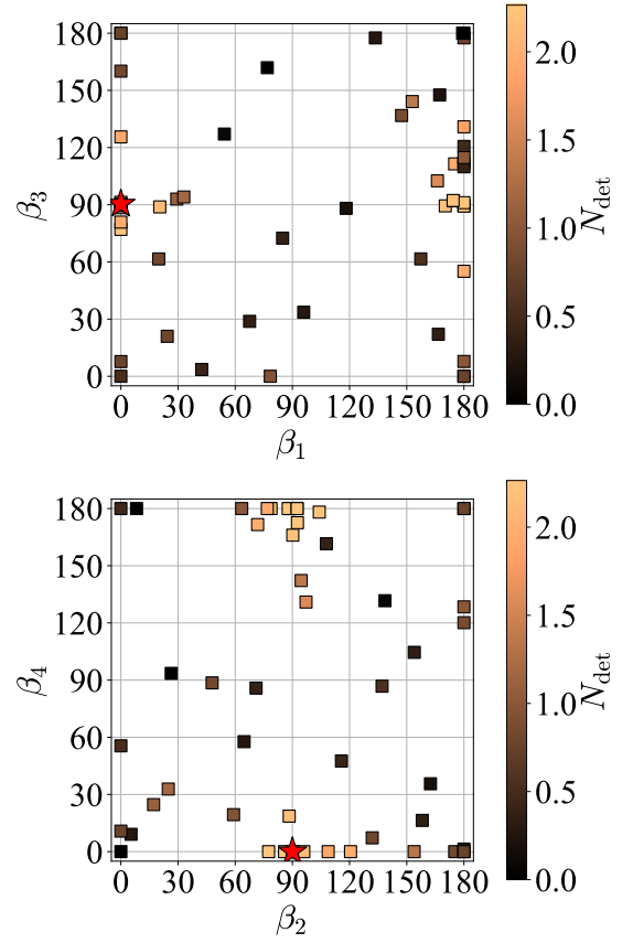
FIG. 10. Optimization results in 4-dimensional parameter space: the linear polarization angle of the different belt pulses ( \beta_1, \beta_2, \beta_3, \beta_4 ). The optimization objective was to maximize the number of photons in a 10^\circ \times 10^\circ detector around (\vartheta, \varphi) = (90^\circ, 180^\circ) . The probe collides with a belt configuration consisting of 4 focused Gaussian pulses at an angle of \vartheta_{\text{probe}} = 90^\circ , the polarization of the probe is fixed to \beta_{\text{probe}} = 0^\circ . Other parameters are similar to Fig. 7. Found optimum is (\beta_1^*, \beta_2^*, \beta_3^*, \beta_4^*) \approx (0^\circ, 90^\circ, 90^\circ, 0^\circ) achieving N_{\text{det}} \approx 2.3 .
