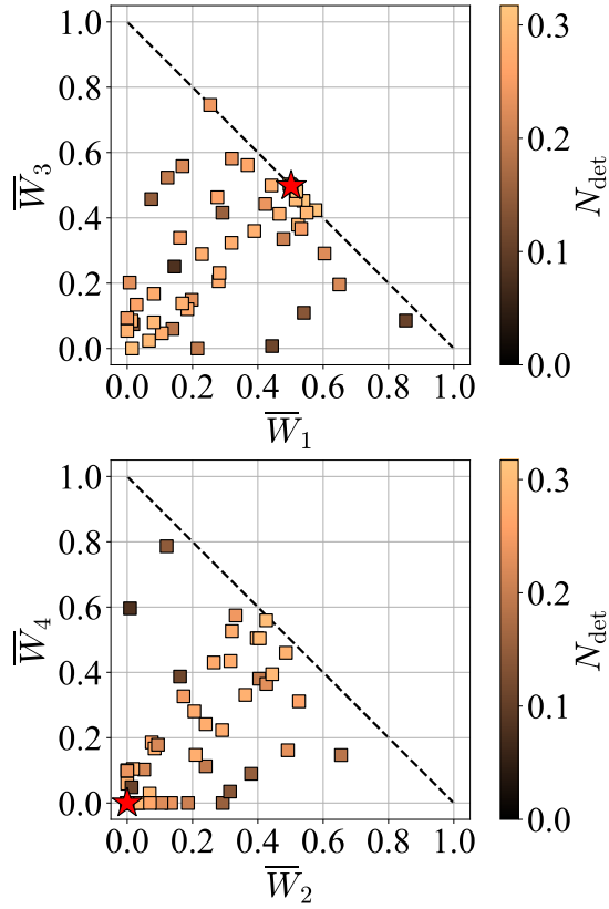
FIG. 11. Optimization results in 3-dimensional parameter space: energy fraction of three pulses in the belt configuration ( \bar{W}_1, \bar{W}_2, \bar{W}_3 ). The energy fraction of the fourth pulse is \bar{W}_4 = 1 - \bar{W}_1 - \bar{W}_2 - \bar{W}_3 . The total energy budget for the belt pulses was fixed to W_{\text{pump}} = 40 J. The optimization objective was to maximize the signal in a 10^\circ \times 10^\circ detector around (\vartheta, \varphi) = (135^\circ, 180^\circ) . The polarization of pulses is \beta_1 = \beta_2 = \beta_3 = \beta_4 = 0^\circ , other parameters are similar to Fig. 7. Found optimum is (\bar{W}_1^*, \bar{W}_2^*, \bar{W}_3^*, \bar{W}_4^*) \approx (0.5, 0, 0.5, 0) achieving N_{\text{det}} \approx 0.32 .
