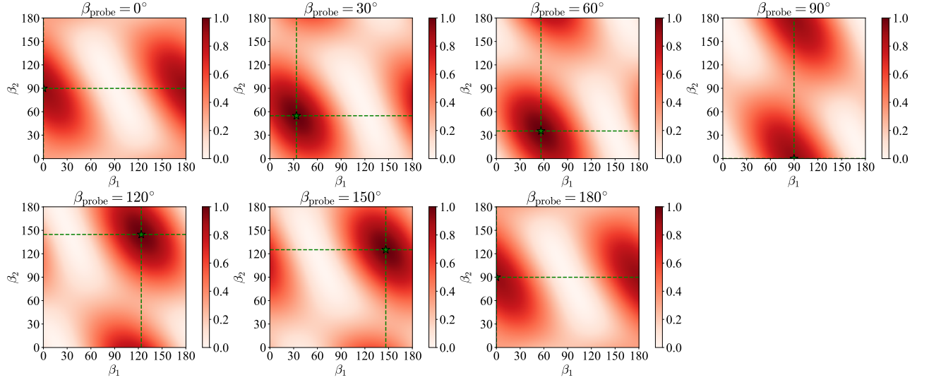
FIG. 16. Polarization prefactor (from Eq. B3) dependence on the polarization of individual beams (\beta_1, \beta_2, \beta_{\text{probe}}) for a fixed collision angle \theta_c = 60^\circ . The maximal prefactor value was normalized to 1, with a normalizing factor of \approx 32329 .
