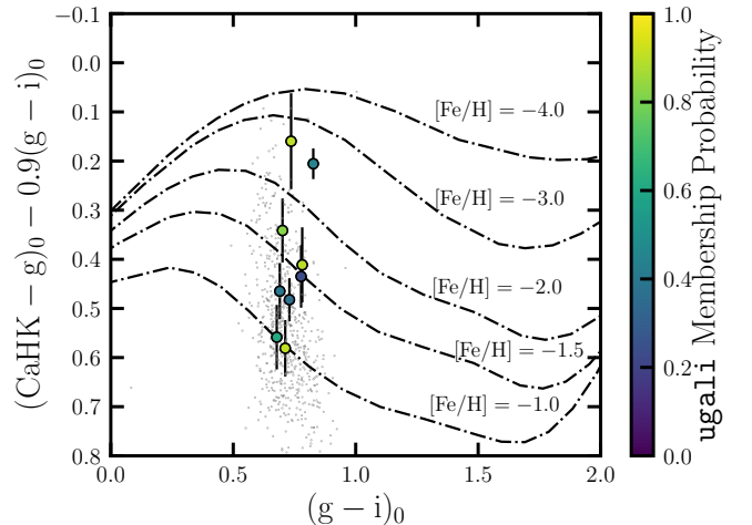
Figure 5. Color-color diagram for possible RGB members of Carina IV (colored by their ugali membership probability) and the Milky Way foreground (gray points) now including narrow-band CaHK observations from the MAGIC survey. The dot-dashed lines show iso-metallicities lines for synthetic RGB stars with [\text{Fe}/\text{H}] = -1.0, -1.5, -2.0, -3.0, -4.0 , assuming a surface gravity of \log g = 2 and effective temperatures ranging from 3500 to 7500 K, generated from the TSLTE grid. The detection of four low-metallicity stars ( [\text{Fe}/\text{H}] < -1.5 ) confirms Carina IV as an old, metal-poor system.
