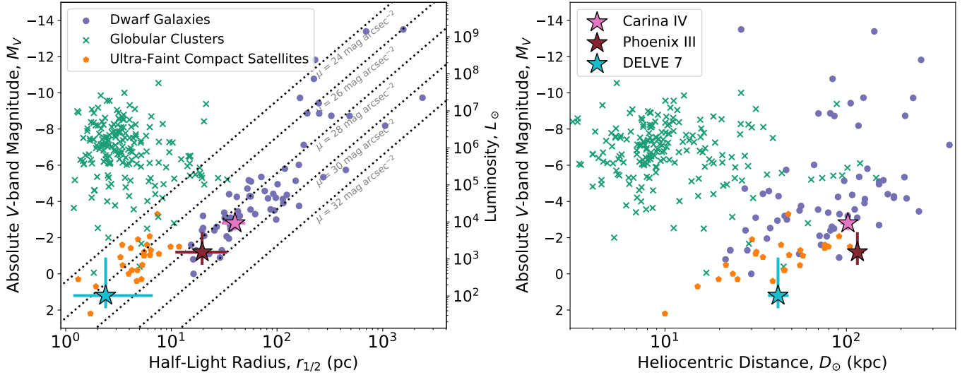
Figure 6. (Left) Absolute V -band magnitude ( M_V ) versus azimuthally averaged physical half-light radius ( r_{1/2} ) for the three new Milky Way satellites and the population of known Local Group globular clusters and dwarf galaxies. (Right) The same diagram, but showing M_V versus heliocentric distance ( D_{\odot} ). Spectroscopically confirmed dwarf galaxies and likely galaxy candidates are shown in purple circles, while Milky Way globular clusters are shown with green ‘x’ symbols. Ambiguous ultra-faint compact satellites are shown with orange pentagon symbols. The three systems discovered in this work are shown as colored stars with bars representing 68% posterior uncertainty intervals. Data on the Milky Way satellite population were compiled by Pace (2025), and we adopt the same classifications as Tan et al. (2025a).
