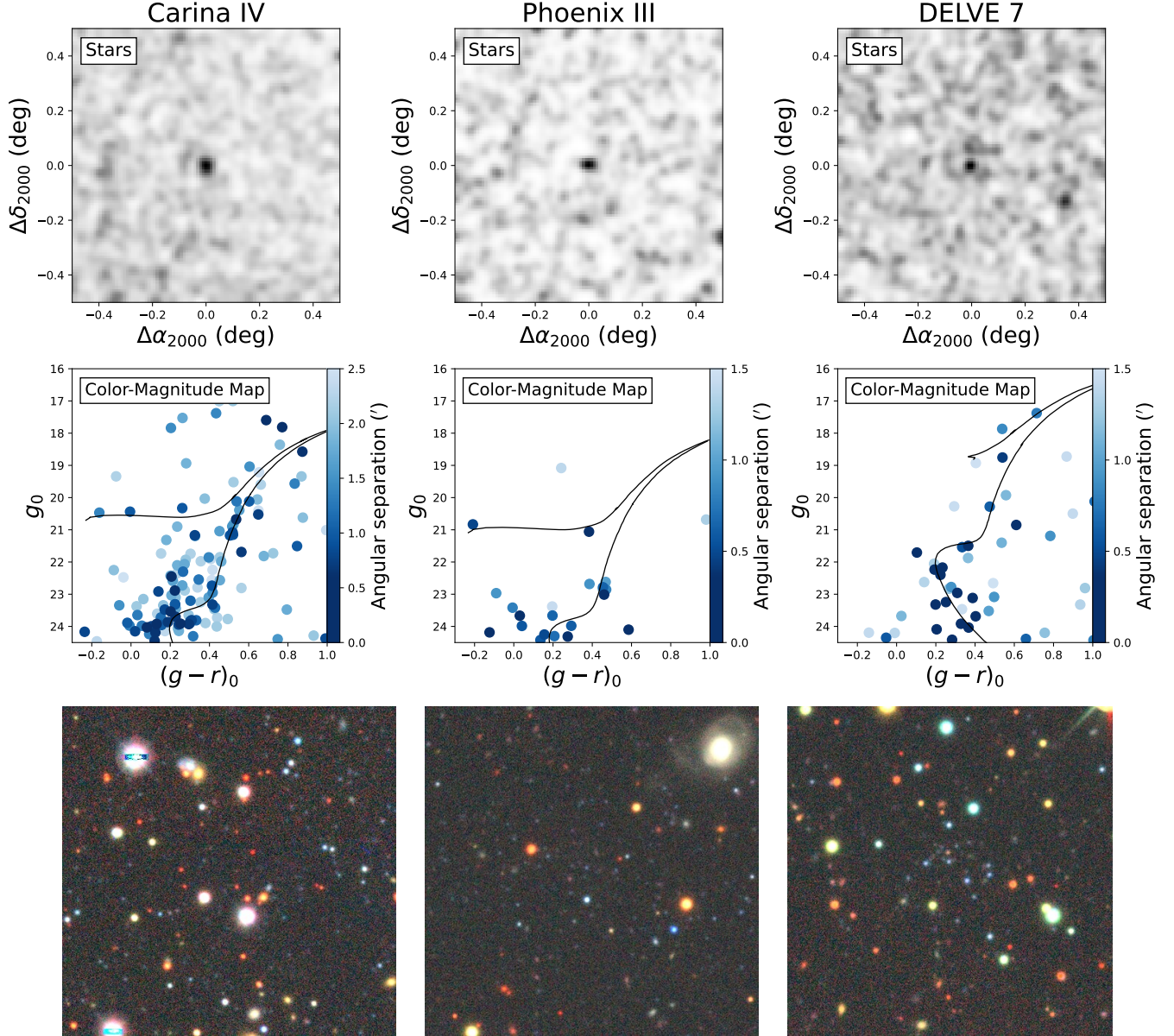
Figure 1. Diagnostic plots for each of the three newly-discovered satellites, closely matching those used to identify the systems in our search. (Top) Stellar density maps for a 1^\circ \times 1^\circ degree region centered on each candidate, smoothed with a 0.5 Gaussian kernel. (Middle) Color-magnitude diagrams for stars within 2.5 of Carina IV and 1.5 of Phoenix III and DELVE 7, centered on each candidate system. Stars are colored by separation from each system’s centroid, with darker colors representing smaller separations. Also overlaid is the best-fit old, metal-poor PARSEC isochrone, with parameters taken from the best-fit ugal results in Table 1. (Bottom) False-color coadded images ( \sim 2' \times 2' , \sim 0.03^\circ \times 0.03^\circ ) of Carina IV, Phoenix III, and DELVE 7 from the Legacy Surveys Sky Viewer DR10. Each cutout has been artificially brightened by a factor of 1.8\times to highlight faint sources.
