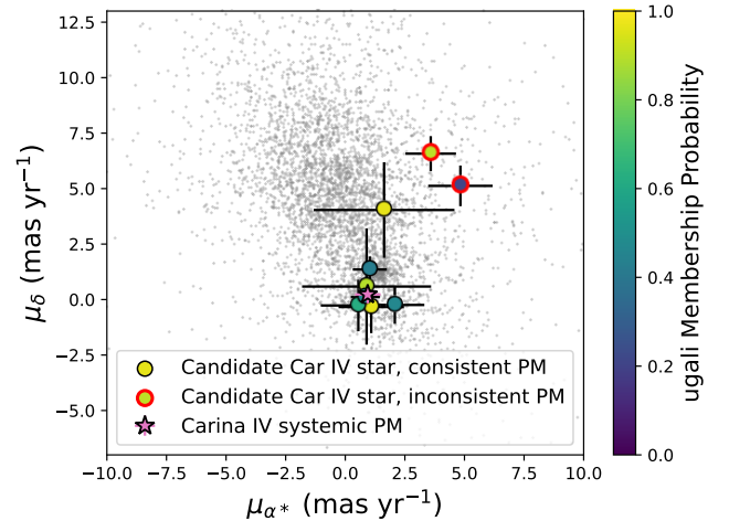
Figure 4. Proper motion of candidate member stars in Carina IV using data from Gaia DR3. The cluster of stars at (\mu_\delta, \mu_{\alpha*}) \sim (0, 0) mas/yr indicate the presence of a halo system. We outline in red the candidate stars whose proper motions deviate by more than 2\sigma from the systemic Carina IV proper motion (shown as the pink star). Stars within 0.5' of Carina IV with a low ugali membership probability ( p < 0.20 ) are shown in grey.
