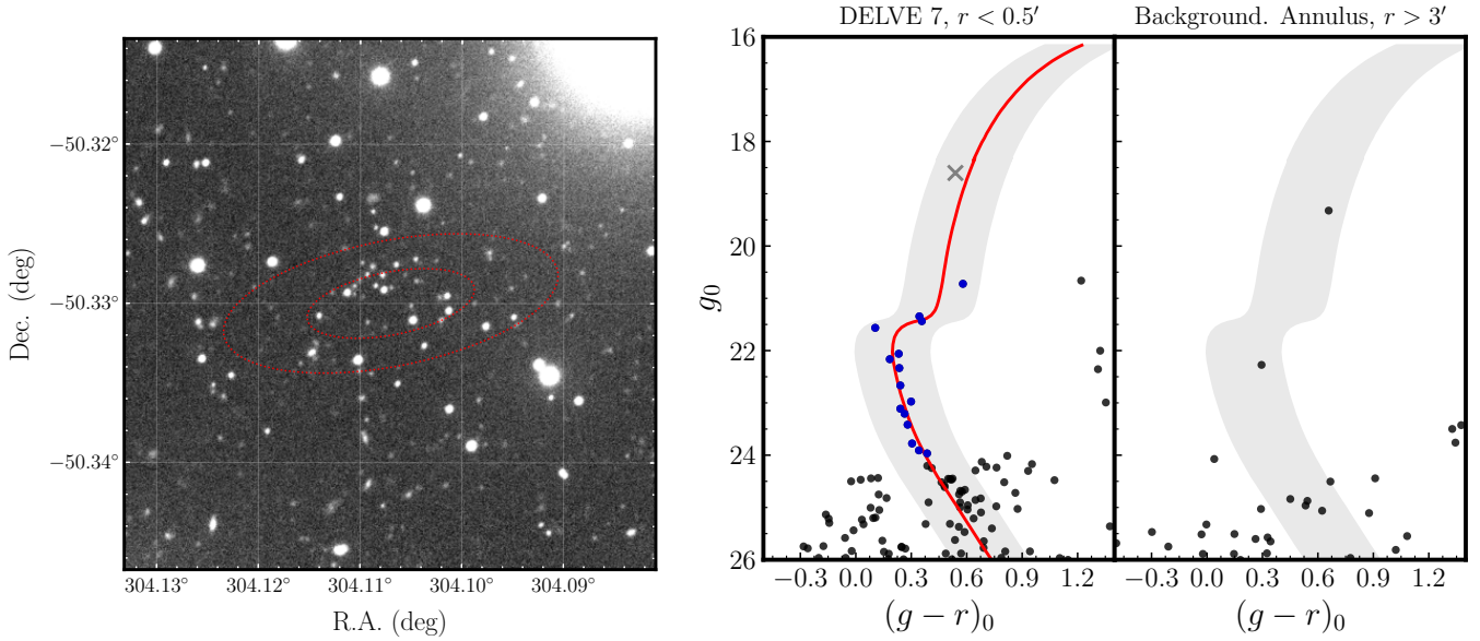
Figure 3. Follow-up imaging of DELVE 7 performed with Magellan/IMACS. (Left) 2' \times 2' g -band cutout image centered on DELVE 7, which can be seen as a clear overdensity of faint point-like sources. We overlay red ellipses demarcating a_h and 2a_h . (Right) Color-magnitude diagrams for point-like sources in the vicinity of DELVE 7. The left panel shows a circular region with r < 0.5' while the right panel shows an equal-area background annulus with inner radius r = 3' . Stars used for the isochrone fit are shown in blue; the best-fit isochrone (shown in red) was found to be \tau = 10 Gyr, Z = 0.00061 , (m - M)_0 = 18.1 . Although one bright candidate RGB member falls close to the isochrone, this star has a Gaia parallax of \varpi = 0.71 \pm 0.15 mas that places it well in the foreground of DELVE 7; we mark it here with an ‘x’ to emphasize its non-membership. The shaded regions show \pm 0.2 in color about the best-fit isochrone.
