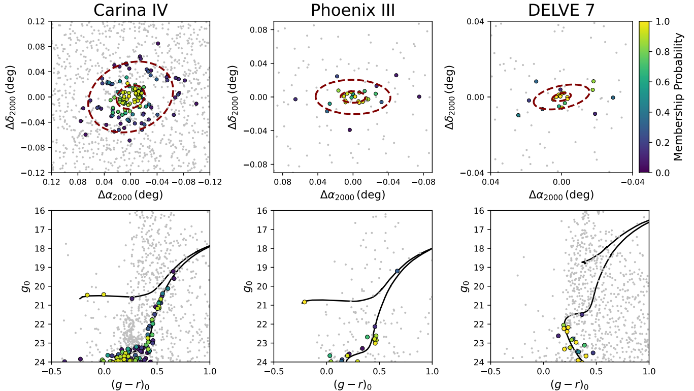
Figure 2. The spatial distributions (top) and color-magnitude diagrams (bottom) for likely member stars in Carina IV (left), Phoenix III (center), and DELVE 7 (right). Stars are colored by their membership probabilities derived as part of our ugali characterization analysis, which incorporates the spatial, photometric, and color information of each star. Stars with a lower ugali membership probability ( p < 0.05 ) are shown in grey. The top panels also show ellipses representing the ugali best-fit half-light radius, r_h , and three times this half-light radius, 3r_h , for each system. Carina IV is the best-populated of the three systems, featuring a clear main-sequence turn off (MSTO), red giant branch (RGB), and blue horizontal branch (BHB). Phoenix III is at a similar distance, but it is fainter with only a handful of likely member stars. DELVE 7 is substantially fainter, featuring no highly-probable RGB members and is potentially only comprised of main-sequence stars. This lack of RGB stars is consistent with other faint Milky Way satellites at M_V > 0 (e.g., DELVE 5, Kim 3, and Ursa Major III/UNIONS 1).
