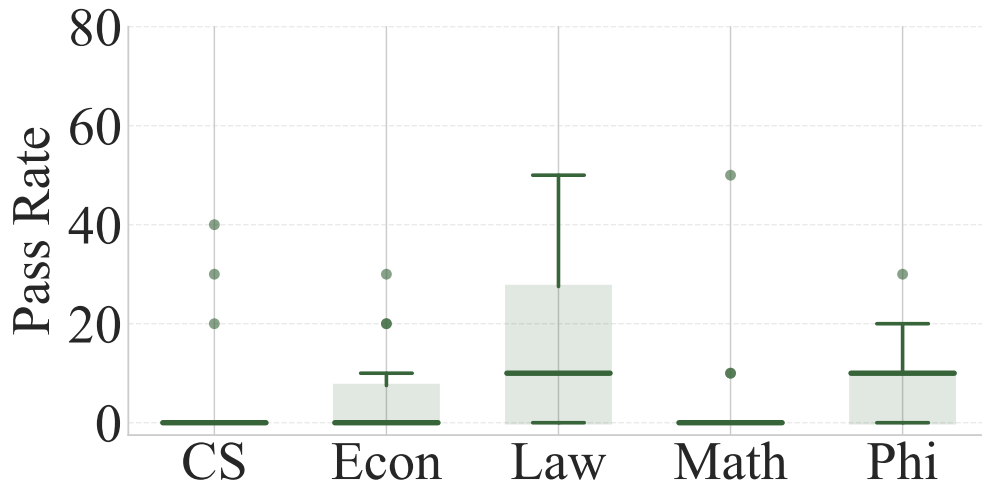
Figure 11 General performance on different domains with Pass Rate.
