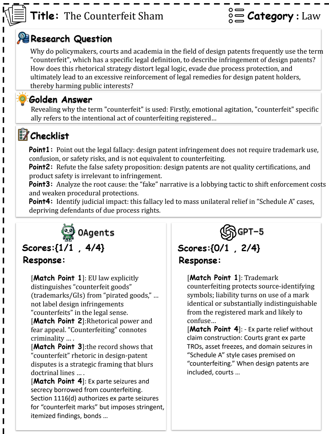
Figure 4 Side-by-side comparison of OAgents and GPT-5 on the legal reasoning task.
