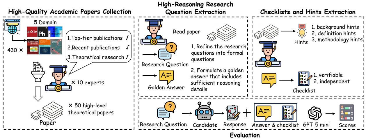
Figure 1 Overview of the ACADREASON benchmark construction and evaluation pipeline. It consists of three stages: (1) High-Quality Academic Papers Collection – experts filter 430 papers across 5 domains into 50 top-tier theoretical works; (2) High-Reasoning Research Question Extraction – research questions are refined into formal queries with golden answers containing sufficient reasoning; (3) Checklists and Hints Extraction – background, definition, and methodology hints are provided together with verifiable, independent checklists. For evaluation, candidate responses are compared against golden answers and checklists, and GPT-5 mini assigns final scores.
