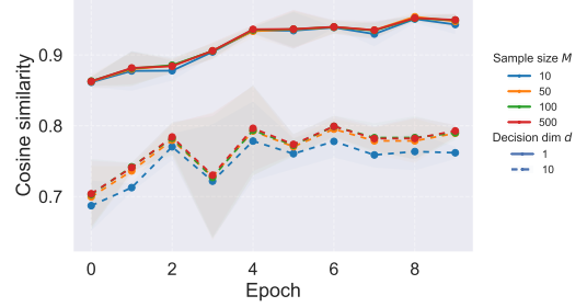
Figure 2: Cosine similarity between the reparameterization and score function gradient across different dimensions.
