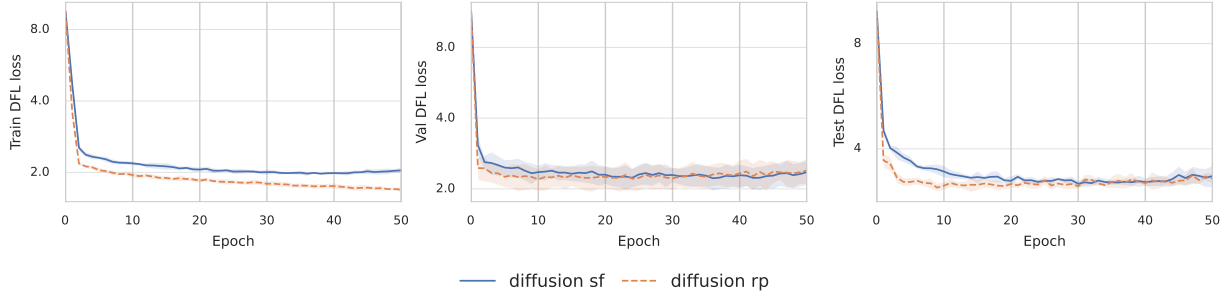
Figure 8: Score function vs. Reparameterization
