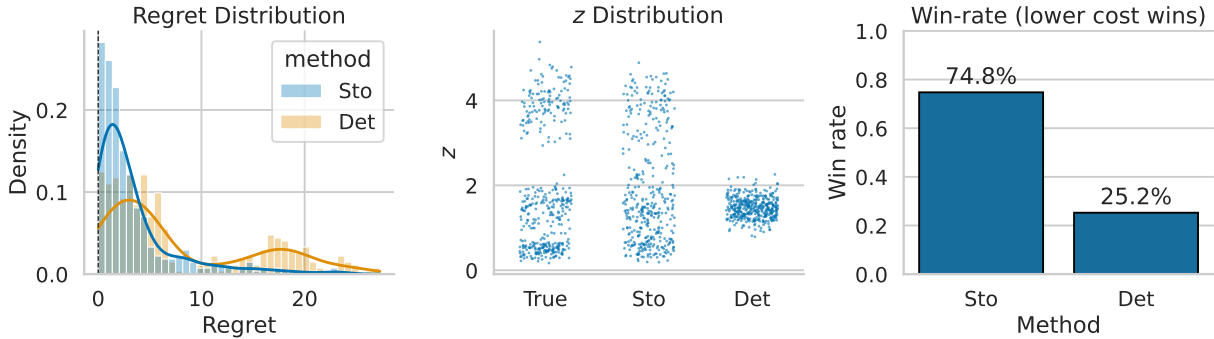
Figure 10: Toy decision task comparing deterministic and diffusion DFL. Left : distribution of per-instance regret (lower is better). Middle : distribution of chosen decision z in the lower-level; the stochastic method tracks the true distribution z^* more closely. Right : pairwise win-rate on test set; a large fraction of costs from the stochastic method are lower than the deterministic one, indicating that modeling uncertainty yields better decisions.
