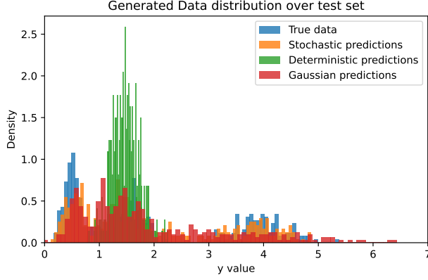
Figure 11: Prediction distribution for inventory stock problem.
