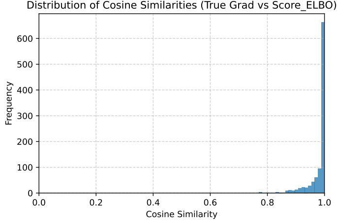
Figure 6: Compare the cosine similarity between the true gradient and the estimated gradient using a linear model.
