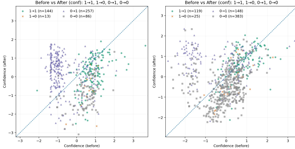
Figure 5: Confidence dynamics before and after UCAS training on the MATH and Olympiad datasets.
