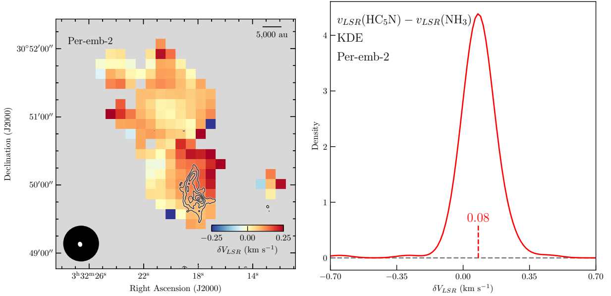
Figure 9. Velocity differences between \text{HC}_5\text{N} and \text{NH}_3 line emission. Left panel shows the velocity difference between a single Gaussian fit to the \text{HC}_5\text{N} line and the hyperfine fit of \text{NH}_3 obtained by GAS. A clear velocity gradient connects the streamer and the main gas reservoir. Overlaid in contours is the \text{HC}_3\text{N} (10–9) integrated intensity from NOEMA (J. E. Pineda et al. 2020). The beam sizes and scale bars are shown in the bottom left and top right corners, respectively. The right panel shows the KDE of the velocity difference in the regions shown in the left panel. The vertical line shows the median value of the velocity difference.
