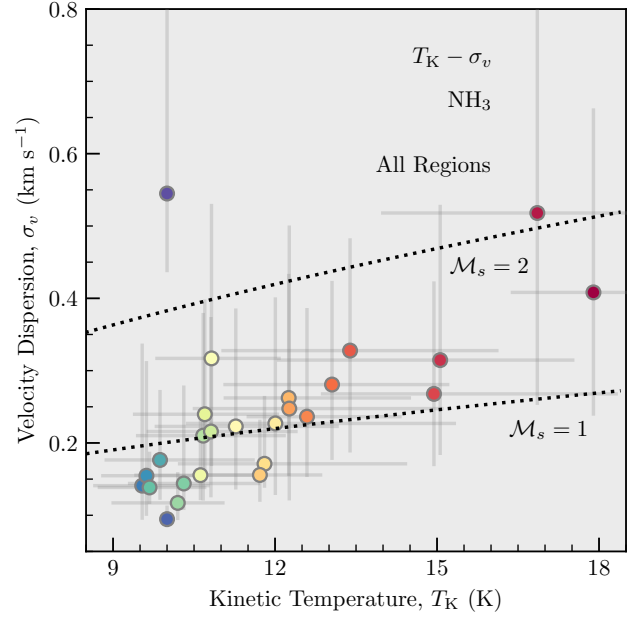
Figure 11. Comparison of typical velocity dispersion and kinetic temperature for all regions. Symbols show the 50 th , 16 th , and 84 th percentiles of the values for each region, with asymmetric uncertainties. The color of the symbols corresponds to the mean T_K , consistent with Fig. 3. The dotted lines indicate the expected velocity dispersions for sonic Mach numbers of \mathcal{M}_s = 1 and \mathcal{M}_s = 2 .
