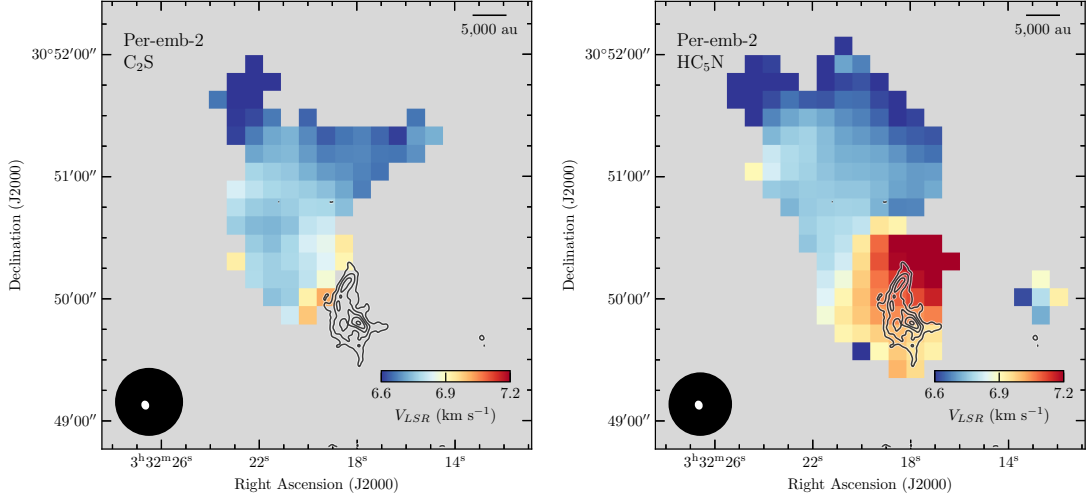
Figure 8. Velocity maps obtained towards Per-emb-2 from a single Gaussian fit to the \text{C}_2\text{S} and \text{HC}_5\text{N} data cubes from GAS. A clear velocity gradient connects the streamer and the main gas reservoir. Overlaid in contours is the \text{HC}_3\text{N} (10–9) integrated intensity from NOEMA (J. E. Pineda et al. 2020). The beam sizes and scale bars are shown in the bottom left and top right corners, respectively.
