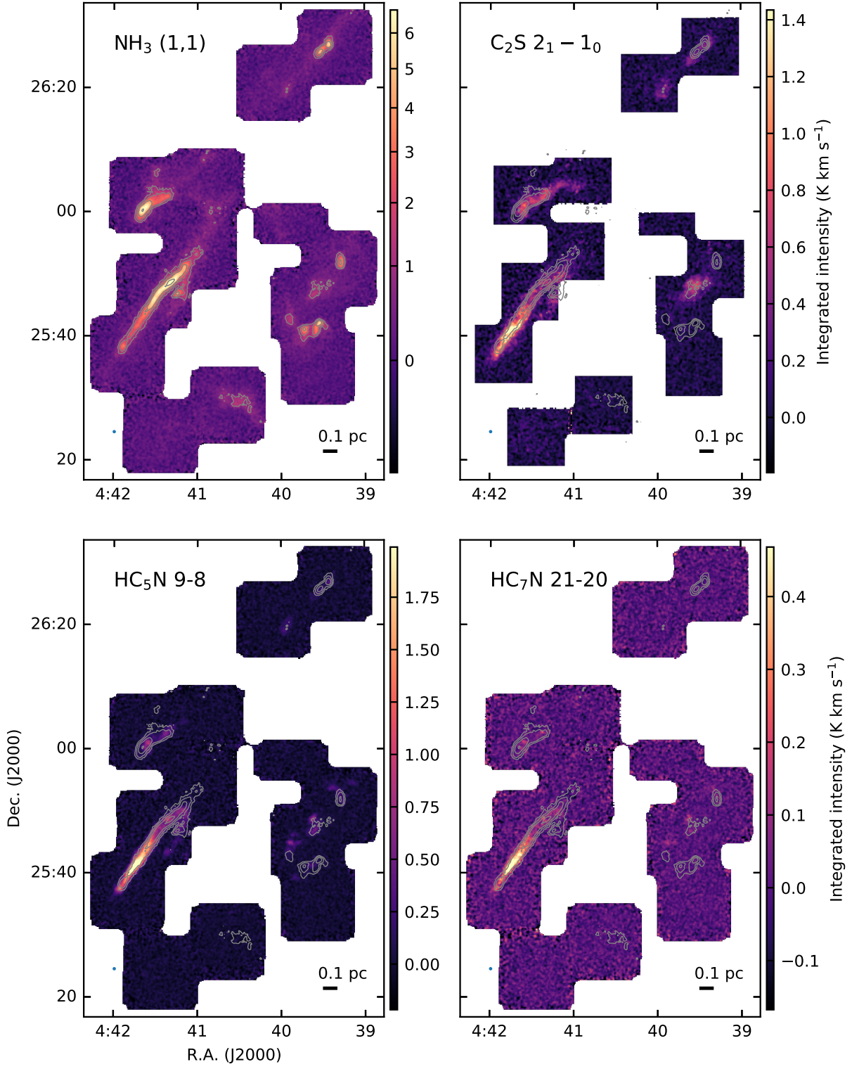
Figure 2. Integrated intensity of \text{NH}_3 (1,1), \text{C}_2\text{S} , \text{HC}_5\text{N} , and \text{HC}_7\text{N} emission toward Heiles Cloud 2 in Taurus. In all plots, grey contours follow the \text{NH}_3 (1,1) emission. The blue circle at lower left shows the GBT beam
