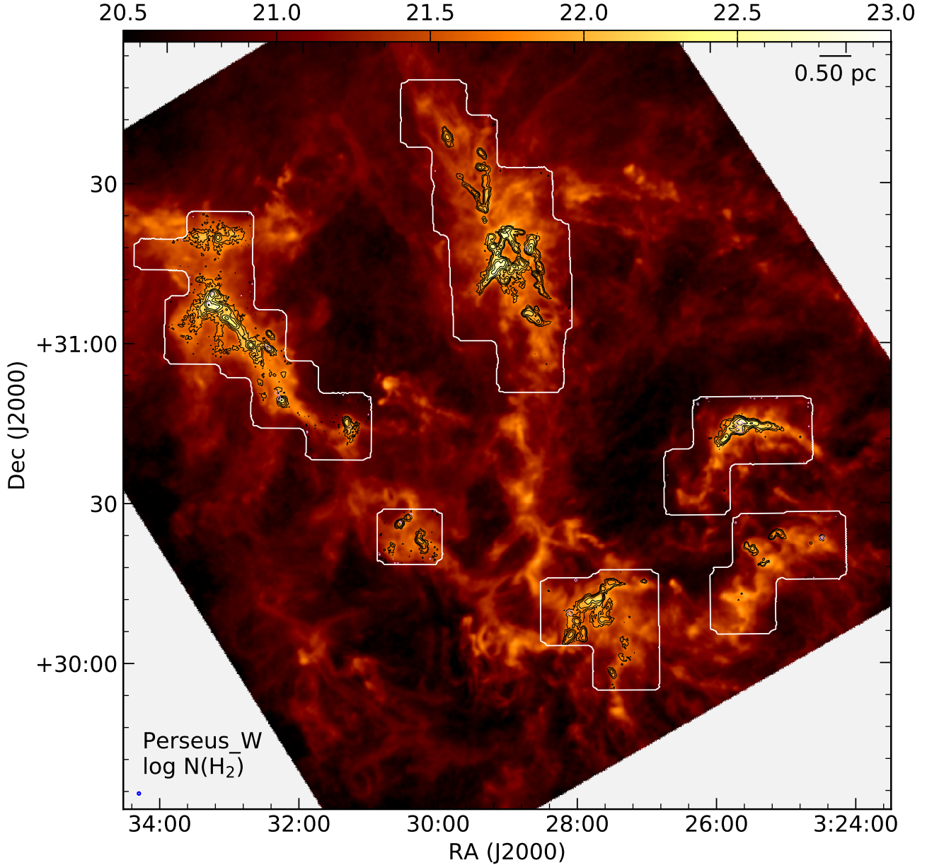
Figure 1. Observed GAS regions in the western Perseus molecular cloud. The color scale shows N(\text{H}_2) derived from SED fitting of Herschel continuum maps (A. Singh & P. G. Martin 2022). White contours highlight the extent of the GAS maps. Black contours show the integrated \text{NH}_3 (1,1) emission. The 32'' GBT beam is shown at bottom left.
