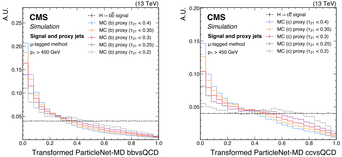
Figure 19: Shapes of the transformed ParticleNet-MD X \rightarrow b\bar{b} (left) and X \rightarrow c\bar{c} (right) discriminants for SM H \rightarrow b\bar{b} ( c\bar{c} ) signal jets and proxy jets selected with different \tau_{21} selection thresholds. The examples correspond to the calibration of the ParticleNet-MD X \rightarrow b\bar{b} and X \rightarrow c\bar{c} discriminants with the \mu -tagged method, using simulated events under 2018 data-taking conditions for jets with p_T > 450 GeV. The error bars represent the statistical uncertainties due to the limited number of simulated events.
