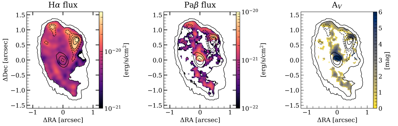
Fig. C.1. Line emission from medium-band F210M and F410M NIRCam imaging. From the left, we show maps of recovered H\alpha and Pa\beta line flux (not corrected for dust attenuation), and finally of nebular A_V , as inferred from Pa\beta/H\alpha line ratios. Black solid and dashed contours are the same as in Fig. 4.
