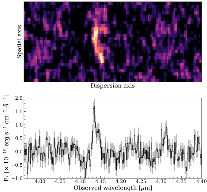
Fig. 3. Continuum-subtracted NIRCам F444W WFSS data of K20-ID7, zoomed-in over 3.95 - 4.40 \mu\text{m} , encompassing \text{Pa}\beta line emission. In the 2D slitless spectra (upper panel), \text{Pa}\beta line emission is clearly spatially resolved perpendicularly to the dispersion axis, and also extended along the parallel direction, which leads to a double-peaked \text{Pa}\beta line profile in the total 1D spectrum (lower panel). This is consequence of resolved spatial offsets combined with velocity gradients along the grism dispersion axis (discussed in Sect. 5).
