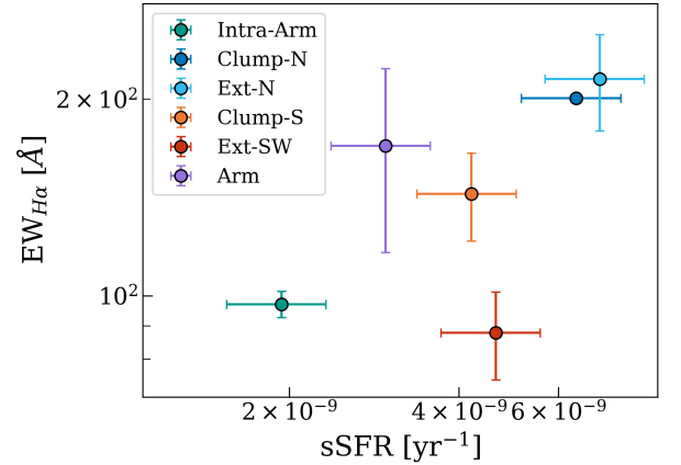
Fig. 7. Rest-frame \text{EW}(\text{H}\alpha) as a function of sSFR for the various galaxy regions probed by distinct MSA shutters. \text{EW}(\text{H}\alpha) measurements are derived from PRISM/CLEAR data, while sSFRs from our SED-based SFR10 and M_* maps. The plot highlights a correlation between the two quantities, with higher \text{EW}(\text{H}\alpha) values at higher sSFR, which is also indicative of younger stellar populations.
