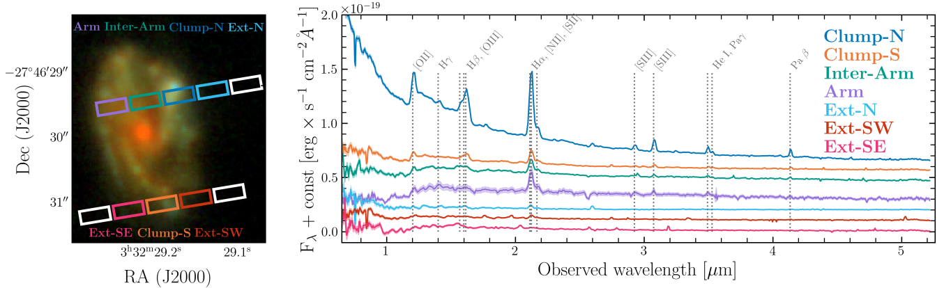
Fig. 2. NIRSpec MSA spectroscopy of K20-ID7. Left: Location of the two distinct MSA mask arrays, with open shutters drawn on the top of a NIRCcam RGB image of K20-ID7, composed of F356W+F444W (red), F182M+F200W+F277W (green), and F090W+F115W+F150W (blue) filters. Right: PRISM/CLEAR spectra extracted from the seven coloured MSA shutters (those exhibiting some galaxy emission, same colors as in the left panel), using our custom-made reduction (described in Sect. 2.2). White shutters do not contain any galaxy emission. Spectra from different regions clearly differ in continuum shape and line intensities, over the total covered rest-frame near-UV to near-IR wavelength range. For the purpose of a better visualization, each spectrum has been vertically shifted by an arbitrary constant.
