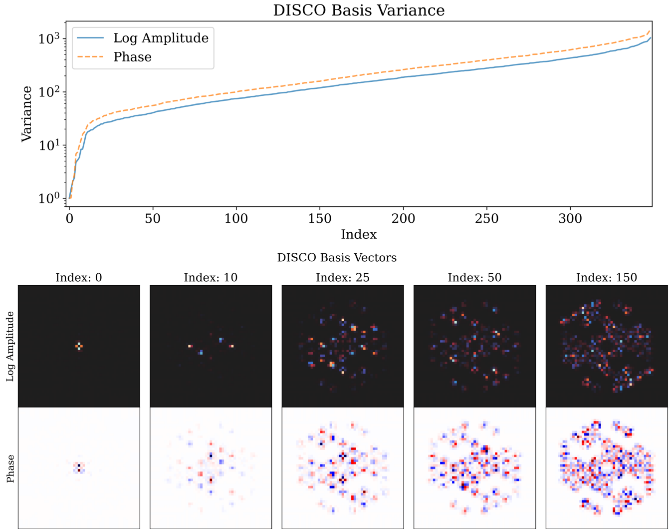
Figure 7. Example Delay-Insensitive Subspace of Calibrated Observables (DISCO) basis vectors found from the GO 1843 observation, discussed in Section 7.3. Top panel: Normalised log amplitude and phases basis vector variances. Bottom panel: Selection of representative DISCO basis vectors. Matching with the latent visibility basis vectors, low index vectors are better constrained and have lower spatial fidelity.
