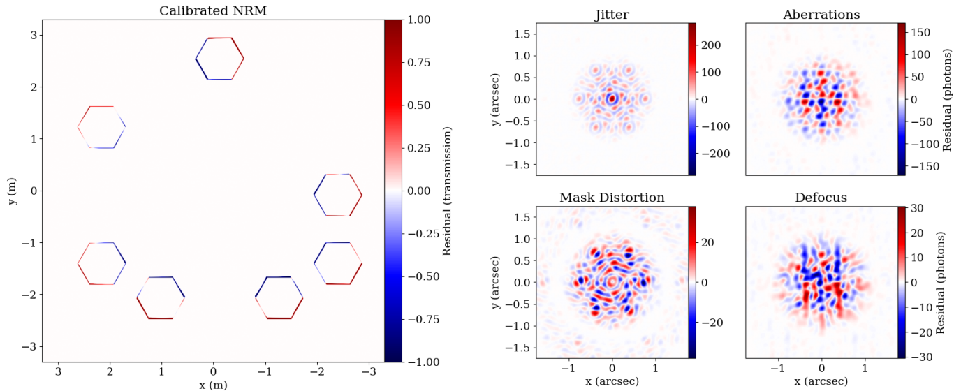
Figure 4. Left panel: Residual between the calibrated aperture mask and its idealised undistorted counterpart. Right panel: PSF residuals of the four primary optical effects on the PSF. Top left: Instrumental jitter, applied through a convolution with a Gaussian kernel. Top right: Primary mirror aberrations, modelled using Zernike polynomials on the primary. Bottom left: Aperture mask distortions, modelled by applying a distortion to the coordinates over which the aperture mask is calculated. Bottom right: Fresnel defocus modelled using a Fresnel propagation algorithm. All effects are shown for the F430M filter, using a PSF with 10^6 total photons.
