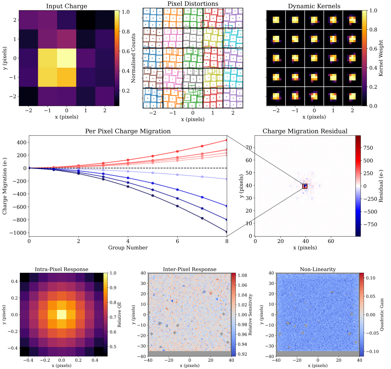
Figure 9. Demonstration of the EDM BFE model and recovered detector parameters. Starting with the normalised input charge distribution (top left), the CNN predicts a series of distortion coefficients that are applied to a 3\times oversampled set of coordinates for each pixel. The distorted output pixel positions are visualised in the top middle panel. These output positions have their overlap fractions with each neighbouring pixel calculated in order to produce a set of flux conservative convolutional kernel for each pixel, shown in the top right panel. This dynamic convolution is applied to the predicted input illuminance pattern for a fixed number of time steps. The middle left panel shows the charge migration between a set of pixels around the brightest region of the PSF as charge is accumulated up the ramp. The middle right panel shows the cumulative charge migration between pixel for each individual pixel. The bottom row shows the various recovered pixel-level effect. The bottom left panel shows the recovered intra-pixel sensitivity variations, applied through a simple quadratic function. The Amigo model only uses a 3\times oversample, but is visualised here with 9\times oversample. The bottom middle panel shows the inter-pixel sensitivity variations, ie the flat-field. The resulting distribution of sensitivities shows similar properties to the existing JWST pipeline calibrations. The bottom right panel shows the recovered quadratic non-linear gain term applied through the electronics model. Every pixel shows the expected negative gain as a function of pixel depth, in line with existing calibrations.
