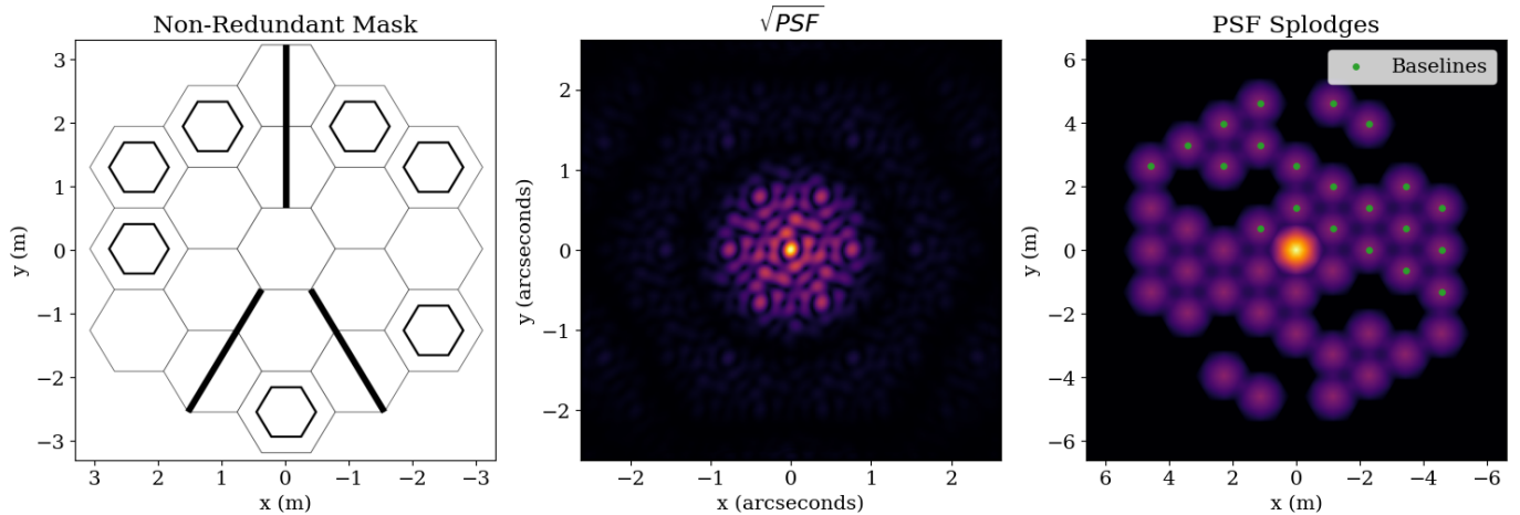
Figure 1. Left panel: Schematic diagram of the 7-hole NRM projected over the primary mirror. Middle panel: The resulting PSF (i.e. interferogram) from the non-redundant mask, visualised on a square-root scale to highlight low-power features. Right panel: The power-spectrum of the PSF featuring baseline-specific regions of fringe power known in the literature as splodges that can be conveniently found by Fourier transform of the PSF. The 21 discrete non-redundant baselines are indicated by the overlaid green dots.
