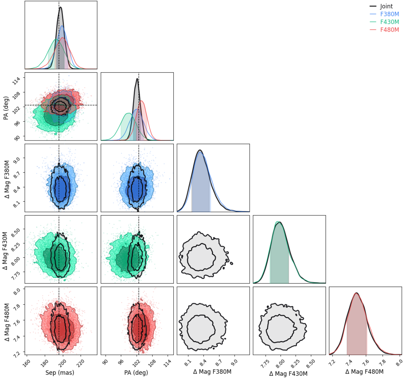
Figure 17. Joint posterior distributions from an MCMC fit to the HD 206893 B companion. Two fit types are shown: Joint — simultaneously modelling astrometry and photometry across all three filters — and per-filter fits. While both companions are fit simultaneously, only the B companions samples are shown here for clarity. The parameters shown include the separation (mas), position angle (degrees), and contrasts ( \Delta mag) in the F380M, F430M, and F480M bands. The joint-fit samples are shown in black. One- and two- \sigma credible regions are shown in dark and light shades, respectively. The tight constraints in both astrometry and photometry reflect the high signal-to-noise of the companion detection. The expected position predicted by GRAVITY orbit fits (with a precision of \sim 1 mas) are overlaid in a black dashed line, showing strong agreement with AMI, both in each filter and in the joint-fit.
