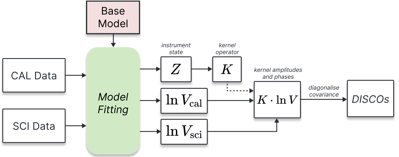
Figure 12. Schematic diagram of the basic workflow of extracting the DISCOs from data.
