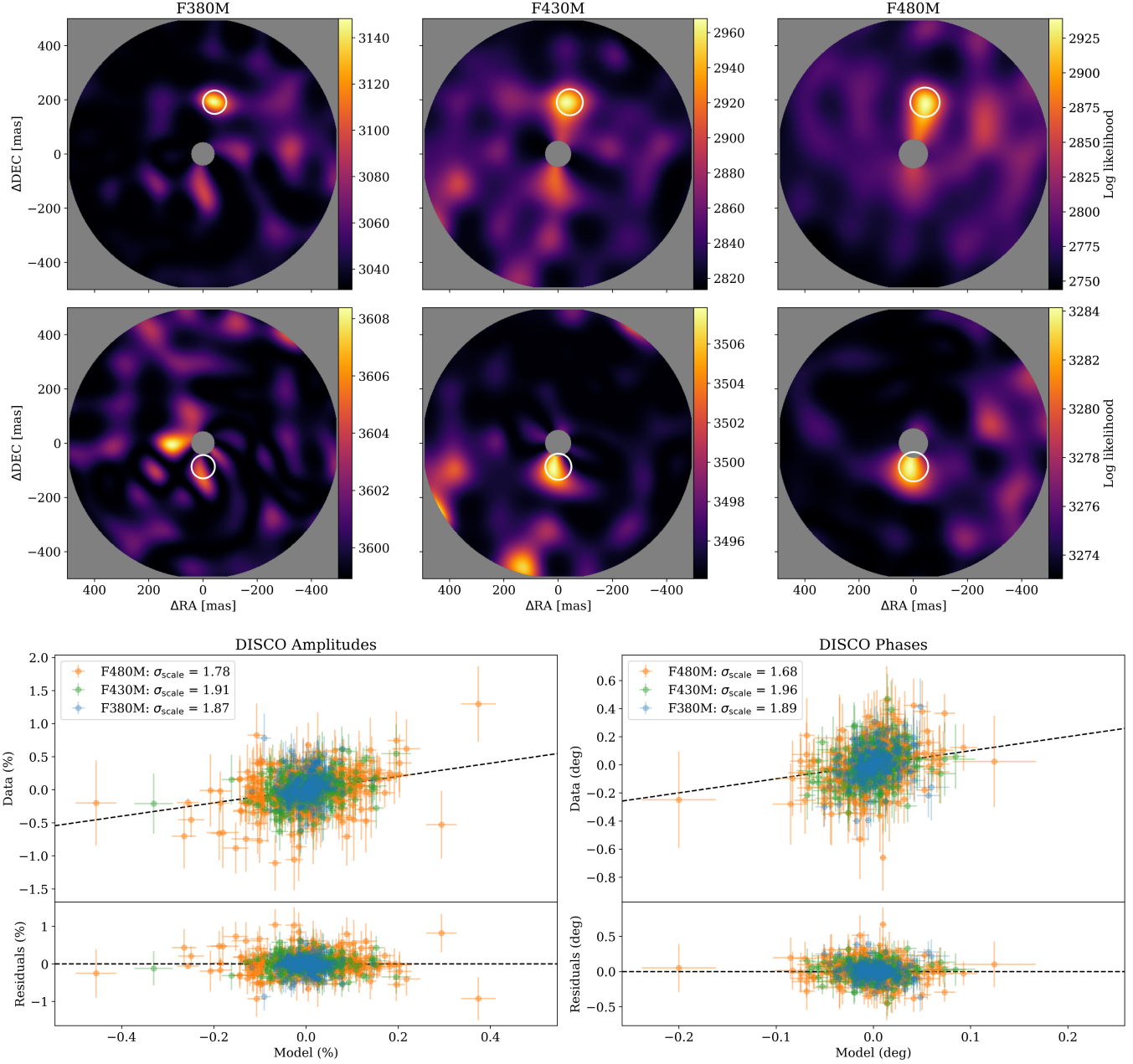
Figure 16. Summary of the fits to the HD 206893 companions. The top two panels show the marginalised log-likelihood surface as a function of companion offset in \Delta RA and \Delta DEC , revealing a strong and consistent peak in all filters. The top row shows the detection maps for the full data, with the GRAVITY prediction for the B companion shown as a white circle. The middle row shows the detection map after the best-fit B companion has been subtracted from the data, revealing the inner c companion being consistently detected in all three filters, with the GRAVITY prediction overlaid with a white circle. The peaks in each filter for both companions can be seen matching the expected positions. The greyed central region denotes the IWA masked by the interferometric null. The bottom panels show the predictive posterior check comparing AMIGO recovered DISCO amplitudes (left) and phases (right) against the predicted values from the MCMC samples, for the three filters: F380M, F430M, and F480M. Each panel shows individual measurements with 1\sigma error bars, with the top panels plotting model predictions against data and the lower panels showing residuals. The black dashed line represents the 1:1 line for a perfect model prediction. Scale factors \sigma_{scale} are applied to the observational uncertainties in MCMC with the effect of ensuring \chi^2_{\nu} \approx 1 and are quoted in the legend for each filter. The agreement across filters and observables confirms the validity of the forward model and appropriate uncertainty quantification in the recovered posterior.
