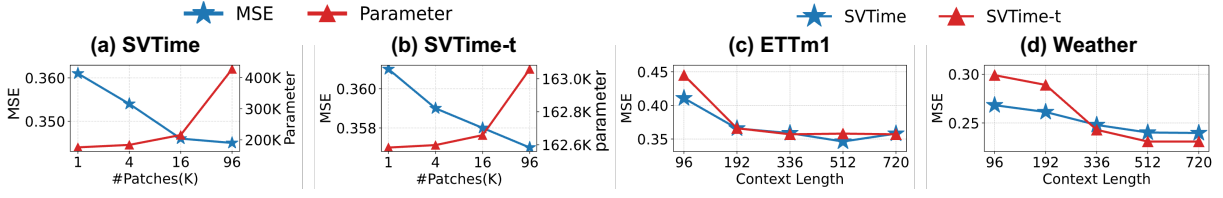
Figure 7: Results on the impact of the number of patches K on (a) SVTIME; and (b) SVTIME-t in terms of LTSF performance and model size; and the impact of lookback window (or context) length on both models using (c) ETTm1; and (d) Weather datasets.
