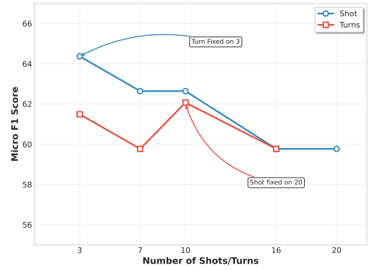
Figure 3: Impact of varying the number of examples and turns on final evaluation performance. We observe a negative correlation with the number of examples, likely attributable to the “lost-in-the-middle” problem (Liu et al., 2023).
