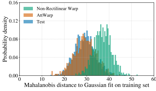
(a) Analyzing data shift.
