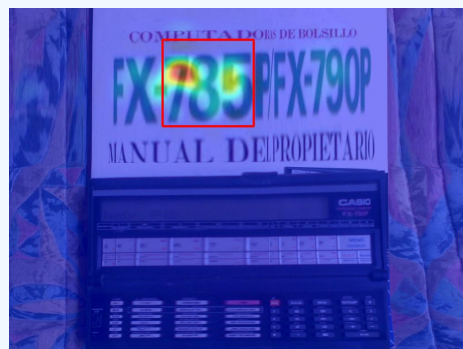
Warped Output
