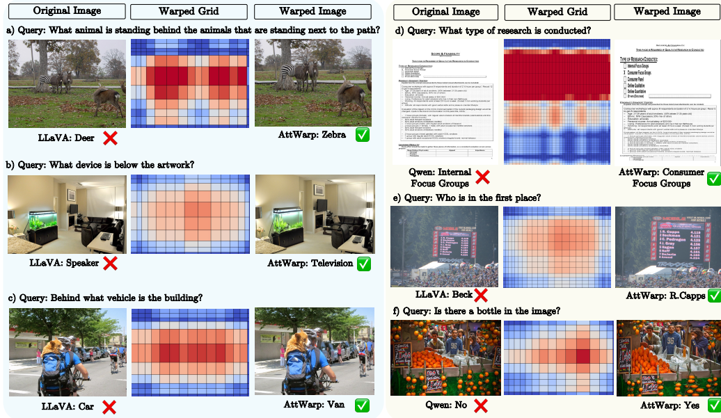
Figure 3: The figure shows the original image, the rectilinear warping function visualized as a warped grid, and the corresponding warped image. AttWarp enhances compositional and spatial reasoning, as illustrated by examples from the GQA dataset: (a) expanding the region containing the zebra behind the path, (b) expanding the television below the artwork, and (c) expanding the walls of the building. It also improves text understanding in document-based and real-world images: (d) expanding the phrase "consumer focus groups" (DocVQA), and (e) expanding the player's name on the board (TextVQA). Additionally, it aids fine-grained perception of small and occluded objects, exemplified by (f) the expansion of a bottle region in the POPE dataset.
