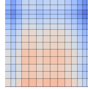
Warped Grid
