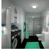
MLLM: Basket
