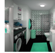
AttWarp: Dryer
