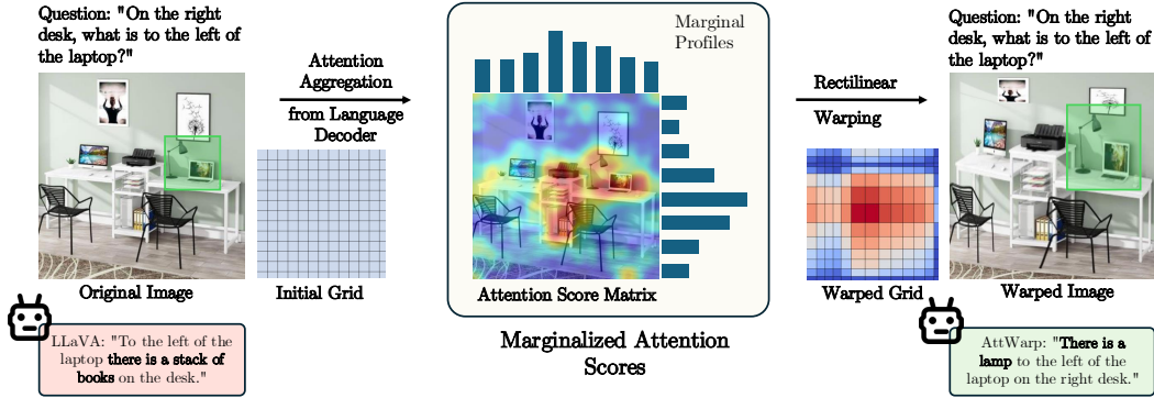
Figure 1: AttWarp overview. Given a query, our method extracts cross-modal attention maps from the MLLM’s language decoder, aggregates them into marginal attention profiles, and uses rectilinear warping to expand high-attention regions while compressing low-attention areas. The warped image is then processed by the same MLLM, which now produces the correct answer.
