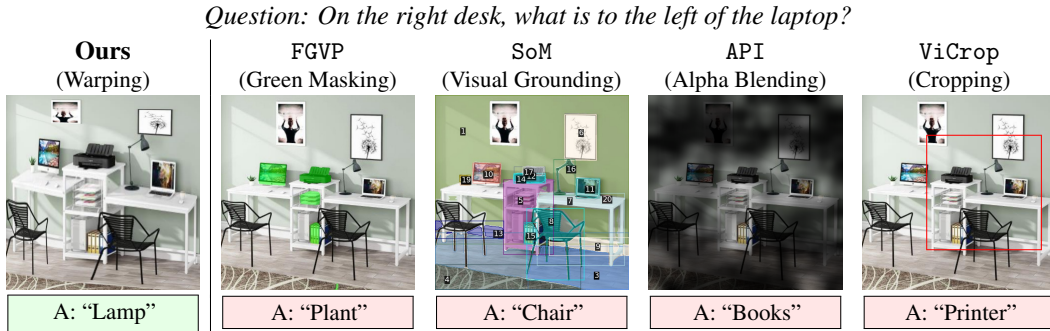
Figure 4: Qualitative comparison of AttWarp and baselines of test-time visual intervention. While plausible, the answers generated by prior works are incorrect. The answer (A) for each case is generated with LLaVA.
