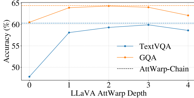
Figure 11: Impact of iterative warping depth on accuracy for TEXTVQA and GQA. Fixed-length warping initially improves performance but degrades with excessive iterations due to recursive instability. The adaptive AttWarp-Chain (dashed lines), guided by the KL divergence stopping criterion, consistently achieves the best accuracy while avoiding over-warping.
