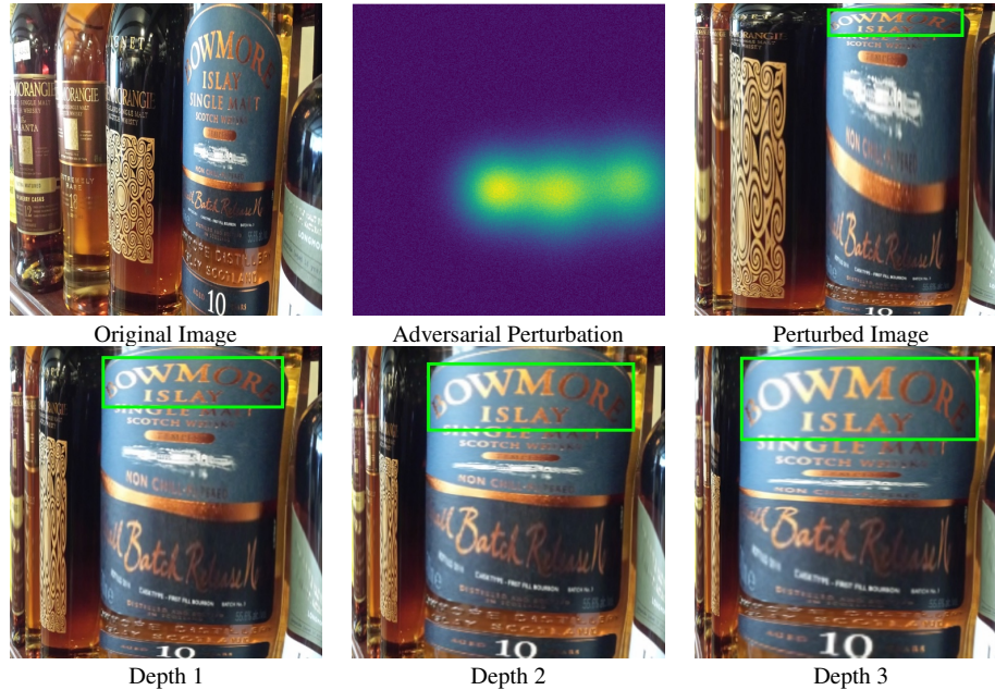
Figure 10: (top row) the original image, the adversarial perturbation designed to corrupt attention, and the resulting perturbed image in which the task-relevant region is shrunk; (bottom row) outputs of AttWarp at Depth 1–3, illustrating how our method progressively overcomes the interference to refocus on the relevant region.
