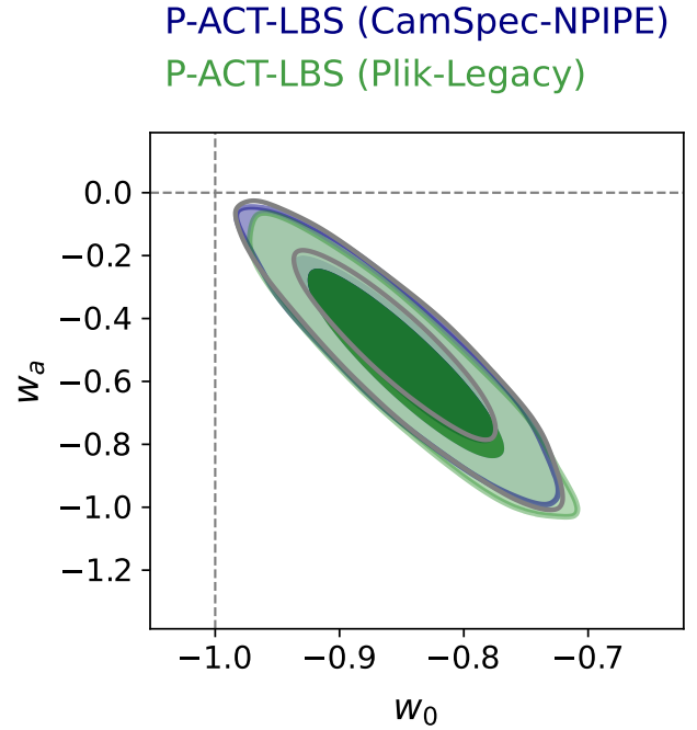
Figure 10. Constraints on w_0 w_a from P-ACT-LBS using either Plik-Legacy (green) or CamSpec-NPIPE (dark blue). The dashed lines denote \Lambda CDM at w_0 = -1, w_a = 0 . The empty grey contour uses the same data combination but with non-marginalized CamSpec-NPIPE likelihood. The contours are insensitive to the choice of Planck .
