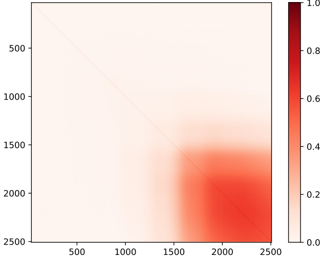
Figure 2. The TTTT subblock of the correlation matrix. The marginalization over foregrounds captures a lot of information in the \ell > 1500 part of the covariance, leading to high correlations between different bins.
