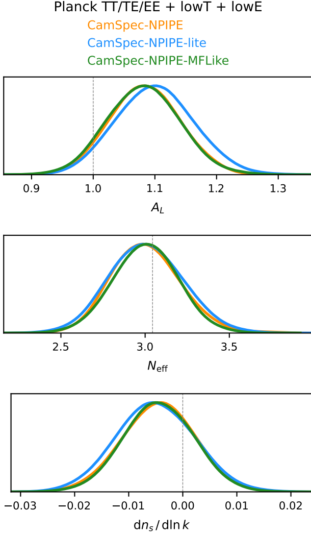
Figure 5. Comparison of the constraints on select single-parameter extensions to \Lambda CDM as obtained from the full Planck TT/TE/EE+lowT+lowE dataset using the original CamSpec -NPIPE likelihood (orange), our implementation in MFLike (green), and our CamSpec -NPIPE-lite likelihood (blue). We show the constraints on the lensing peak smearing amplitude A_L (top panel), the effective number of relativistic species N_{\text{eff}} (middle panel), and the running of the spectral index dn_s/d \ln k (bottom panel). We observe that foreground marginalization has little effect on the constraints of extension models. The constraints from the lite likelihood are consistent and at most 5 – 10% wider than those from the full likelihoods. The vertical lines show the expected values of these parameters in \Lambda CDM.
