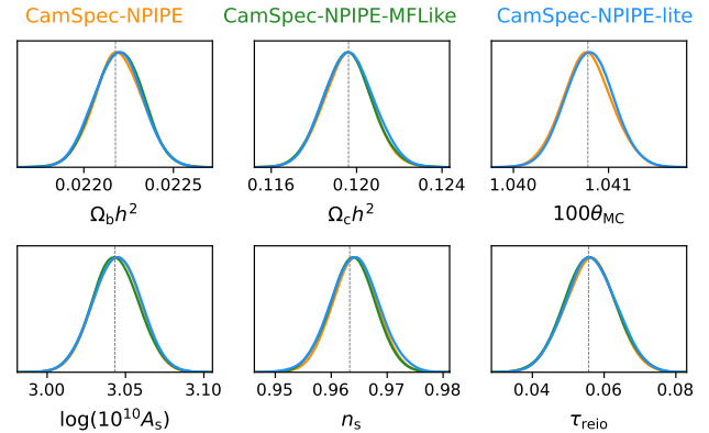
Figure 4. Posteriors of the \Lambda CDM cosmological parameters recovered from different implementations of the CamSpec-NPIPE likelihood. We find very good agreement in all five free parameters (we infer the optical depth \tau_{\text{reio}} through a prior), and see only a slight widening of 9% on the constraint on n_s from the lite likelihood due to the foreground marginalization. All posteriors are obtained with the full Planck TT/TE/EE+lowT+lowE dataset. The vertical lines indicate the best-fitting values from the CamSpec-NPIPE chain (original likelihood, shown in orange).
