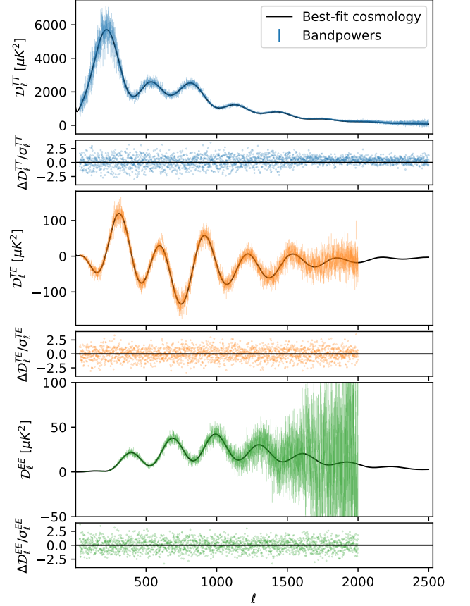
Figure 1. CMB foreground-marginalized CamSpec-NPIPE spectra. The TE and EE spectra appear normal distributed around the best-fitting model, as does the TT spectrum below \ell < 1500 . At \ell > 1500 , the TT datapoints are highly correlated and the full behaviour of the data is captured in the covariance matrix.
