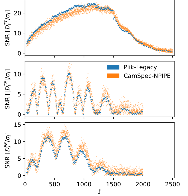
Figure 6. Comparison of the signal-to-noise ratios \mathcal{D}_\ell/\sigma_\ell of Plik -Legacy (blue) and CamSpec -NPIPE (orange) after foreground-marginalization. The Plik data points contain an additional factor of \sqrt{\Delta\ell} to correct for the bin widths of the data, while the NPIPE is plotted with an additional 1% error margin since the likelihood marginalizes over additional TE and EE calibration factors.
