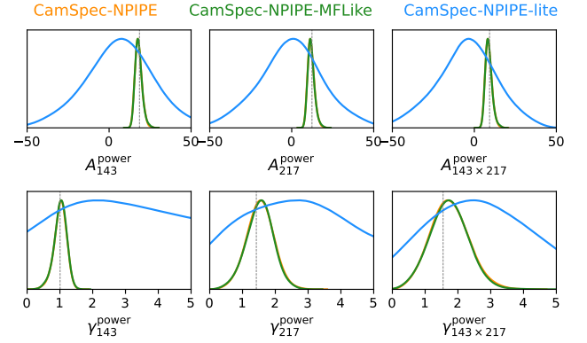
Figure 3. Posterior distributions of the foreground nuisance parameters from the multi-frequency likelihood (orange for the original CamSpec-NPIPE likelihood and green for our implementation in MFLike ), and from the foreground marginalization procedure (blue). Due to the fact that each foreground appears in only one spectrum each, they are fully degenerate in the foreground marginalization procedure, and thus highly unconstrained. Orange and green posteriors are obtained with a fit to the full Planck TT/TE/EE+lowT+lowE dataset but receive contribution only from the high- \ell CamSpec-NPIPE likelihood. The vertical lines indicate the best-fitting values from the CamSpec-NPIPE chain (original likelihood, shown in orange).
