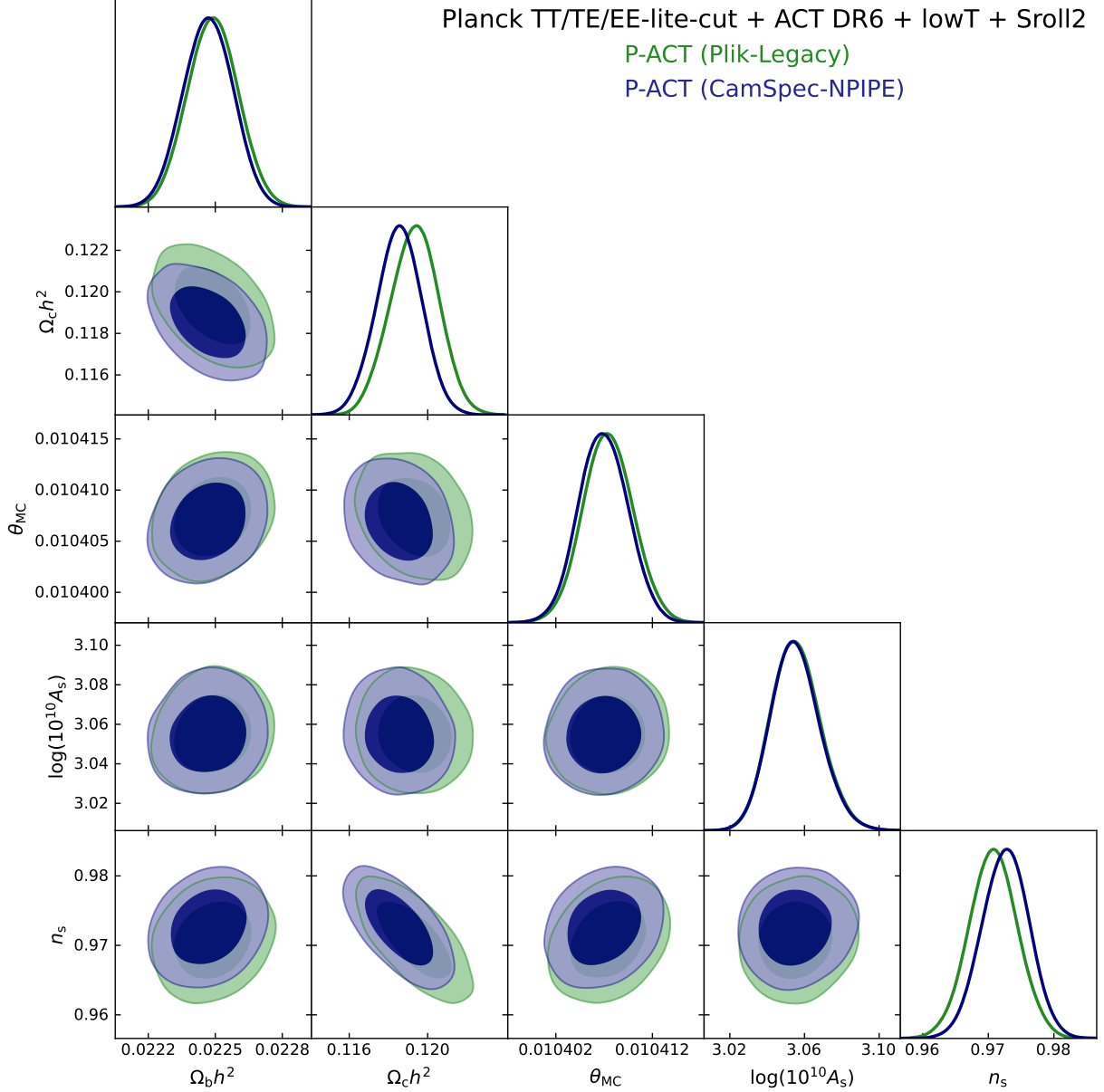
Figure 8. \Lambda CDM constraints from the P-ACT combination with either Plik-Legacy (green) or CamSpec-NPIPE (dark blue) in all five cosmological parameters. We find excellent agreement in between either choice in the P-ACT combination. Compared to Figure 7, we notice that there is less difference in most parameters.
