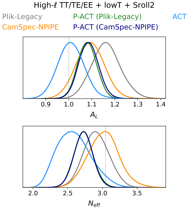
Figure 9. Comparisons of the ACT, Planck , and P-ACT constraints on A_L and N_{\text{eff}} for the Plik-Legacy and CamSpec-NPIPE likelihoods. In both cases, the P-ACT combination gives identical results for either Planck likelihood.
