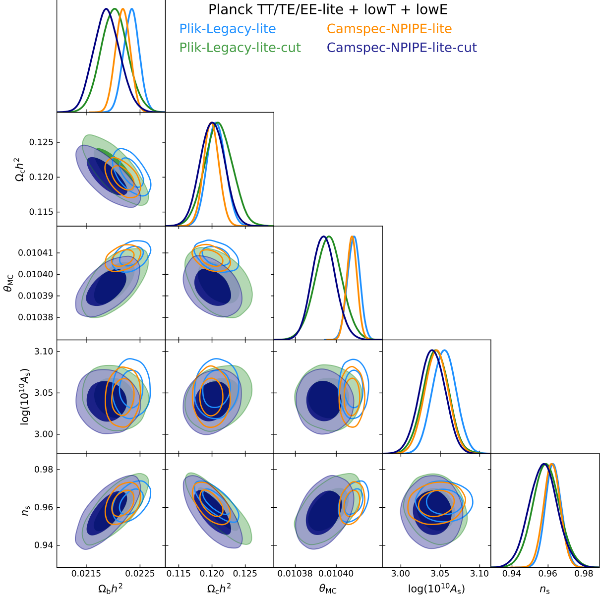
Figure 7. Comparison of \Lambda CDM parameters as obtained from Plik-Legacy and CamSpec-NPIPE likelihoods, using the full dataset (blue and orange respectively) and a restricted range keeping only the large scales with \ell < 1000/600/600 in TT/TE/EE (green and navy respectively). The results from the full datasets (open contours) do not overlap as much in parameter space as the cut likelihoods (filled contours).
