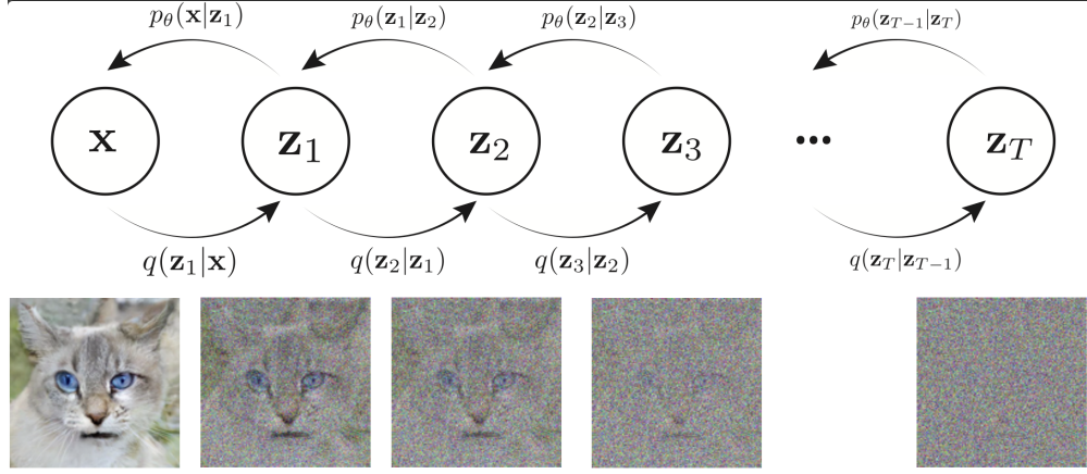
Figure 10: A variational diffusion model adds linear Gaussian noise at each time step, getting a fully Gaussian noise after T latent steps.
