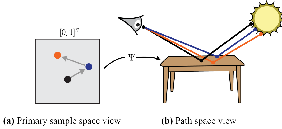
Figure 8: Primary Sample Space MLT performs mutations in an abstract random number space. A deterministic mapping \Psi induces corresponding mutations in path space.
