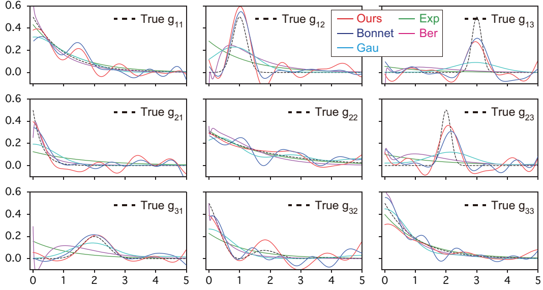
Figure A1: Examples of the estimated triggering kernels in the mutually-exciting scenario. Dashed lines represent the true triggering kernels.
