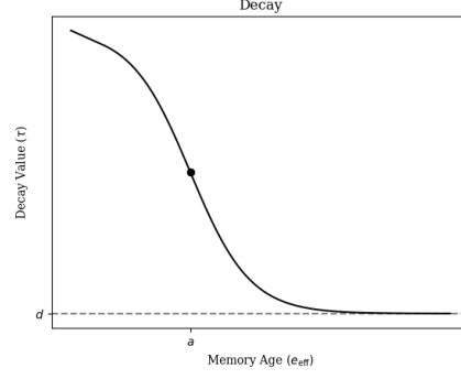
Figure 3: Graph of the decay function.
