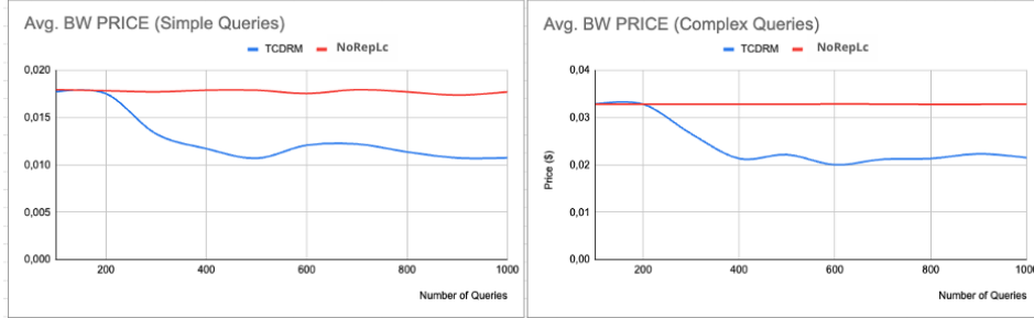
Fig. 5 : Bandwidth Cost per Query: Comparison of bandwidth consumption cost per query between NoRepLc and TCDRM for Simple and Complex Queries
