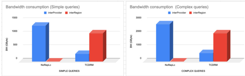
Fig. 4 : Bandwidth Consumption Comparison: Inter-rovider vs. interRegion bandwidth usage under TCDRM and NoRepLc.
