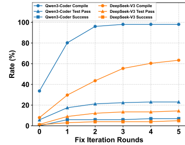
Figure 5: Performance evolution with compilation feedback.
