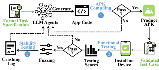
Figure 2: Workflow of APPFORGE.
