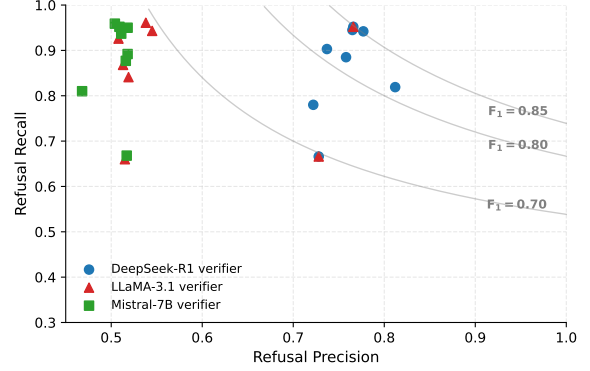
Figure 4: Verifier-swap ablation (Setting 2). Precision–recall trade-off on the Spider dataset.
