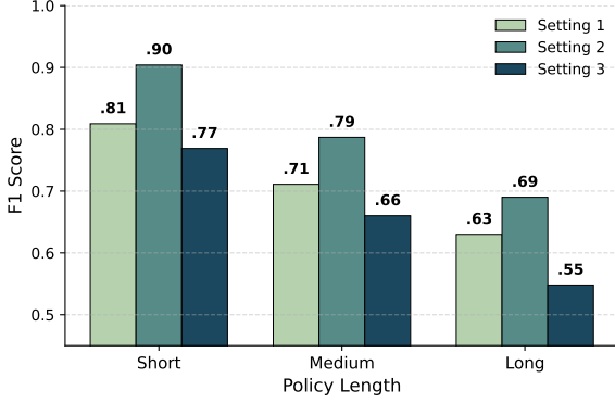
Figure 3: Effect of access-policy length on refusal performance (BIRD). Bars show average F_1 scores across three experimental settings: Setting 1 (GPT few-shot), Setting 2 (GPT→GPT zero-shot), and Setting 3 (fine-tuned Mistral).
