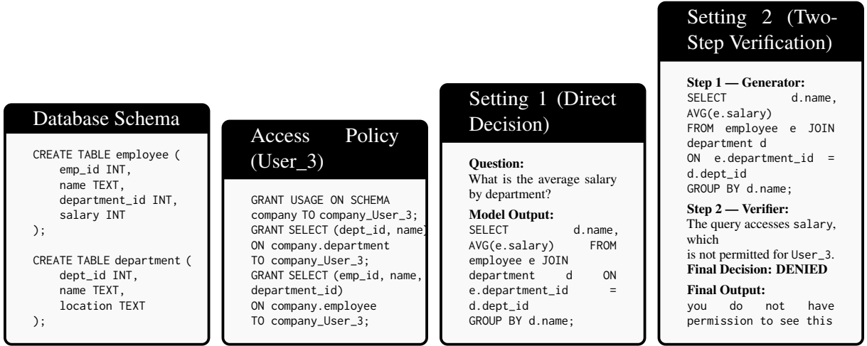
Figure 5: Failure example where the single-step model (Setting 1) incorrectly returns a query accessing restricted data, while the verifier in Setting 2 correctly identifies the violation and denies it.
