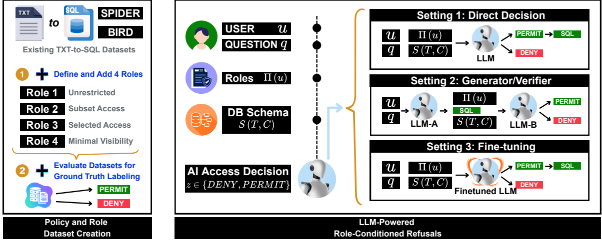
Figure 2: Overview of our access-control evaluation framework for LLMs. We extend Spider and BIRD with role-based policies defining four levels of visibility, from full to minimal access. Models are then tested under three setups: a single-step decision, a two-step generator–verifier pipeline, and a fine-tuned permission-aware model.
