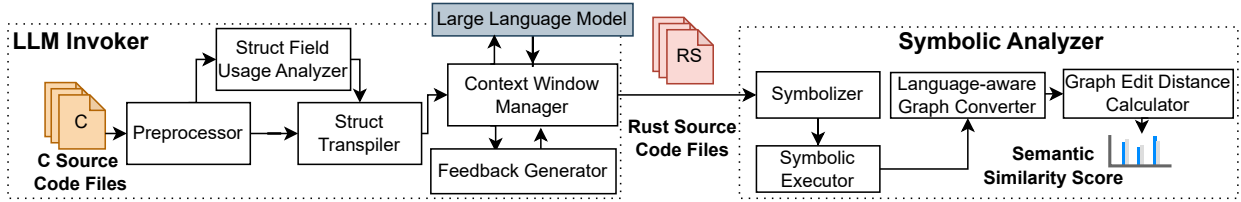
Fig. 2. RustAssure transpiler toolchain.
