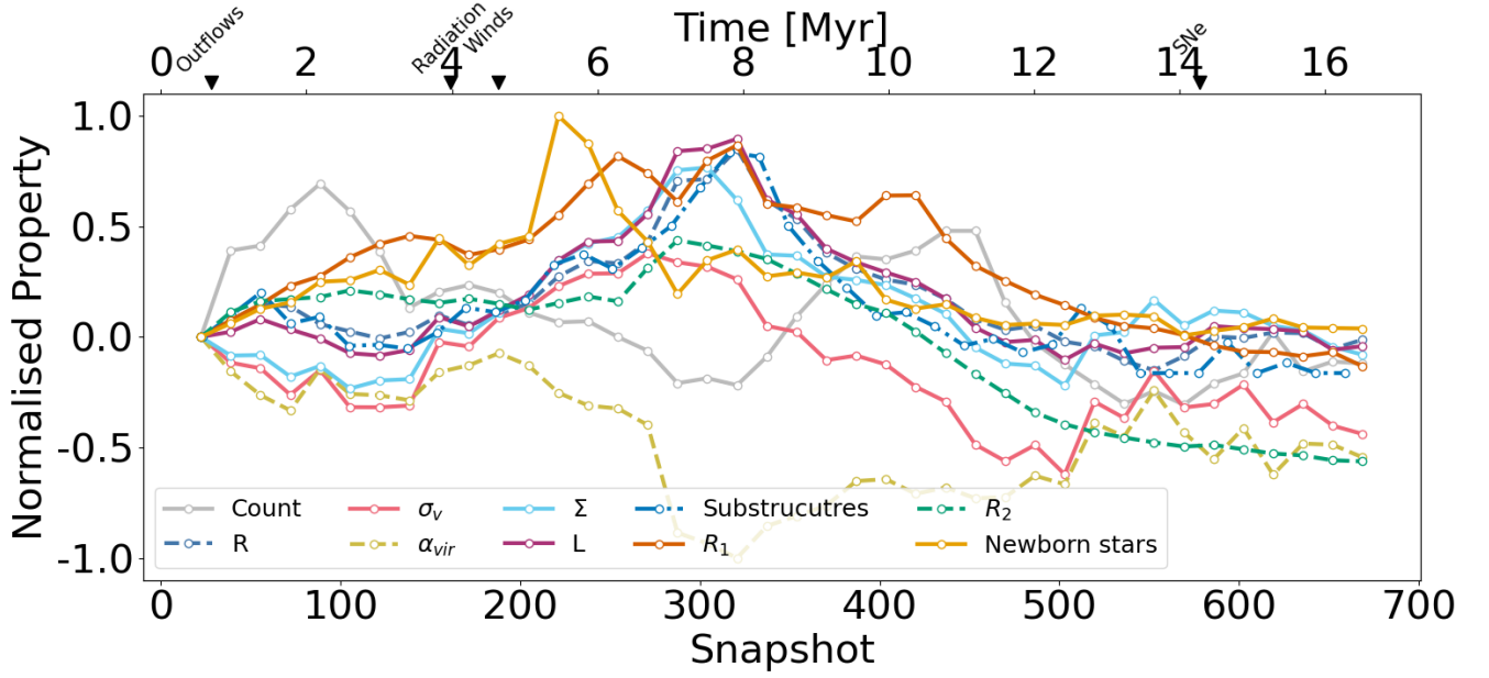
Fig. E.2. Simulation with \alpha_{vir} = 4 . Properties of the clouds at various evolutionary stages. The symbols and colors follow fig. E.1.
