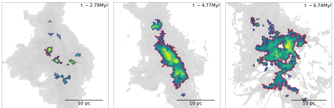
Fig. 4. ^{13}\text{CO}(2-1) moment 0 maps at different evolutionary time. The background greyscale represents \text{H}_2 gas density with ^{13}\text{CO}(2-1) emission overlaid as viridis maps (molecular gas complex), and coloured contours represent different MCs (dendrogram trunks), with red contours representing the largest MCs ( R ) in the cube. The ^{13}\text{CO}(2-1) maps for multiple snapshots along different projections are presented in App. B.
