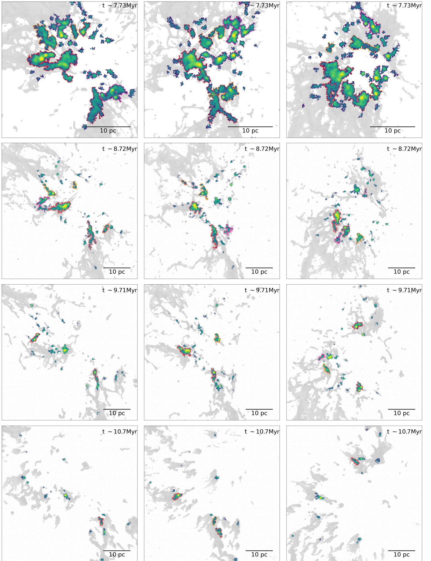
Fig. B.3. ^{13}\text{CO}(2-1) moment 0 maps for different snapshots. The colors and symbols follow fig. B.1.
