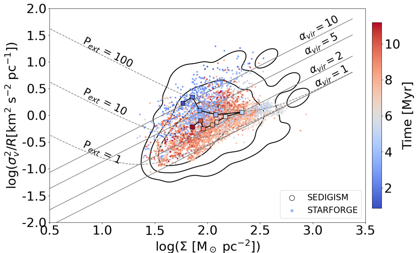
Fig. 9. Scaling relation between \sigma_v^2/R and surface mass density ( \Sigma ). The symbols and notations follow Fig. 8. The solid gray lines represent isocontours of virial parameters. The dashed lines represent \alpha_{\text{vir}} = 1 when including an external pressure P_{\text{ext}} = 1, 10, 100 \text{ M}_\odot \text{ pc}^{-3} \text{ km}^2 \text{ s}^{-2} .
