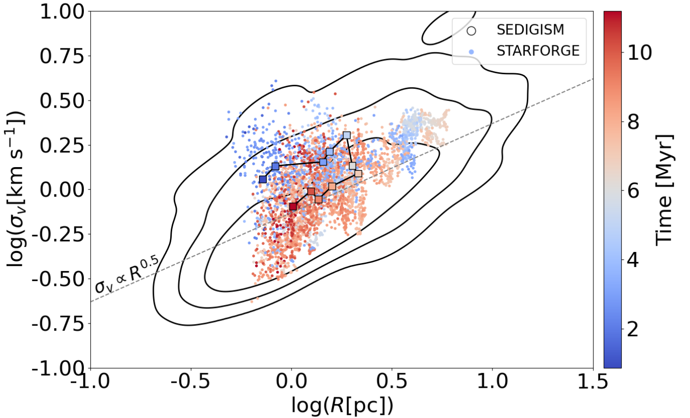
Fig. 8. Size-linewidth relation ( \sigma_v versus R ) for our MCs (scatter points), color coded with respect to the time elapsed (in Myr) since the start of the simulation. The squares represent medians of distributions in \sim 1 Myr bins. The black contours represent the 1\sigma , 2\sigma , 3\sigma levels for the SEDIGISM clouds. The dashed line represents Larson's first relation (Larson 1981; Solomon et al. 1987).
