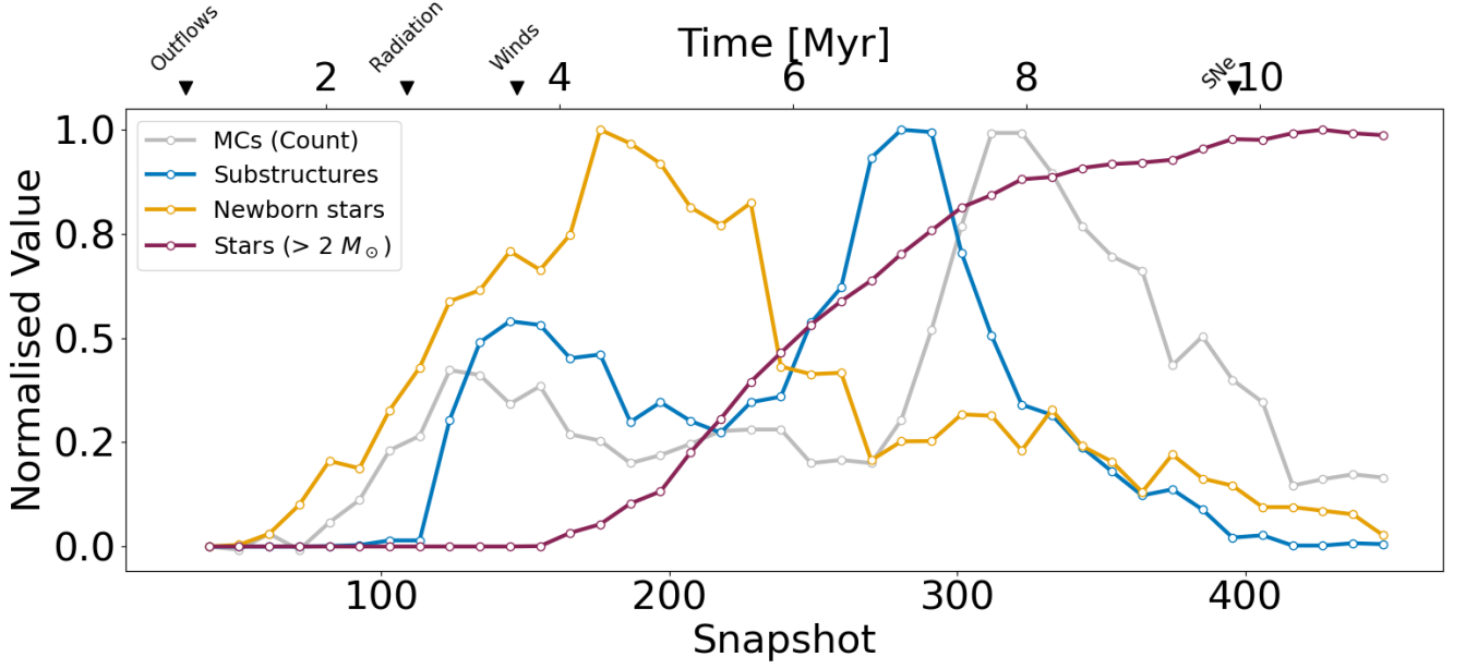
Fig. 7. Quantitative representation of MCs (counts), their substructures (dendrogram descendants), the newborn stars (age < 250 kyr), and the main sequence stars more massive than 2 M_{\odot} as a function of time. The values are normalised using a min-max standardisation.
