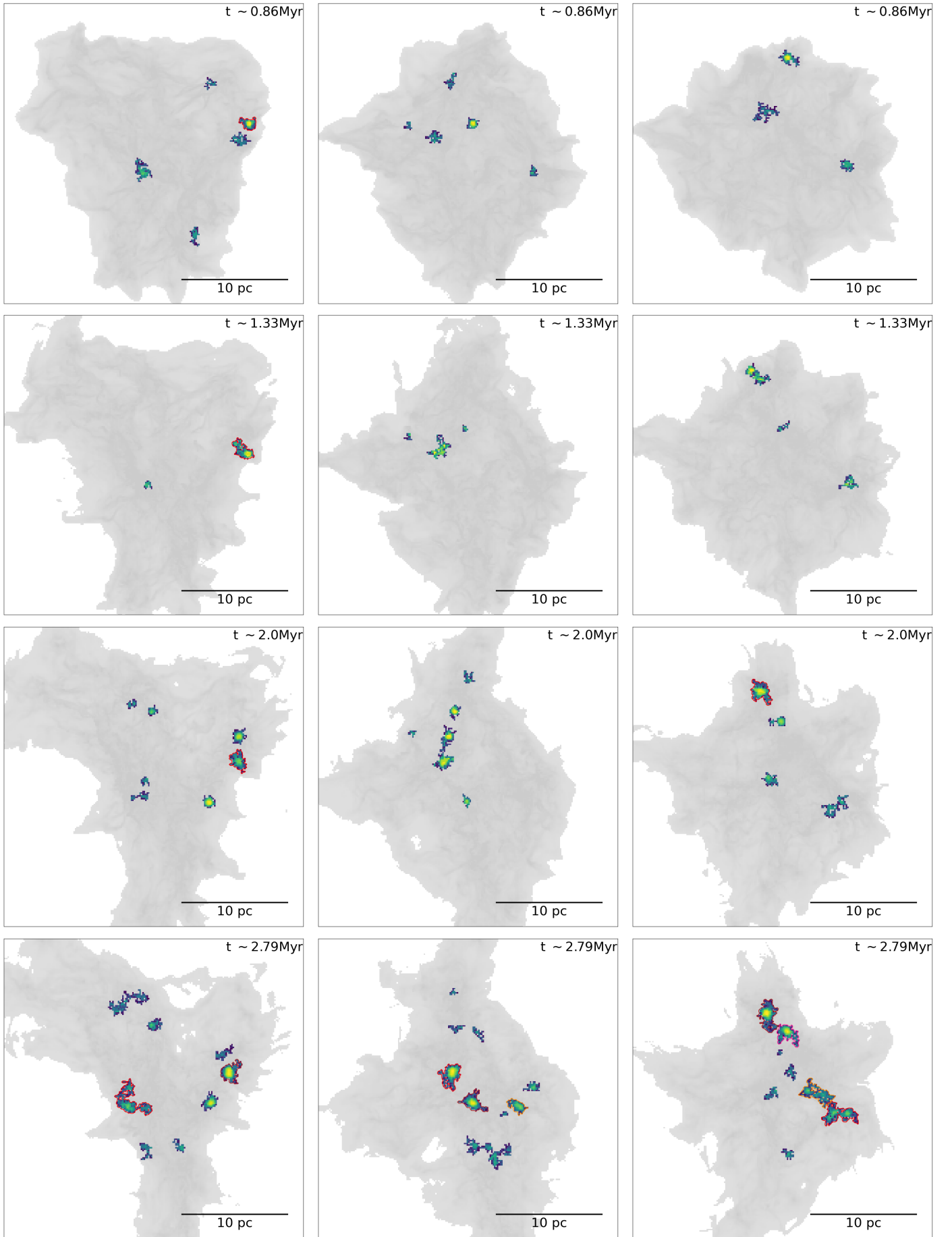
Fig. B.1. ^{13}\text{CO}(2-1) moment 0 maps for different snapshots. The three columns represent the clouds projected along the x, y and z axes, respectively. The background greyscale represents \text{H}_2 gas density with ^{13}\text{CO}(2-1) emission overlaid as viridis maps, and coloured contours represent different MCs (dendrogram trunks), with red contours representing the largest MCs ( R ) in the cube.
