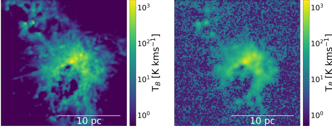
Fig. 1. Left: A synthetic integrated ^{13}\text{CO}(2-1) emission map created with RADMC-3D. Right: The same map after convolution and with noise of \sigma = 0.2 \pm 0.02 K.
