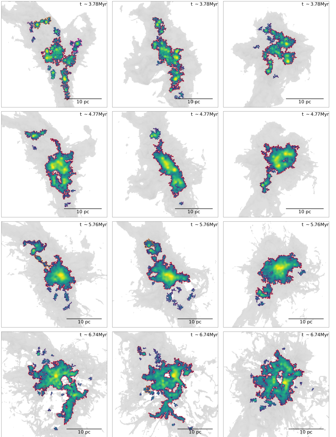
Fig. B.2. ^{13}\text{CO}(2-1) moment 0 maps for different snapshots. The colors and symbols follow fig. B.1.
