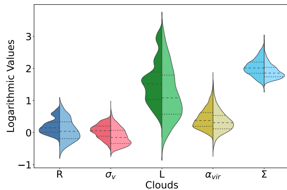
Fig. 3. Comparison of MC properties from STARFORGE (left side violins) and SEDIGISM (right side violins). The properties are radius (R), velocity dispersion ( \sigma_v ), luminosity (L), virial parameter ( \alpha_{vir} ) and surface density ( \Sigma ). The horizontal dashed lines represent the quartiles of the distributions.
