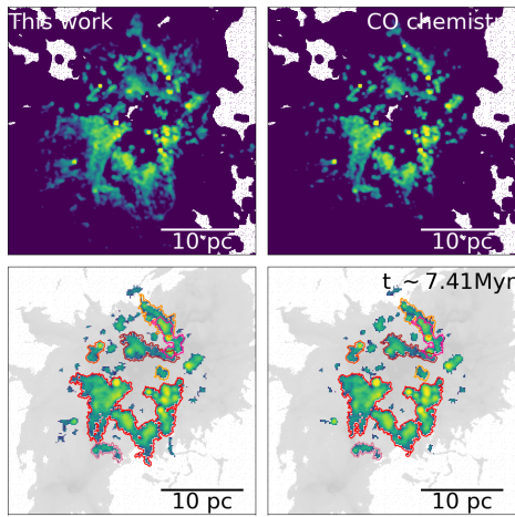
Fig. C.3. Comparison between the ^{13}\text{CO}(2-1) ppv cube used in this work and created by including CO chemistry for snapshot 300 (7.41 Myr). The symbols and notations follow Fig. C.1.
