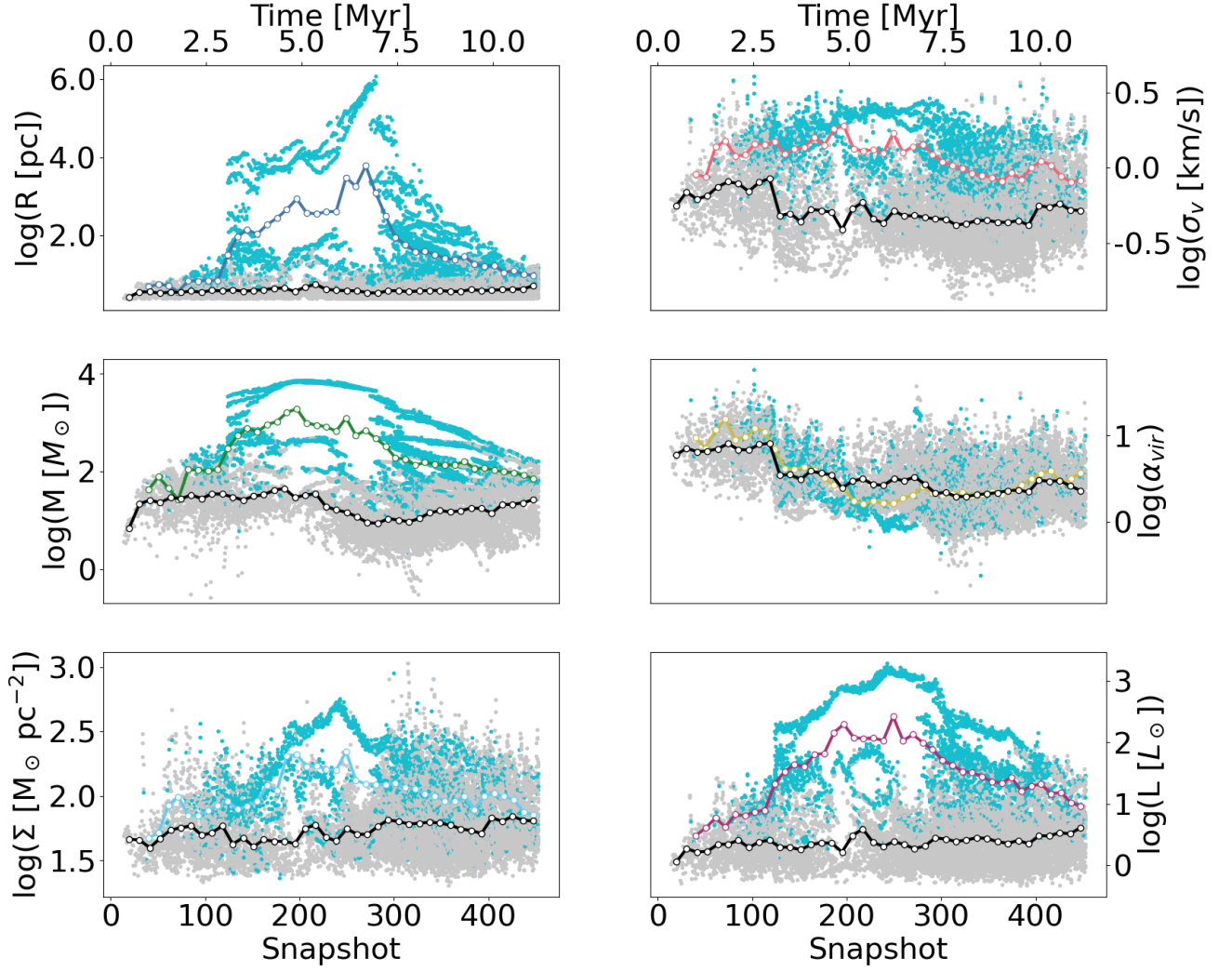
Fig. D.1. The cyan points represents the hierarchical trunks (branches) and grey points represents the isolated trunks (leaves). The colored lines represents the average distribution of hierarchical trunks, with the colors following Fig. 5. The black line represents the average distribution for isolated trunks.
