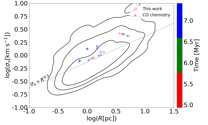
Fig. C.4. Size-linewidth relation ( \sigma_v versus R ) for our MCs (circles) and those created by including CO chemistry (plus). The MCs have been extracted from three ppv cubes in Fig. C.1 - C.3. The symbols and notations are consistent with Fig. 8.
