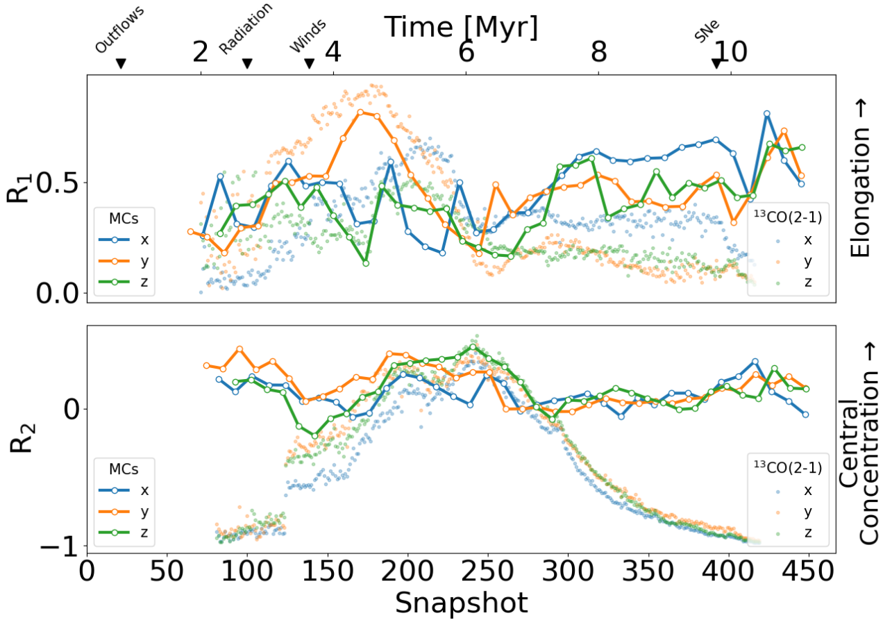
Fig. 6. Morphological analysis of the MCs (solid line) and molecular gas complexes (points) in different snapshots. R_1 represents the degree of elongation and R_2 represents the degree of central concentration. The lines represent the R_1 and R_2 values for the MCs, and the scatter points represent the same for the molecular gas complexes (entire ^{13}\text{CO}(2-1) emission in snapshot) obtained using the projections along the three axes. The color scheme is the same as in Fig. 3.
