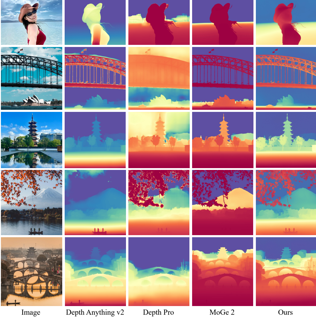
Figure 4: Comparison with existing depth foundation models on open-world images. Our model preserves more fine-grained details than Depth Anything v2 [82] and MoGe 2 [70], while demonstrating significantly higher robustness compared to Depth Pro [4].
