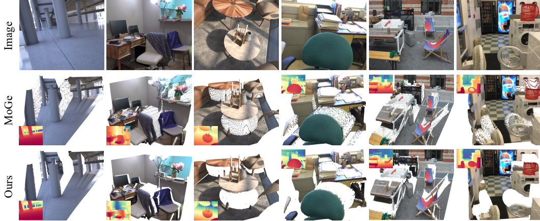
Figure 7: Qualitative comparisons with MoGe [69]. Top: input images are taken from four test sets: Hypersim [50], DIODE [63], ScanNet [11], and ETH3D [56]. Middle: results of MoGe [69]. Bottom: our results. As a discriminative model, MoGe [69], like other discriminative models [82, 4], also suffers from flying pixels at edges and details.
