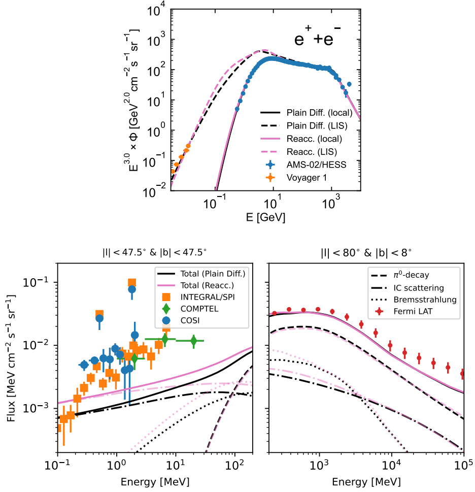
Fig. 2 Upper panel: Comparison of the locally observed primary CR electron + positron spectra by AMS-02 [42] and HESS [43] and the spectrum observed by Voyager-1 in interstellar space [44] (denoted as “LIS” in panel legend) to expectations from two different models of CR propagation. Both models were computed with GALPROP [34], assuming plain diffusion + convection of CR in the ISM in one case (black), and diffusion with re-acceleration of CR in the ISM (pink) in the other case. Lower panel: Expected DGE emission in the MeV and GeV bands from the two CR propagation models shown in the upper panel. The expected emission (black/pink solid lines) is compared to the MeV observations displayed in Figure 1, and to the measurement of the diffuse emission by Fermi LAT in [26] (red bars, right panel). Fermi -LAT measurements have been published for a different region of the sky than the MeV measurements in the left panel. The corresponding region is indicated above the respective panel. Individual contributions from various interaction processes are shown as dashed/dotted lines (see legend).
