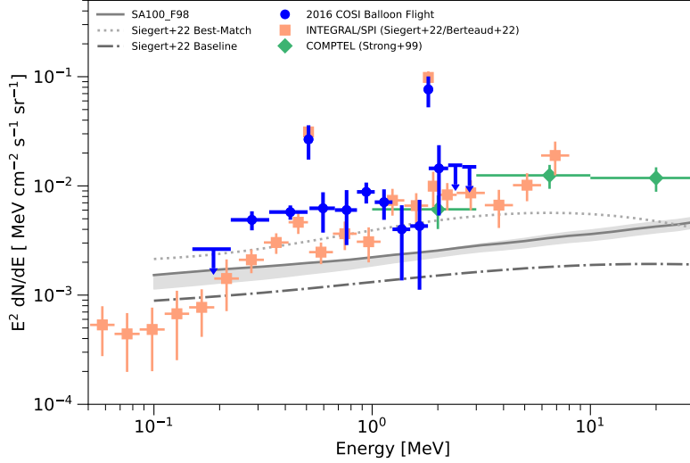
Fig. 1 Measurements of the DGE in the direction of the inner Galaxy during the 2016 COSI balloon flight [30], by COMPTEL [27, 31], and SPI [32, 33] in comparison to expectations [32, 34]. The models do not include line emission visible in the data at 511 keV ( e^+/e^- annihilation) and 1.81 MeV ( ^{26}\text{Al} decay). Figure adapted from [30].
