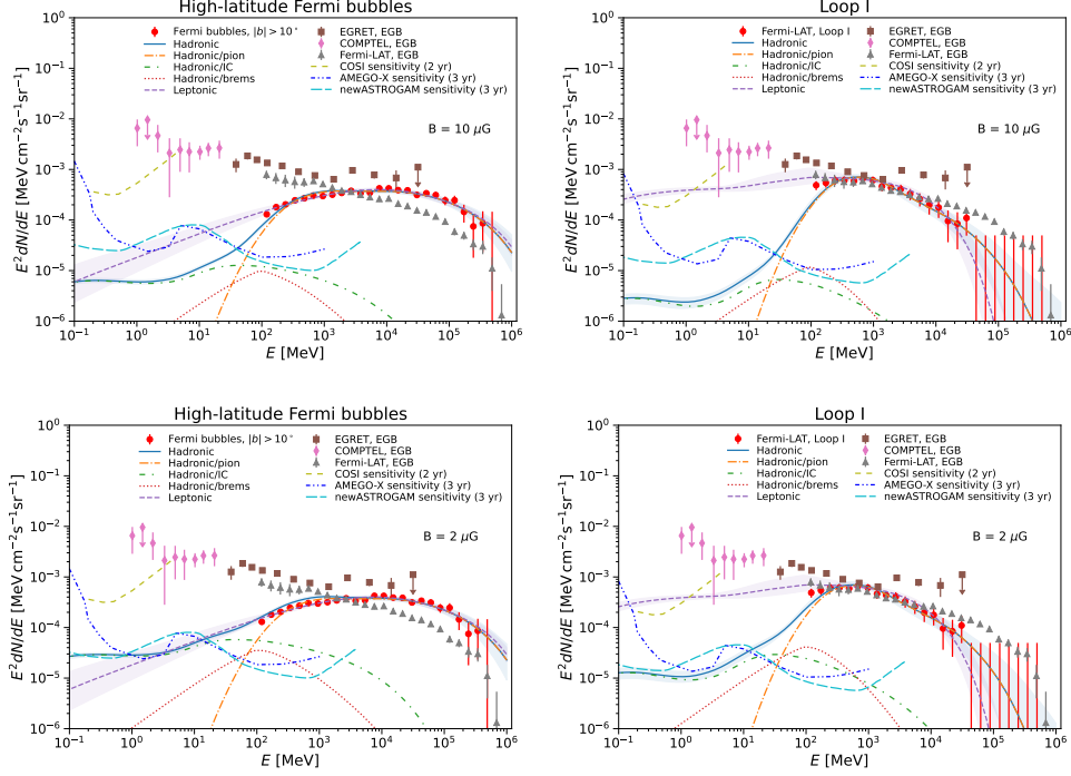
Fig. 3 Intensity of emission of the FBs (red circles, left panel) and Loop I (red circles, right panel) at latitudes |b| > 10^\circ [59]. Blue solid line shows the hadronic model of the \gamma -ray emission. Dashed orange line, green sparse dash-dotted line, and dotted red line show the primary \pi^0 , secondary IC, and secondary bremsstrahlung components in the hadronic scenario respectively. Dashed purple line - leptonic scenario of \gamma -ray emission (dominated by IC emission). Bands show the 1 sigma model uncertainty ranges for statistical plus 10% systematic uncertainties in the data. Pink diamonds, brown squares, and grey upward triangles show the extragalactic diffuse \gamma -ray background measured by COMPTEL [93], EGRET [94], and Fermi LAT [22] respectively. Yellow sparse dashed lines show expected COSI sensitivity after 2 years of observations [56] for an extended source with the area of the high-latitude FBs \Omega \approx 1 sr and Loop I \Omega \approx 3 sr respectively. Expected AMEGO-X [54] and newASTROGAM [53] sensitivities for high-latitude FBs and Loop I after 3 years of observations are shown by blue dash-dot-dotted and cyan long-dashed lines respectively.
