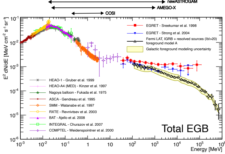
Fig. 4 Measurements of the extragalactic X-ray and \gamma -ray background from 1 keV to 820 GeV. The energy ranges of the upcoming COSI satellite and other proposed future \gamma -ray space missions are indicated by the arrows above the figure. Figure adapted from [22].
