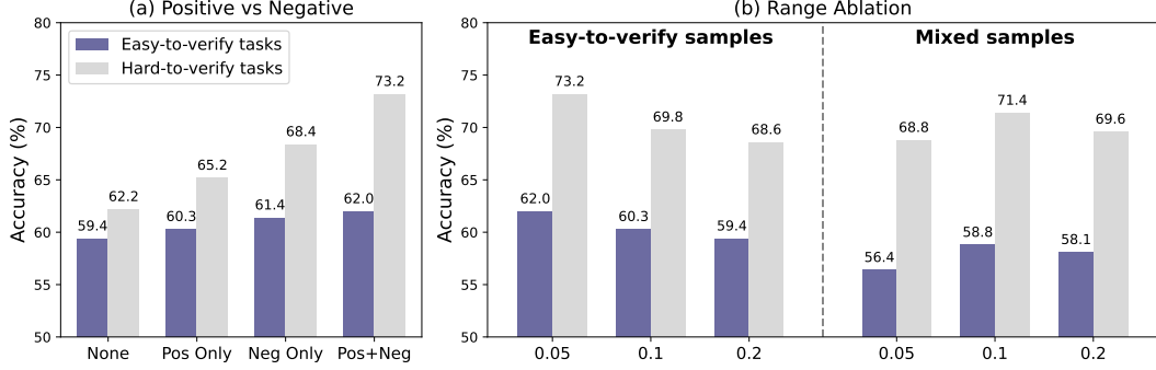
(a) Impact of using positive and negative dense ranges. Dense negative rewards contribute more to stable learning than positive samples. (b) Effect of varying reward ranges under different training regimes. Smaller ranges perform best on verifiable tasks, while larger ranges benefit mixed settings by providing denser feedback.
