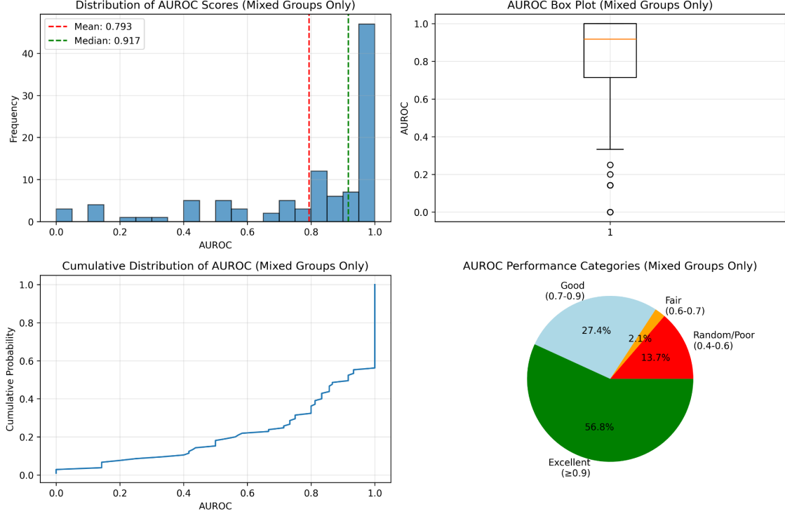
Reward model qualification ability on mixed groups: (a) distribution of AUROC scores, (b) AUROC box plot, (c) cumulative distribution of AUROC, and (d) AUROC performance categories.
