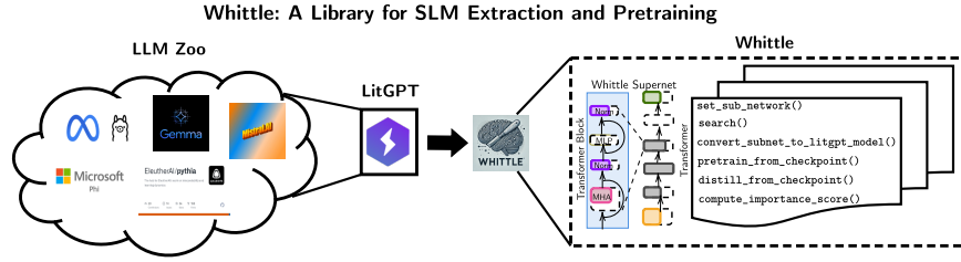
Figure 9: An overview of the Whittle library.
