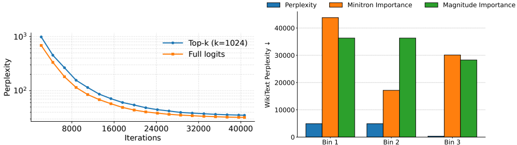
Figure 7: Full vs. top- k logit distillation.
