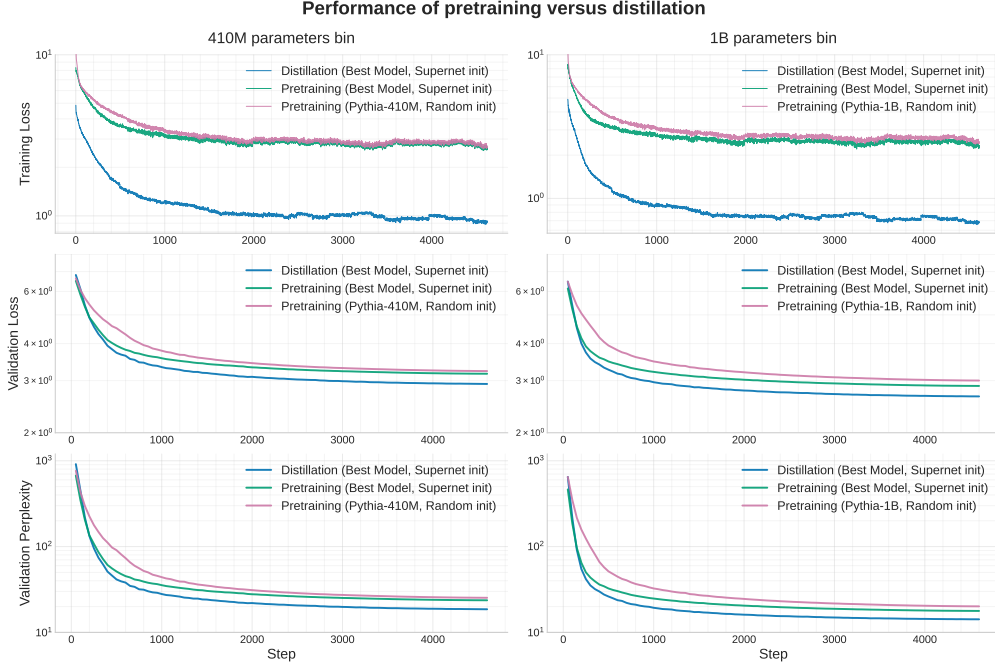
Figure 16: Training curves of the best models in bins 1 and 2, obtained through distillation and pretraining. In both cases, the models are initialized with weights from the supernet (Pythia-6.9B). For comparison, a Pythia model of similar size is trained from random initialization in both bins, serving as a baseline. All models are trained on 10 billion tokens.
