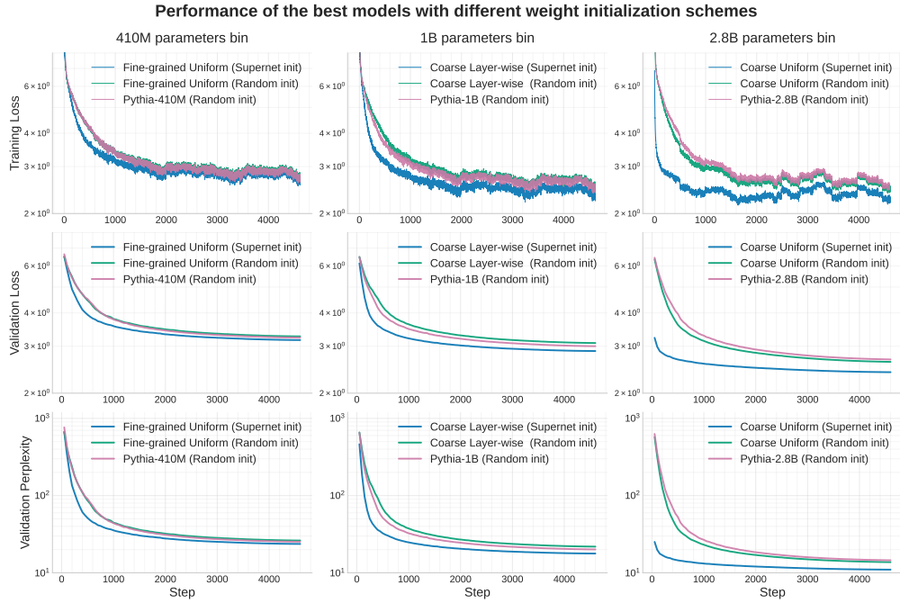
Figure 15: Training curves of the best models found in each bin, initialized with supernet weights as well as random weights. A Pythia model of comparable size is also trained with random initialization in each bin as a baseline. The models are trained with 10 billion tokens.
