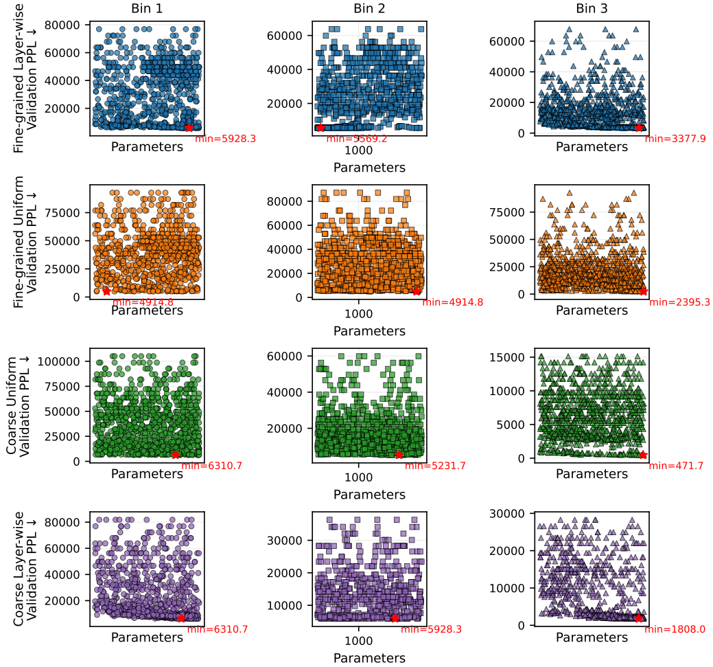
Figure 13: Evolutionary search on coarse uniform , coarse layer-wise , fine-grained uniform and fine-grained layer-wise search spaces for Pythia-6.9B. Minimum perplexity for each bin marked in red
