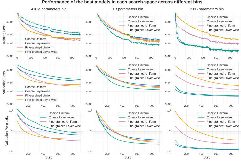
Figure 14: Training curves of the best models from each search space extracted from Pythia-6.9B (trained for 2 billion tokens)
