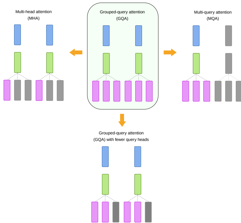
Figure 11: An example of how grouped-query attention (GQA) can be masked to emulate other forms of attention, such as multi-head or multi-query attention. The masked heads are shown in gray. Note that GQA can also be reduced to fewer query heads while preserving the same number of groups.
