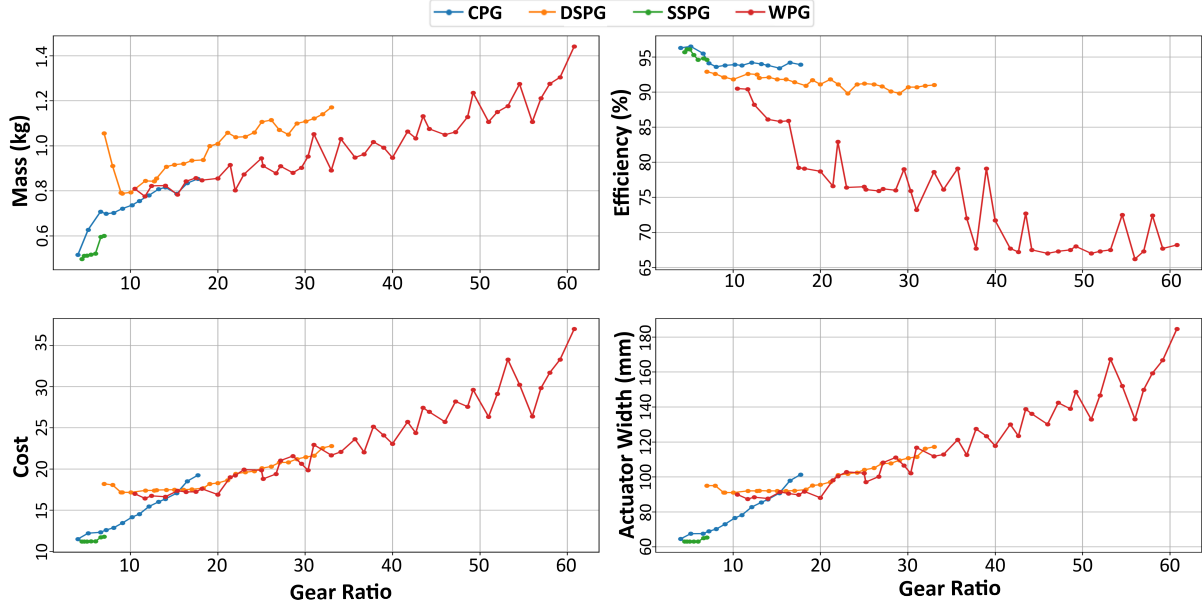
Fig. 6: Optimization results for gearbox ratios between 4:1–60:1 with the MAD-M6C12 motor. Mass, efficiency, width, and cost are plotted against gear ratio to identify the optimal gearbox type for a given motor.
