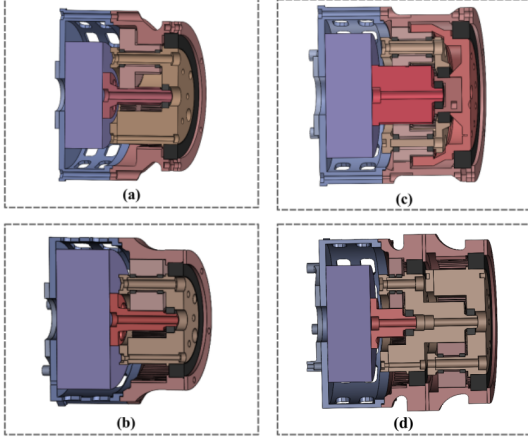
Fig. 3: 3D CAD models of the actuators (Red: gear assembly , Blue: motor assembly ). (a) CPG : 14:1, Motor: MAD-M6C12; (b) SSPG : 7.2:1, Motor: T-motor MN8014; (c) WPG : 16.36:1, Motor: MAD-M6C12; (d) DSPG : 22.05:1, Motor: MAD-M6C12. Refer Table I for specifications.
