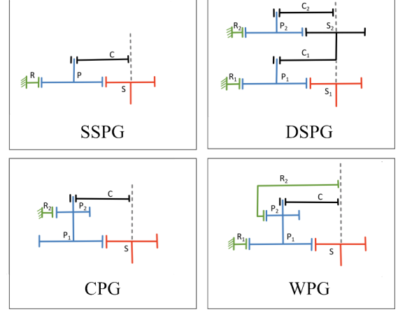
Fig. 2: Line diagrams of planetary gearbox configurations. SSPG: Sun ( S ) input, Ring ( R ) fixed, Carrier ( C ) output. CPG: Sun ( S ) input, Ring ( R_2 ) fixed, Carrier ( C ) output; planets ( P_1, P_2 ) rigidly attached. DSPG: Sun ( S_1 ) input, Rings ( R_1, R_2 ) fixed, Carrier ( C_2 ) output; S_2 and C_1 rigidly attached. WPG (3K): Sun ( S ) input, Ring ( R_1 ) fixed, Ring ( R_2 ) output; planets ( P_1, P_2 ) rigidly attached.
