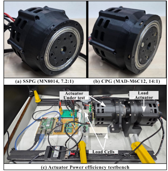
Fig. 4: (a) Assembled SSPG actuator, (b) Assembled CPG actuator, (c) Power efficiency testbench: two load cells measure the torque of the actuator under test, while a second actuator serves as the load.
