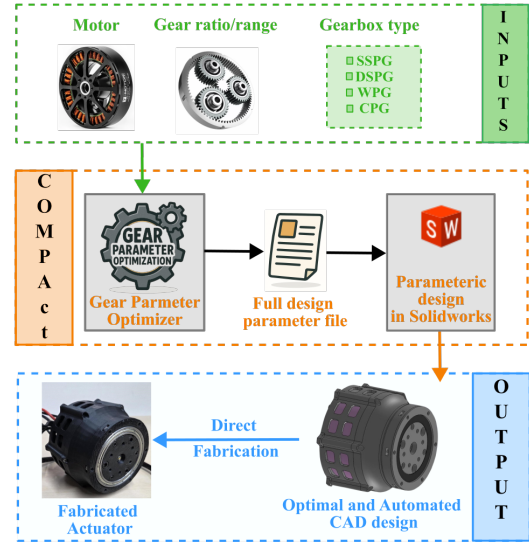
Fig. 1: COMPAct: Framework for optimal design and automated CAD generation of planetary robotic actuators.
