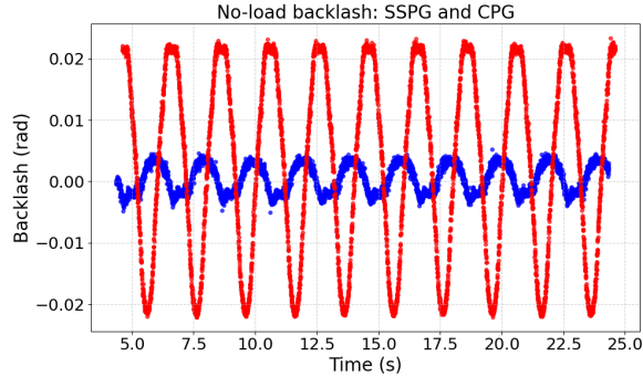
Fig. 8: No-load backlash test results. The compound planetary gearbox (CPG, red) exhibits a backlash of 0.046 rad ( 2.6^\circ ), whereas the single-stage planetary gearbox (SSPG, blue) shows a lower backlash of 0.010 rad ( 0.59^\circ )
