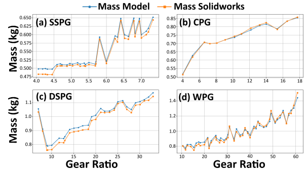
Fig. 5: Comparison of mass model predictions with 3D CAD estimates. The model closely matches the final CAD masses, with RMS errors of 0.01 kg (SSPG), 0.005 kg (CPG), 0.024 kg (DSPG), and 0.028 kg (WPG).
