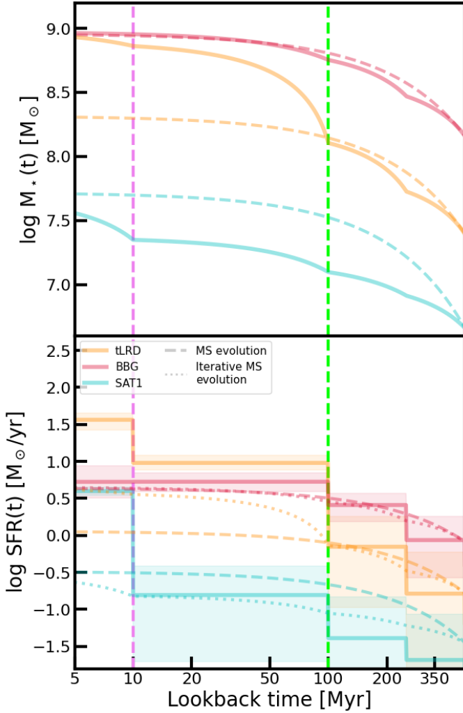
Fig. 8: Top: mass assembly histories of tLRD (solid orange), BBG (solid red), and SAT1 (solid cyan) on log scale. We also show the mass growth of these galaxies, assuming that they followed the main sequence (dashed lines, in the same color code). To calculate these MS tracks, we used the main sequence fit from Mérida et al. (2025b) at 5 < z \leq 7 and the M_* of the sources at t = 500 Myr. We assumed a return fraction of 0.3. Vertical lines highlight t = 10 Myr (violet) and t = 100 Myr (lime), respectively. Bottom: SFHs of our sources, following the same color code. SFHs of analogous galaxies evolving along the main sequence since t = 500 Myr ago are also depicted. Additionally, we show the MS evolution resetting this seed mass to that achieved in each time bin (dotted lines). The shaded region shows the SFH uncertainty of each source. Additionally, we should take into account the main sequence scatter, which is \sim 0.2 dex at this z .
