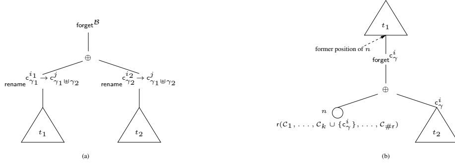
■ Figure 5 The \text{join}(t_1, t_2, c_{\gamma_1}^{i_1}, c_{\gamma_2}^{i_2}) (a) and \text{append}(t_1, t_2, n, k, c_\gamma^i) (b) operations
