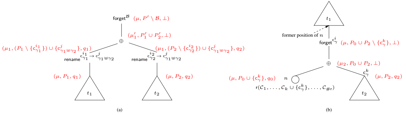
■ Figure 6 The implementation of the \text{join}(t_1, t_2, c_{\gamma_1}^{i_1}, c_{\gamma_2}^{i_2}) (a) and \text{append}(t_1, t_2, n, k, c_{\gamma}^i) (b) operations in \mathcal{A}^* , where the states of \mathcal{A}^* are depicted in red.
