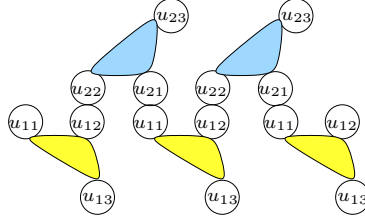
■ Figure 4 Fusion of G structures by 3-generated matchings
