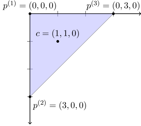
Figure 1: The polygon in the reduction for d = 3 .
