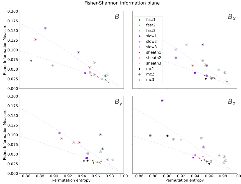
Figure 4. A zoomed-in section of the Fisher-Shannon plane. The top dotted curve is the fBm curve with r = 300 , and the lower curve is the fBm curve with r = 20 .
