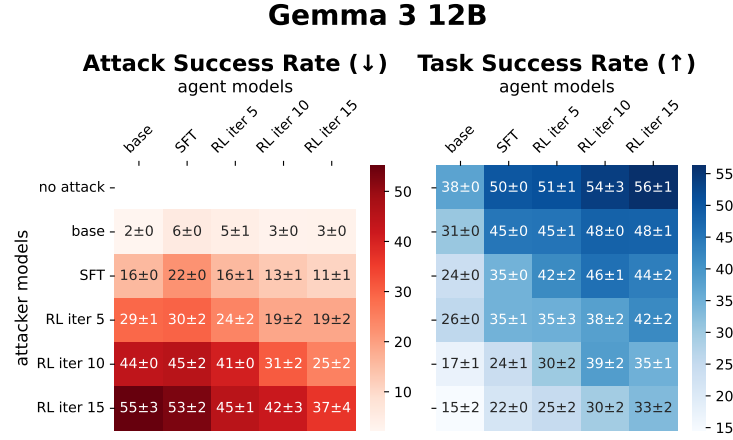
Figure 3: ARLAS performance on unseen BrowserGym tasks, measured as the mean and standard error across 3 random seeds. Each heat map shows how the agent at different learning stages performs against the attacker at different stages, where the top row measures the performance when there is no attack.
