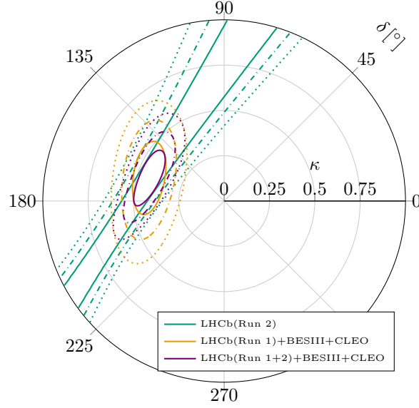
Figure 5: Profile likelihood of \kappa vs. \delta , inclusive over the entire phase space. The \Delta\chi^2 = 2.38, 6.18, 11.83 contours are indicated, corresponding to the 68.7, 95.0, 99.7% confidence intervals for a Gaussian likelihood.
