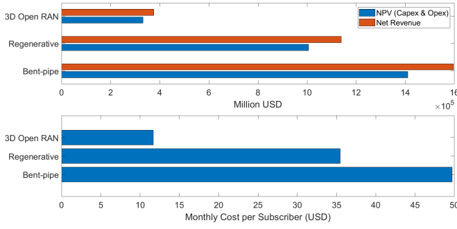
Fig. 12. Economic assessment for System B (2800 beams; 10 MHz).
