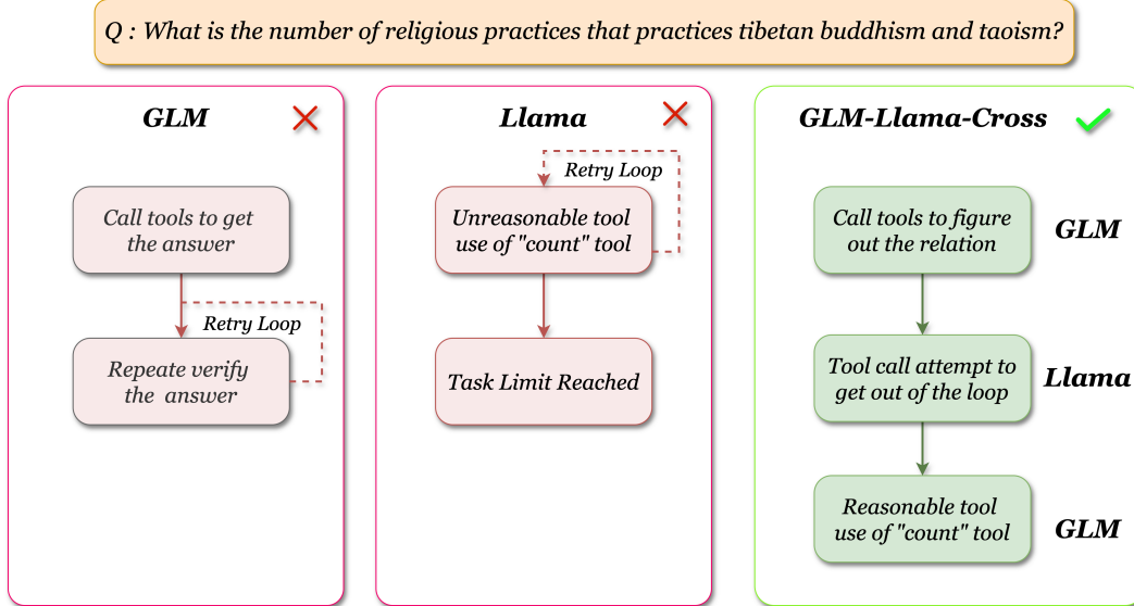
Figure 9: An example of GLM, Llama and GLM-Llama cross sampling in a KG task. This case study demonstrates the Cross-Policy Sampling strategy’s success on a KG question-answering task, where GLM-4 fails in a conclusion loop and Llama falters with tool comprehension. It combines GLM-4’s logic with Llama’s tool interaction to achieve the correct answer.
