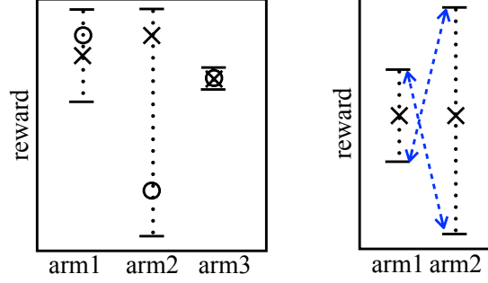
Figure 3: Uncertainty in Multi-armed bandits (MABs). “O” is true mean and “X” is point estimate. Left: Example where greedy w.r.t. point estimate chooses arm2 and suffers large loss. Instead, pessimism chooses arm3 with suboptimality bounded by the uncertainty of the best arm (arm1). Right: Example where return optimization chooses a different pessimistic policy (arm1) than regret minimization. Both arms have the same regret (height of double-headed arrows), and randomizing between them only incurs half of the regret.
