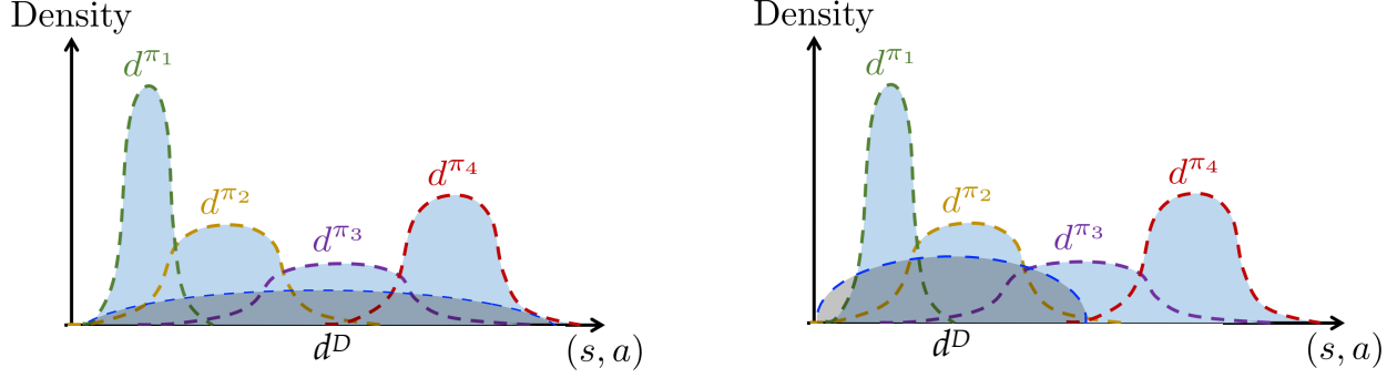
Figure 2: Figurative illustration of different coverage assumptions, adapted from Xie et al. (2023). Left: All-policy coverage. Right: Data only covers \pi_1 and \pi_2 , and pessimistic algorithms in Section 4.1 can compete with the best among them.
