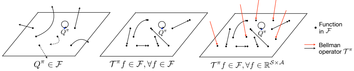
Figure 1: Figurative illustration of different expressivity assumptions on the value-function class \mathcal{F} . Left: Only realizability Q^\pi \in \mathcal{F} is assumed, and Bellman operator (“ \rightarrow ”) can generally take functions in \mathcal{F} out of the class. Middle: Bellman-completeness, where \mathcal{F} is closed under \mathcal{T}^\pi . Right: All functions, including those not in \mathcal{F} , have their image in \mathcal{F} (Section 4.5).
