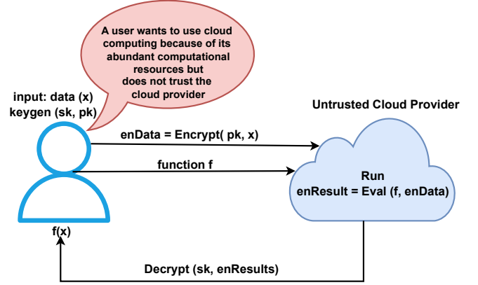
Fig. 1: A HE outsourced cloud computation scenario showing a user who encrypts data and evaluates a function in the cloud. The encrypted results are sent back to the user, who decrypts them to get the evaluated results.
