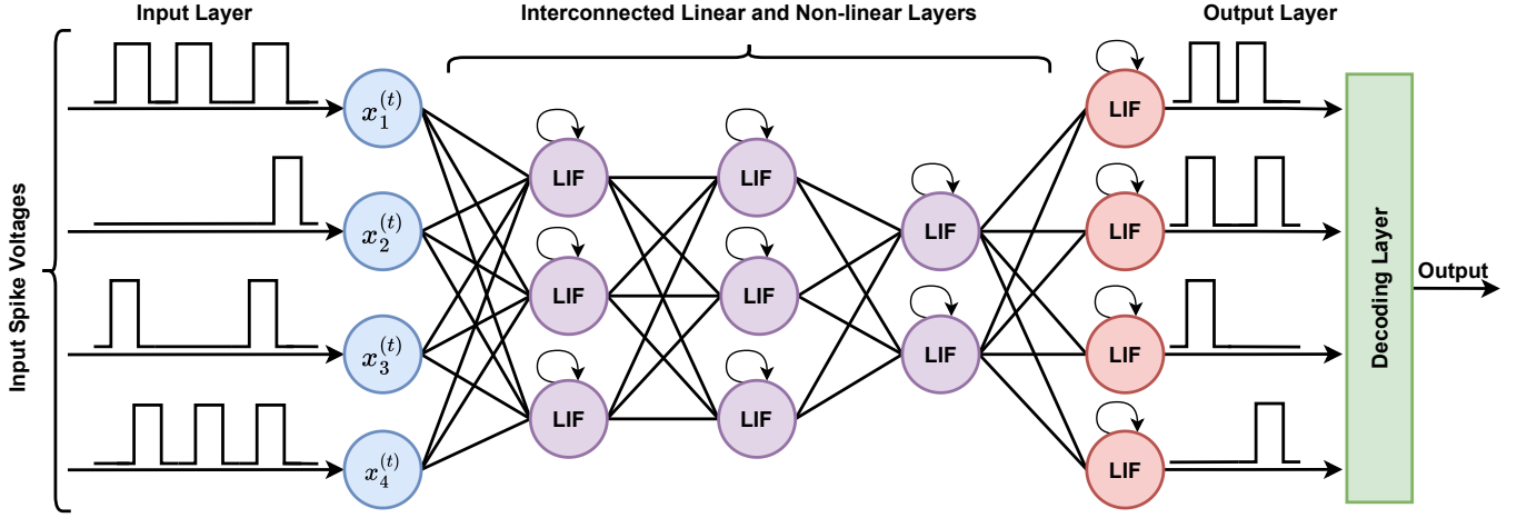
Fig. 2: Overview of a spiking neural network. Spikes are input across discrete time steps and propagated through linear and non-linear layers. Linear layers extract spatial features, while non-linear spiking dynamics capture temporal dependencies via recurrent processing. The output layer accumulates spikes over time and decodes them into a prediction.
