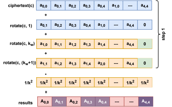
Fig. 5: Vector Encoding Secure Average Pooling: These rotations are then summed and multiplied by 1/k^2
