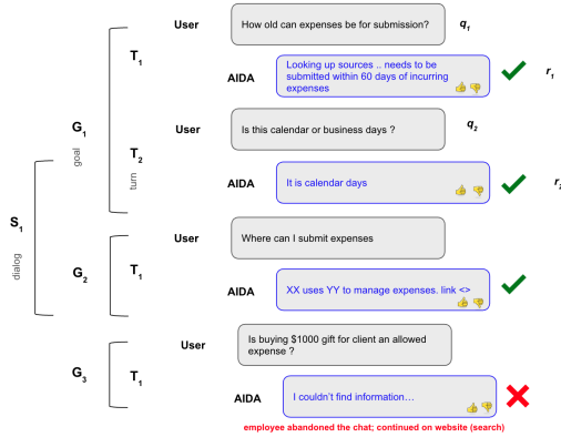
Figure 3: Anatomy of a chatbot session: Each dialog consists of multiple goals ( G_i ), where each goal comprises one or more turns ( T_j ), formed by a query-response pair ( q_j, r_j ). Goal G_3 is marked failed due to information unavailability.
