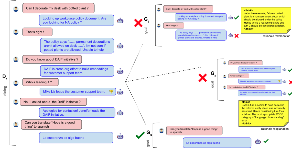
Figure 2: Goal-oriented breakdown of a multi-turn employee chatbot conversation. The full dialog (left) is segmented into three distinct goals: G_1 (policy inquiry), G_2 (project clarification), and G_3 (translation request). Each goal is independently evaluated for success or failure using goal-level metrics. Turn-level evaluation may suggest high success, but goal-level evaluation reveals that G_1 and G_2 failed due to reasoning and language understanding errors, respectively. Root Cause of Failure (RCOF) is annotated using structured rationale snippets (right), highlighting the earliest defective turn per goal.
