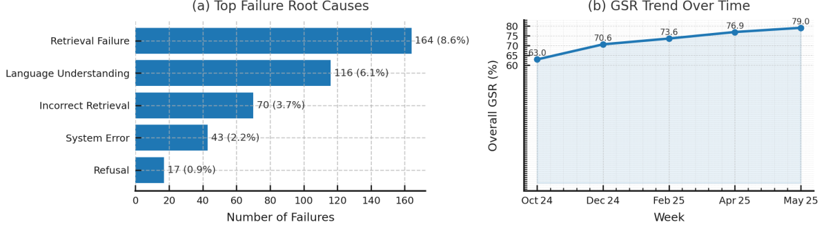
Figure 4: (a) Distribution of the top five chatbot failure root causes, annotated with both absolute counts and percentages. (b) Trend of the overall Goal-Success Rate (GSR) from Oct '24 through May '25, showing a steady improvement.
