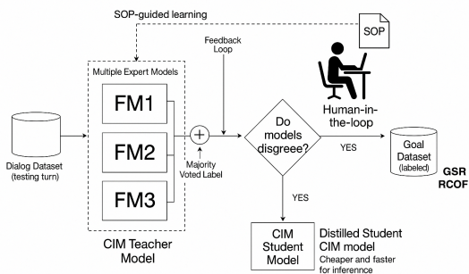
Figure 5: HITL evaluation pipeline: AIDA conversations are processed by multiple expert models using Chain-of-Thought prompts. Majority-voted outputs are accepted as labels. Disagreements are escalated to human experts guided by SOPs.
