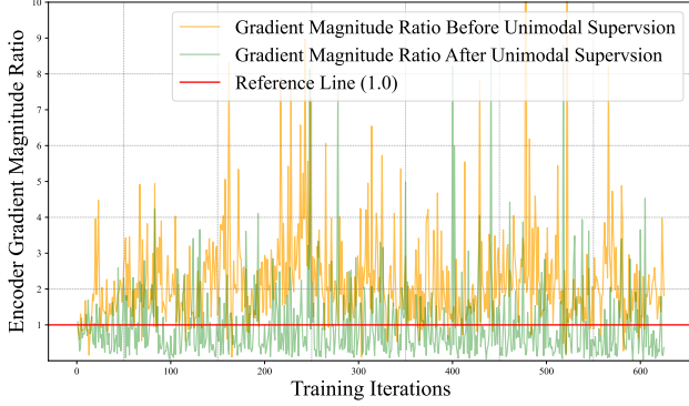
Fig. 3. Gradient magnitude ratio between RGB encoder and thermal encoder.
