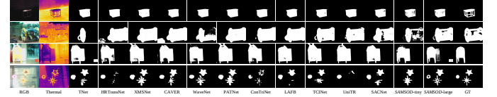
Fig. 8. Failure cases involving hollow objects (1 st and 2 nd rows) and local overexposure scenes (3 rd and 4 th rows).
