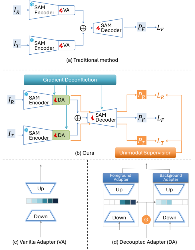
Fig. 1. The framework comparison between traditional methods and ours and their adapters.
