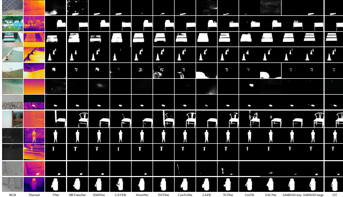
Fig. 7. Qualitative comparisons of visualization in complex background (1 st and 2 nd rows), multiple objects (3 rd and 4 th rows), small objects (5 th and 6 th rows), fine-grained objects (7 th and 8 th rows), objects in low light environment (9 th and 10 th rows), and objects in strong noise condition (11 th and 12 th rows)
