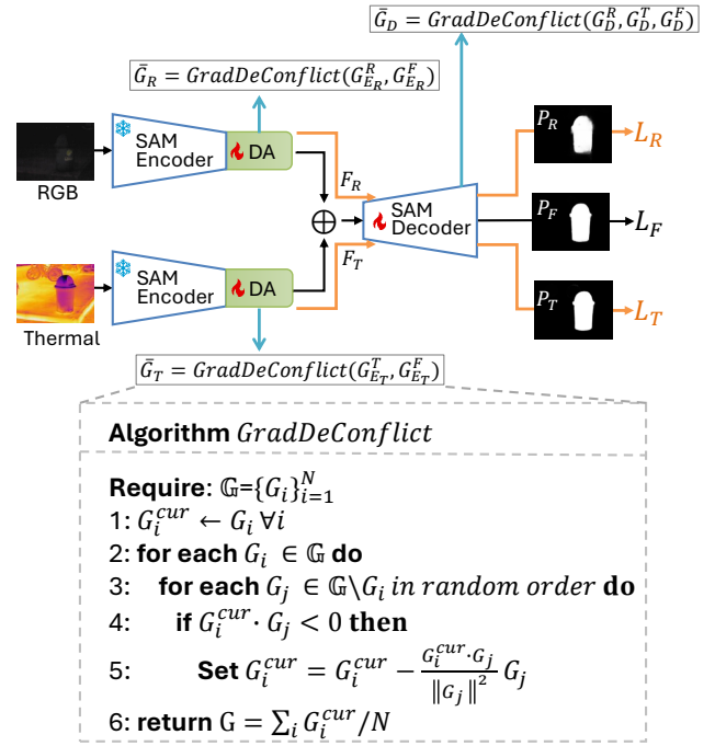
Fig. 2. The pipeline of the proposed SAMSOD .
