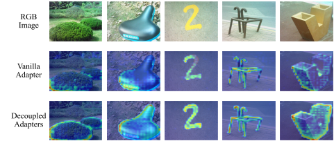
Fig. 10. The visual comparison between vanilla adapters (VA) and decoupled adapters (DA).
