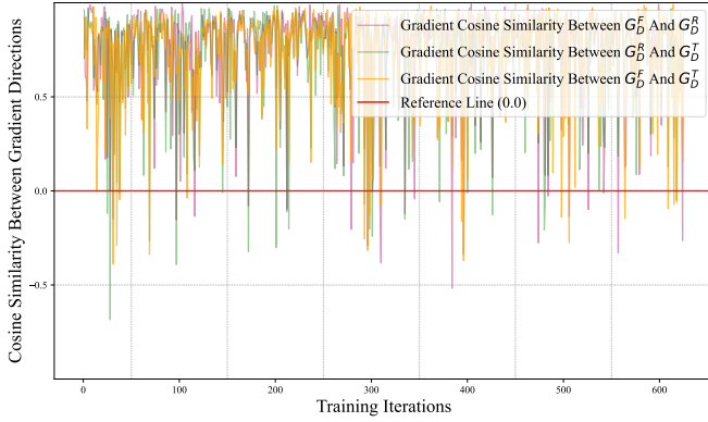
Fig. 4. The cosine similarity between gradients.
