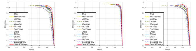
(a) VT821 dataset (b) VT1000 dataset (c) VT5000 dataset Fig. 6. P-R curves comparison of different models on three RGB-T datasets.
