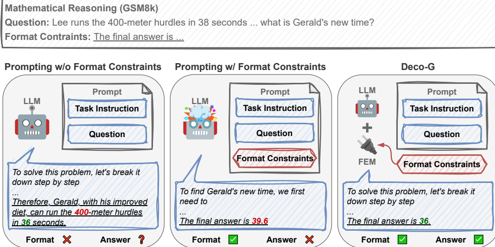
Figure 1: Example of GSM8k responses. LLM prompted without format constraints gets the correct answer, but the number is embedded in a sentence with mixed types, making it hard to capture. LLM prompted with format constraints gets the answer wrong. DECO-G prompts the model with task information and handles the format constraints by employing a Format Estimation Module (FEM). The framework generates the correct answer in the required format, making it easy to harvest.
