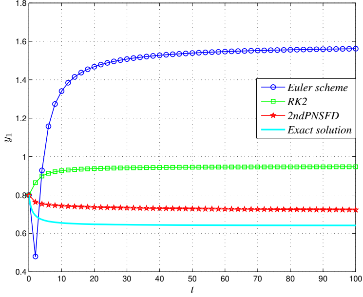
Figure 2: Approximate solutions for the y_1 -components generated by the second-order NSFD scheme and two standard numerical schemes.
