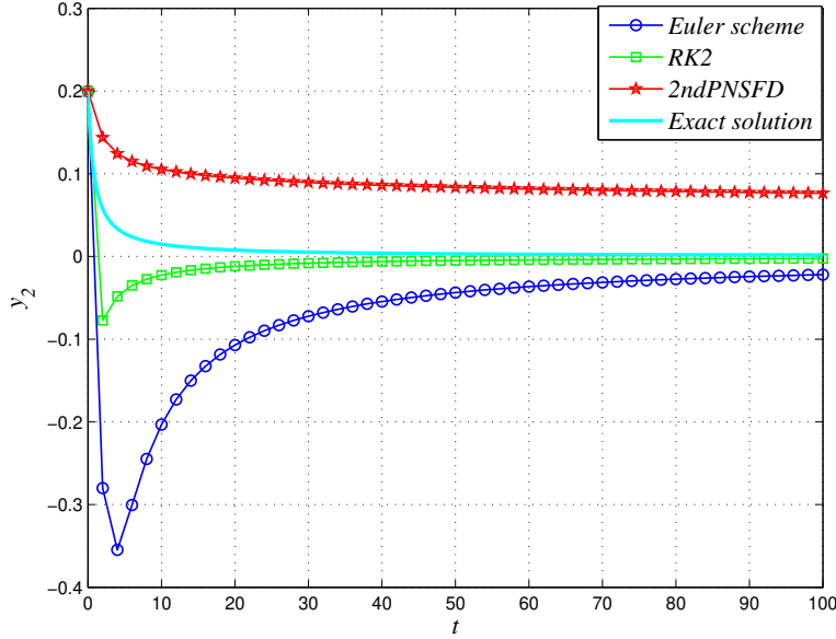
Figure 3: Approximate solutions for the y_2 -components generated by the second-order NSFD scheme and two standard numerical schemes.
