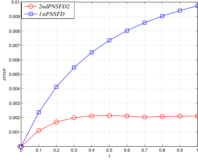
Figure 1: Errors obtained from the second-order and first-order NSFD schemes with \Delta t = 0.01 .
