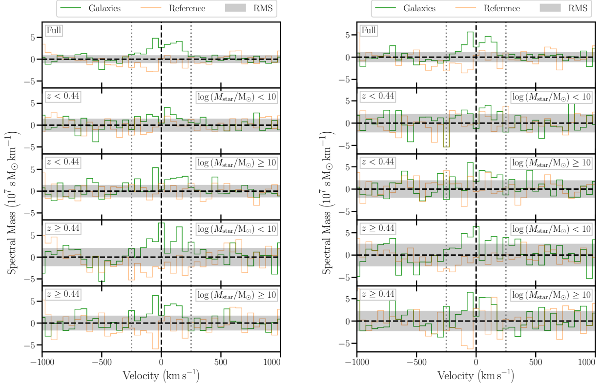
Figure 2. Weighted mean ( left ) and weighted median ( right ) spectra of the H I 21 cm emission line extracted using a physical aperture of 300 kpc in diameter around CUBS-MALS galaxies at 0.24 < z < 0.63 . The stacked spectra of CUBS galaxies are shown in thick green, while the reference spectra are shown in thin orange (see § 3 for details). The gray band marks the RMS fluctuations in the error spectrum. The signal associated with the full sample is presented in the top panel, where the signals extracted for individual subsamples are presented in the bottom four rows. The dotted vertical lines mark the velocity window for extracting the total H I mass for each sample. The 21 cm line is confidently detected in all samples with high- z galaxies displaying the strongest signal strength in both low- and high-mass galaxies (bottom two panels). The mean stacks for 150 kpc- and 450 kpc-diameter apertures are shown in Appendix A.
