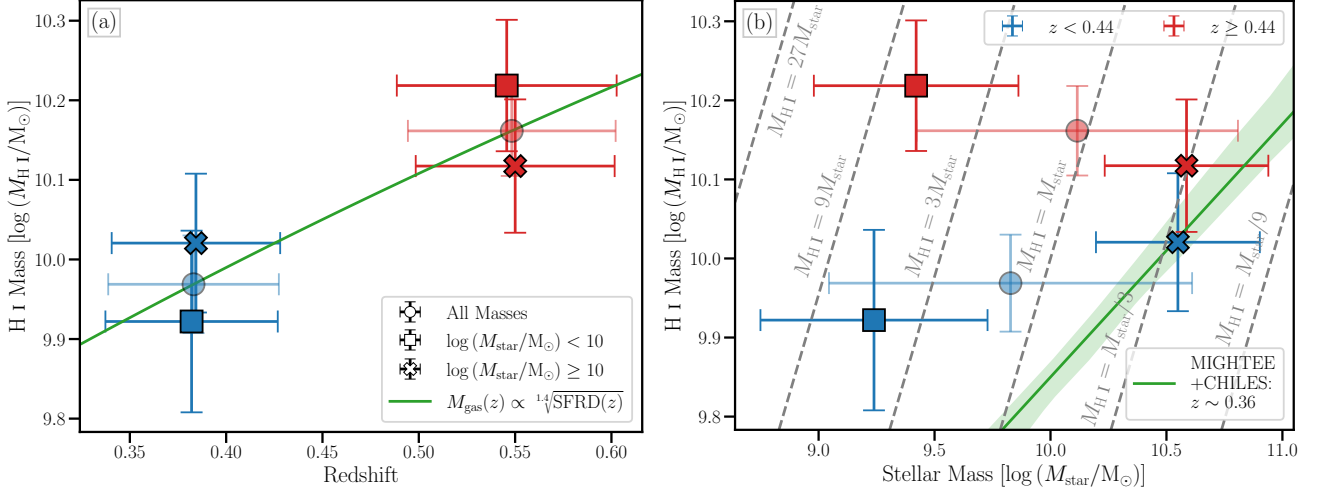
Figure 4. Variation of mean H I mass with redshift (panel a) and galaxy stellar mass (panel b). Data points and vertical error bars mark the weighted mean H I mass measurements and the associated uncertainties, color-coded according to redshift following what is presented in Figure 1. The horizontal bars indicate the dispersion of each subsample. For comparison, the solid green curve in panel (a) shows the anticipated redshift evolution of neutral gas content inferred from the cosmic star-formation rate density (P. Madau & M. Dickinson 2014, Equation 15), assuming a Kennicutt–Schmidt relation (R. C. Kennicutt 1998, see § 4.2 for details). The solid green line and the associated shaded band in panel (b) show the scaling relation and uncertainties from the combined MIGHTEE-H I+CHILES study by A. Bianchetti et al. (2025). The gray dashed lines mark fixed M_{\text{HI}}/M_{\text{star}} ratios to facilitate visual calibrations.
