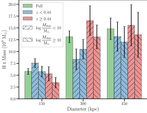
Figure 3. Cumulative mean H I mass with increasing aperture diameter. Doubling the extraction aperture diameter, from 150 kpc to 300 kpc, increases the extracted total H I 21-cm line flux by more than a factor of two, indicating a significant amount of neutral gas located beyond 75 kpc from the central galaxies, while further increasing the aperture diameter to 450 kpc results in a substantial increase in noise without a corresponding gain in signal (see also Figure A.1).
