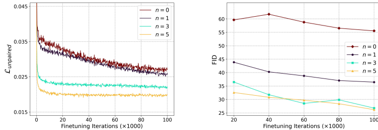
Figure 5: Learning curves of finetuned dDR on Face-UMDT-Latent w.r.t. different number of Tweedie refinement steps n \in \{0, 1, 3, 5\} . The task is Segment \rightarrow Sketch translation.
