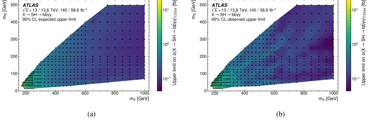
Figure 3: (a) Expected and (b) observed 95% CL upper limits on the X \rightarrow S(\rightarrow b\bar{b})H(\rightarrow \gamma\gamma) cross-section at 13 TeV, in the full (m_X, m_S) plane, including both the 1 b -tagged and 2 b -tagged categories.
