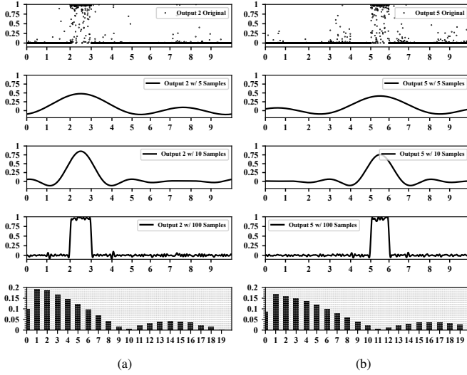
Fig. 1: Row 1: outputs 2 and 5 of a DNN classifier trained on MNIST dataset in columns (a) and (b), respectively. Rows 2-4: Fourier approximation of the two functions using 5, 10, and 100 terms, respectively. Last row: bar charts for the first 20 frequency buckets of the FFT for the two functions. The bar charts are annotated with gray guidelines to aid visual comparison of the heights of the bars between two diagrams.
