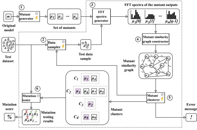
Fig. 2: A DNN mutation analysis workflow involving DM#. Sharp-edged rectangles denote processes; rounded ones denote data/artifacts. Arrows denote control flow. Gear and lightning bolt icons are used to annotate user-configurable and non-deterministic processes, resp. Processes and artifacts inside the area marked by dashed line are part of DM#.
