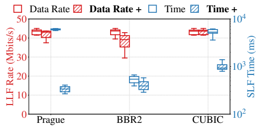
Fig. 11 — L4Span improves the finish time of the SLF (14 kilo-bytes) while keeping the LLF throughput usage (center: median, box edges: 25th- and 75th-percentile, whiskers: 10th- and 90th-percentile).
