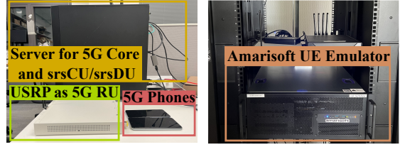
Fig. 8— Hardware used in L4Span implementation. One desktop server runs the 5G Core, srsCU and srsDU, and the USRP is served as the RU. We use both real phones and Amarisoft UE emulator as the UEs for the evaluation.
