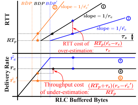
Fig. 6— Cost of errors. L4Span marks the packet using the estimated egress rate and a queuing delay threshold \tau_s . Stars ( \star ) mark the ideal operation points with the estimated egress rate.
